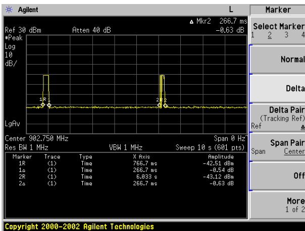
Package Transfer Time Plot CH01-10-11s
