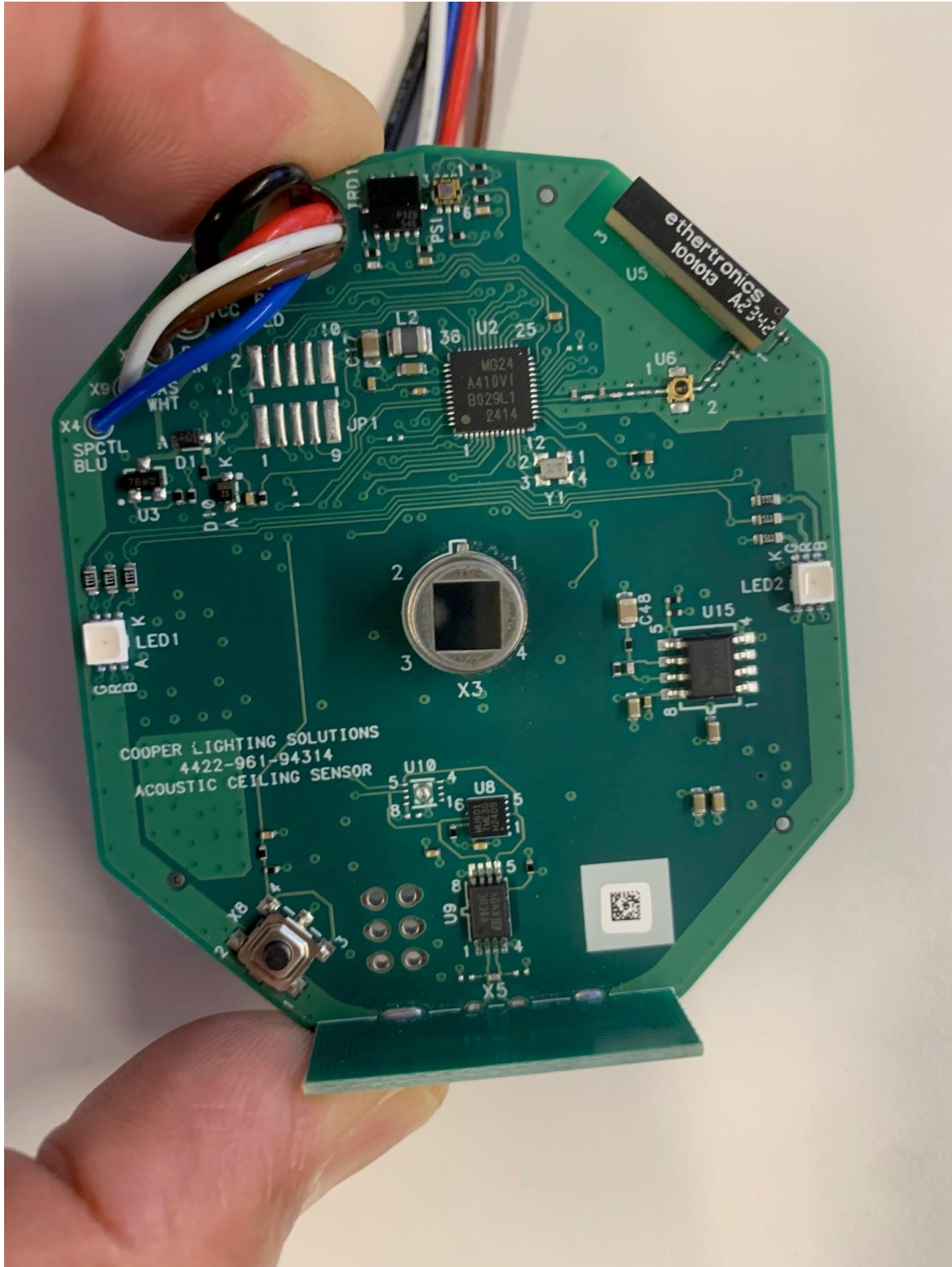
Figure 3: Low Voltage Top View
