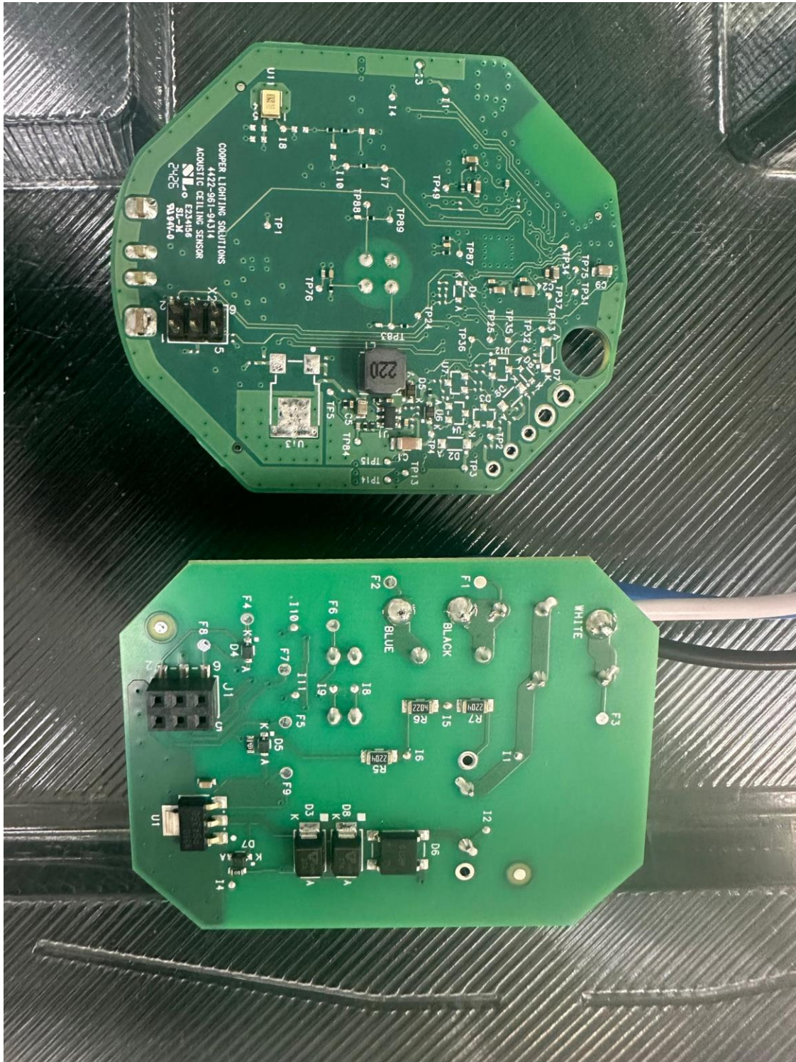
Figure 2: Line Voltage Bottom View
