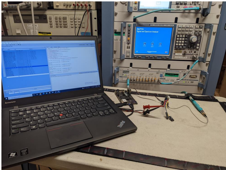
Figure 8: Test Setup – Antenna Port Measurement
