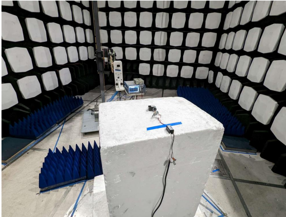
Figure 5: Test Setup – Radiated Emissions >18GHz
