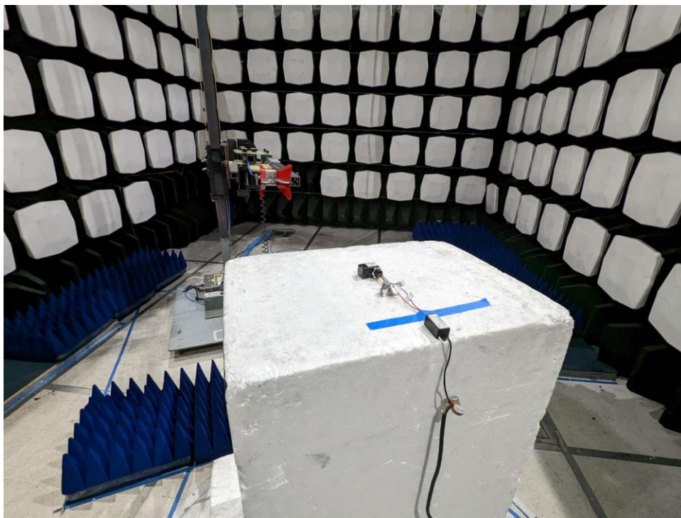
Figure 4: Test Setup – Radiated Emissions >10GHz
