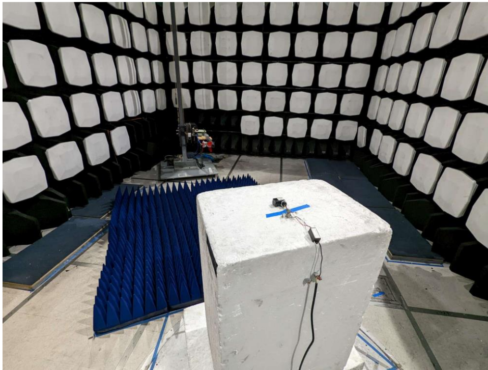
Figure 3: Test Setup – Radiated Emissions >1GHz
