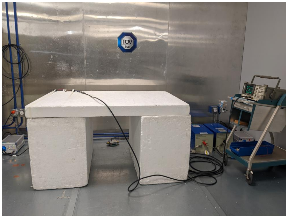
Figure 6: Test Setup – Conducted Emissions
