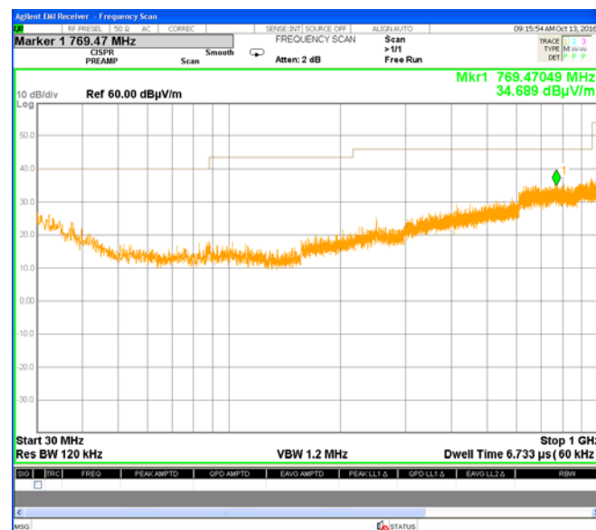
Plot # 33. Investigation result in 30 - 1000 MHz frequency range.
