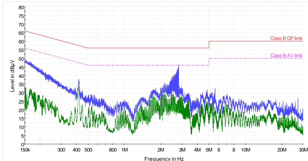
Plot # 35. AC line conducted emissions test. Line Neutral.
