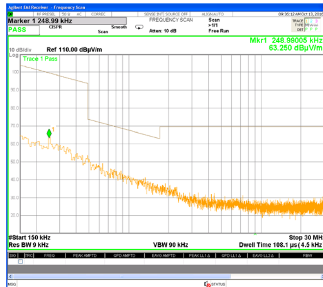
Plot # 32. Investigation result in 0.15 – 30 MHz frequency range.
