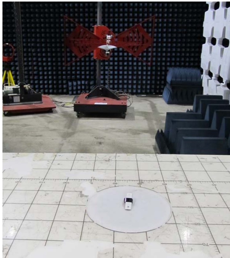
Photo 2. Radiated emissions test setup with Biconilog antenna.
