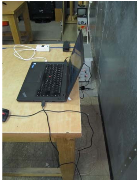
Photo 6. Conducted emissions test setup.
