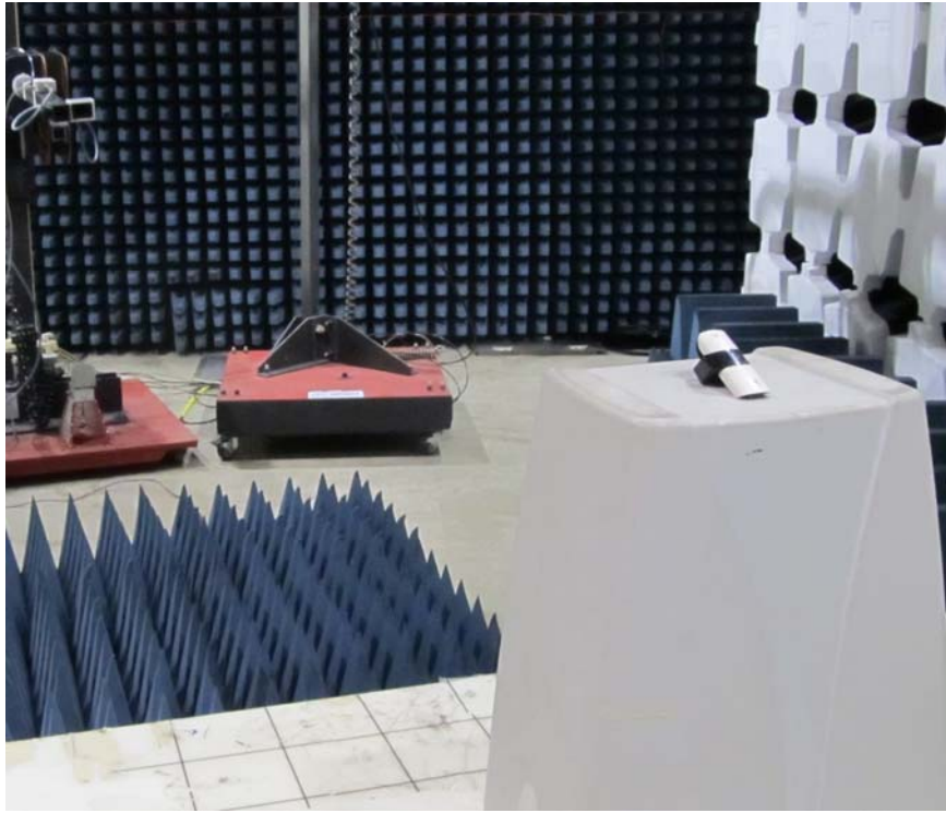
Photo 5. Radiated emissions test setup.
