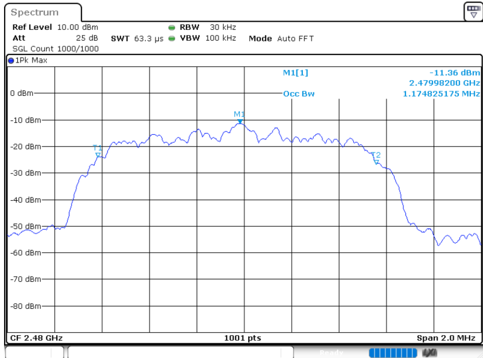
-20 dB BW NVNT 2-DH5 2480MHz Ant1
