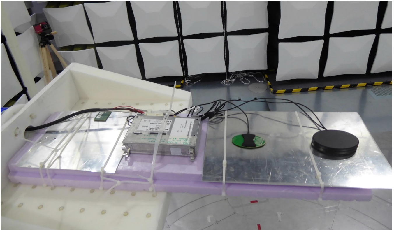
Test setup on positioner
