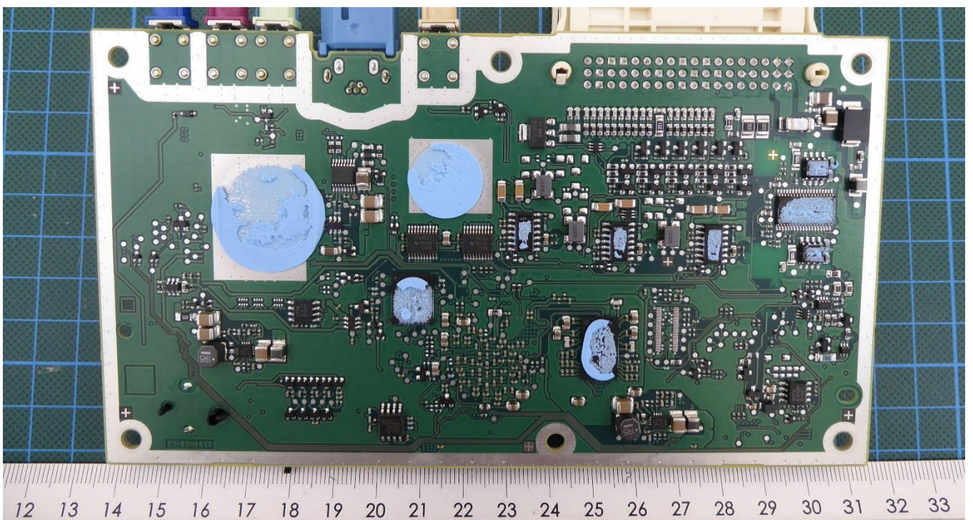
PCB bottom view
