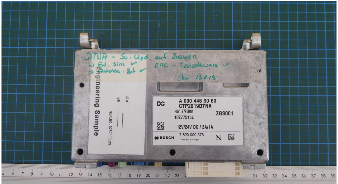
EUT, top view
