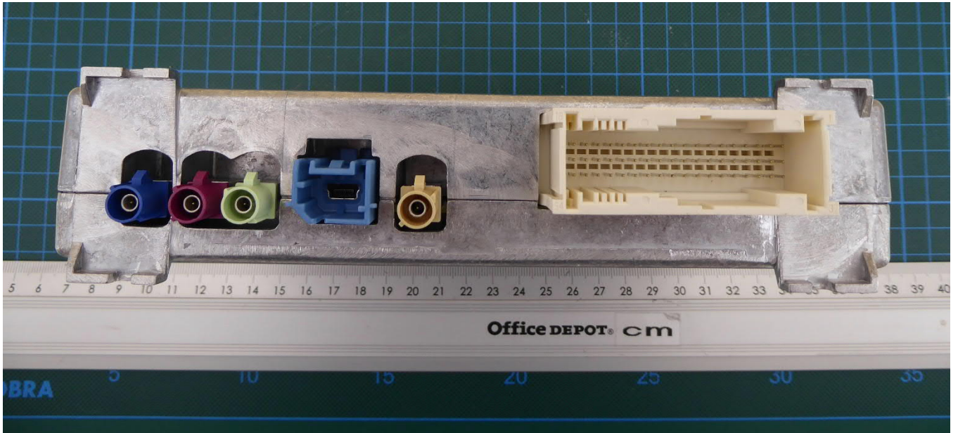
Connectors rear view
