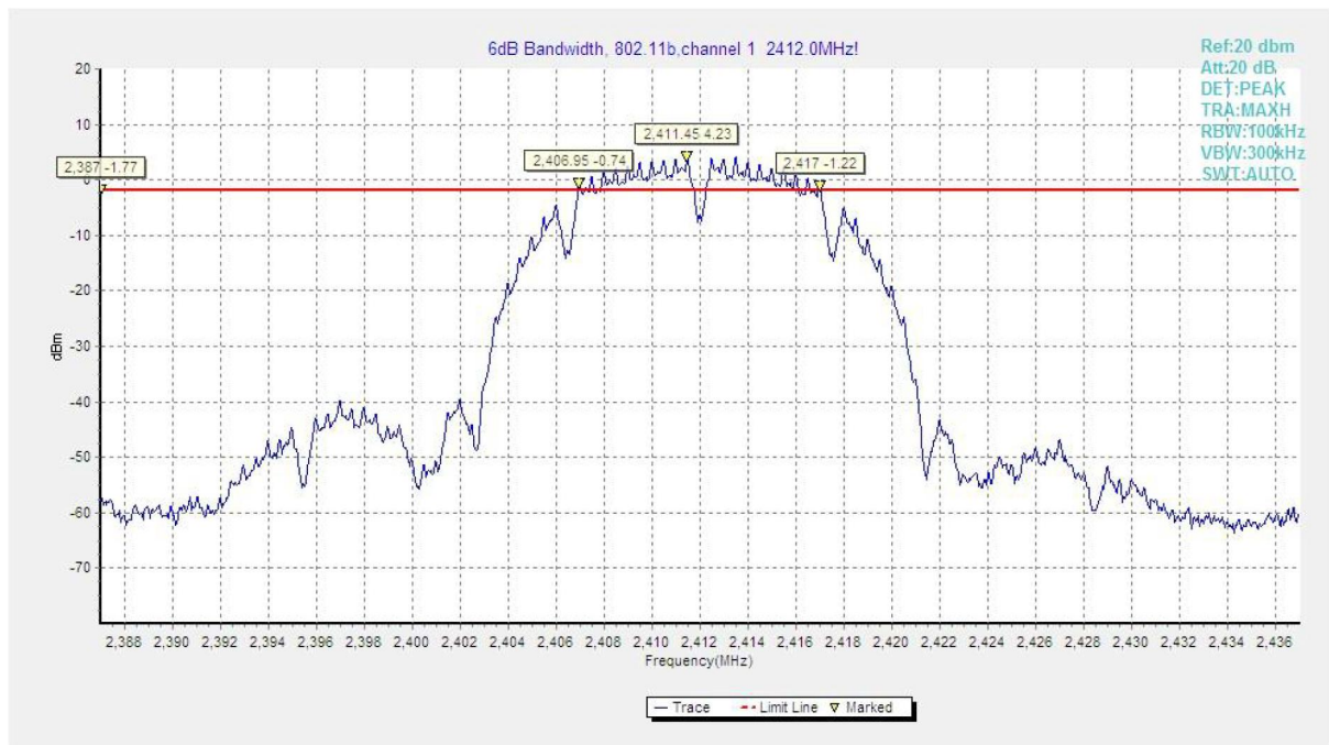
Fig.10 6dB Bandwidth (802.11b, CH 1)
