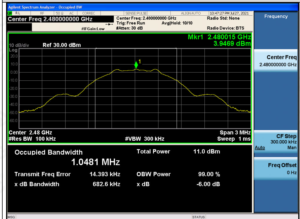
Test_Graph_LE1M_ANT1_2480_1Mbps_DTSBW
