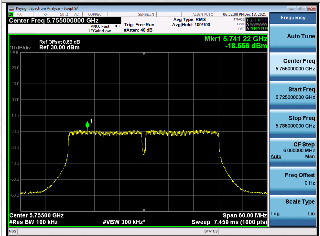
Test_Graph_802.11ac40_ANT2_5755_MCS9_PSD
