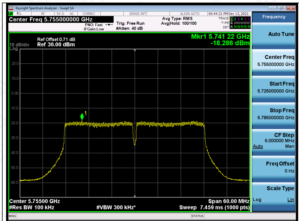
Test_Graph_802.11n40_ANT2_5755_MCS0_PSD
