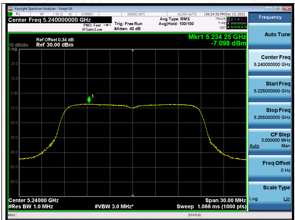
Test_Graph_802.11ac20_ANT2_5240_MCS9_PSD
