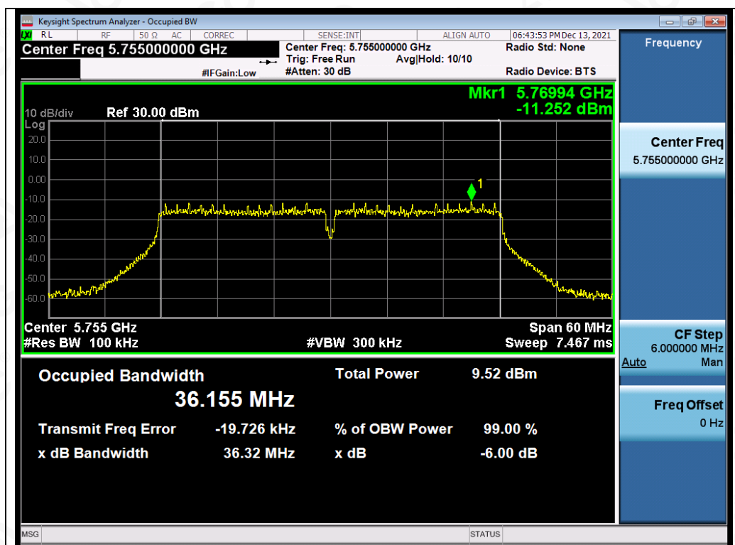
Test_Graph_802.11n40_ANT2_5755_MCS0_DTSBW
