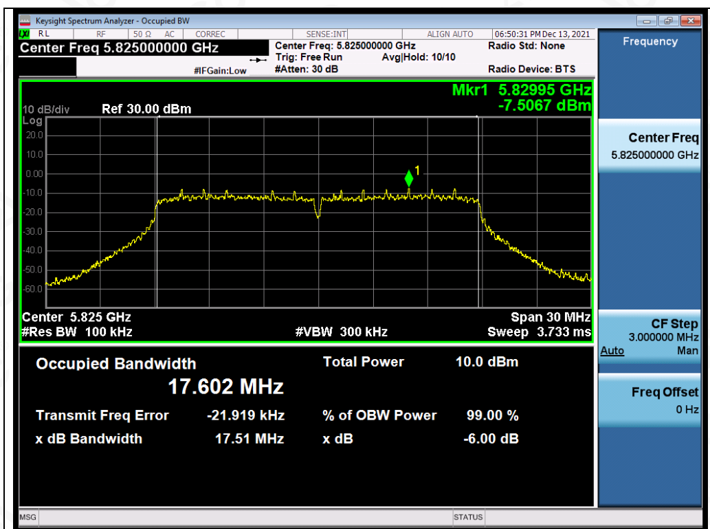
Test_Graph_802.11ac20_ANT2_5825_MCS9_DTSBW
