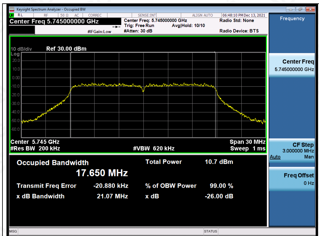
Test_Graph_802.11ac20_ANT2_5745_MCS0_OBW
