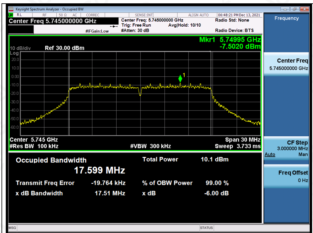
Test_Graph_802.11ac20_ANT2_5745_MCS0_DTSBW
