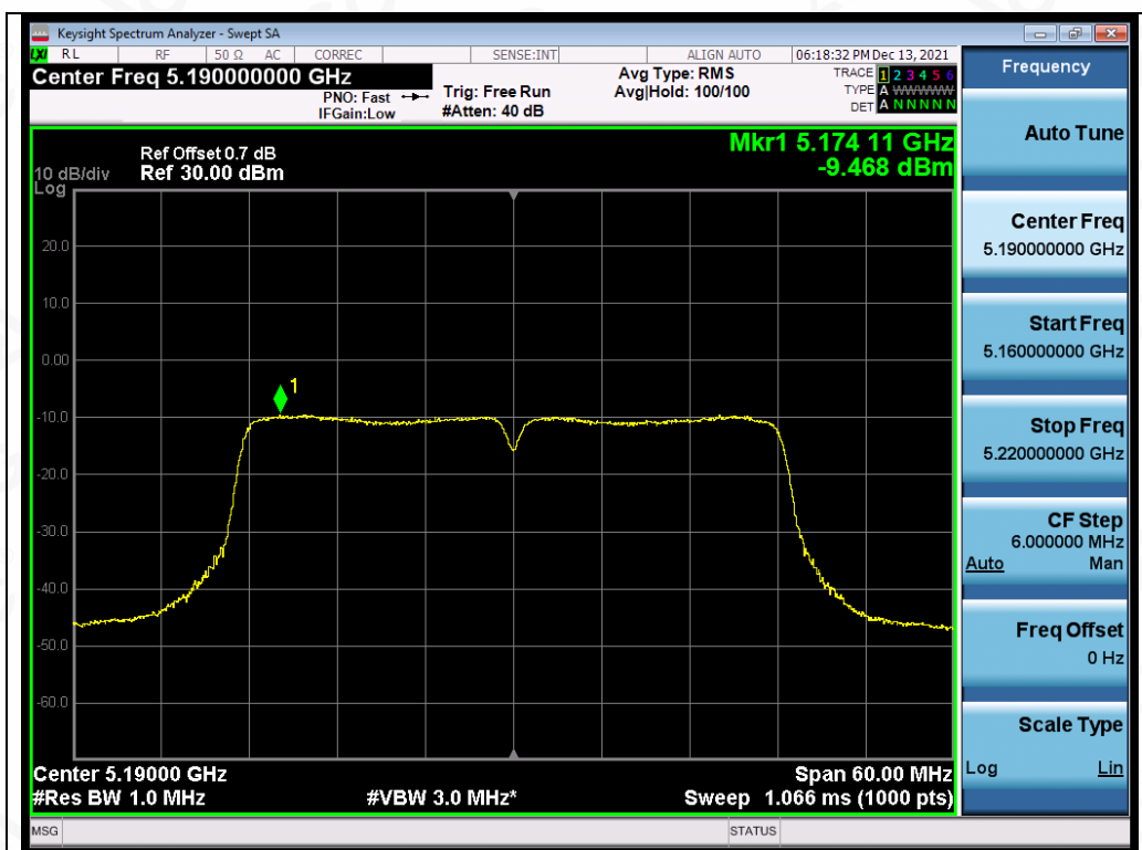
Test_Graph_802.11n40_ANT2_5190_MCS0_PSD
