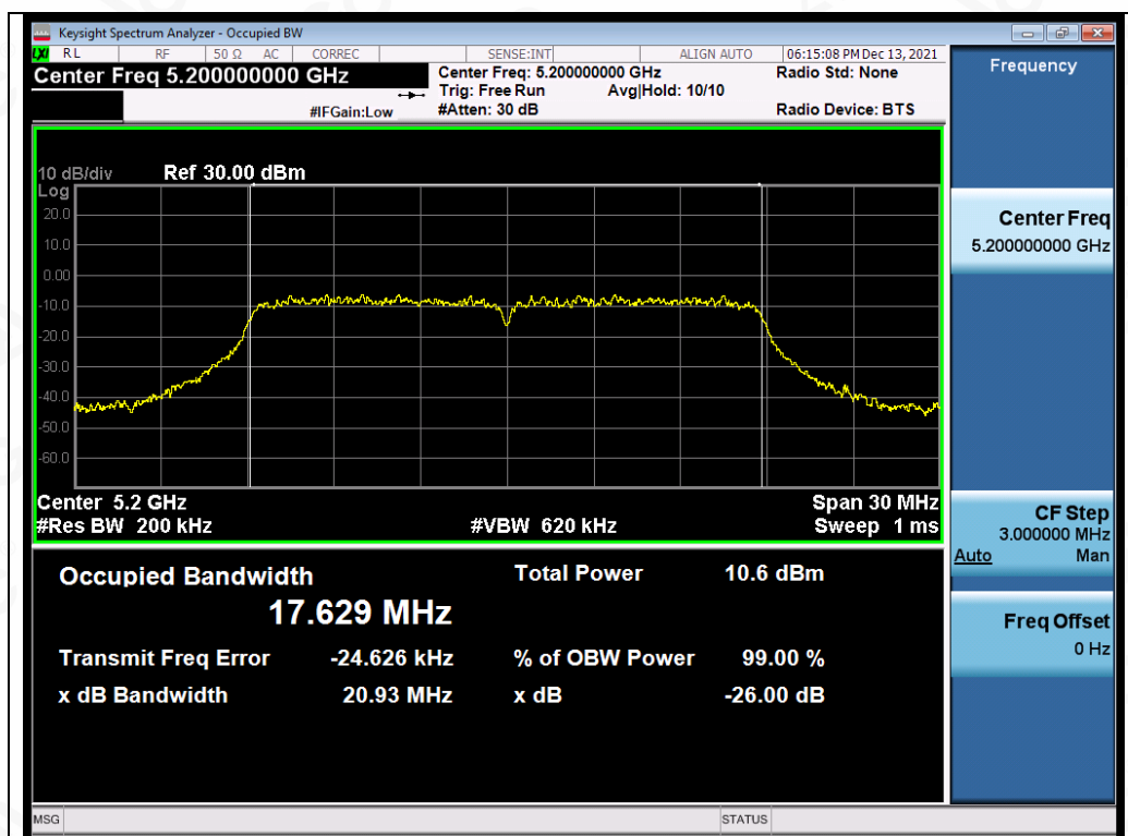
Test_Graph_802.11n20_ANT2_5200_MCS0_OBW
