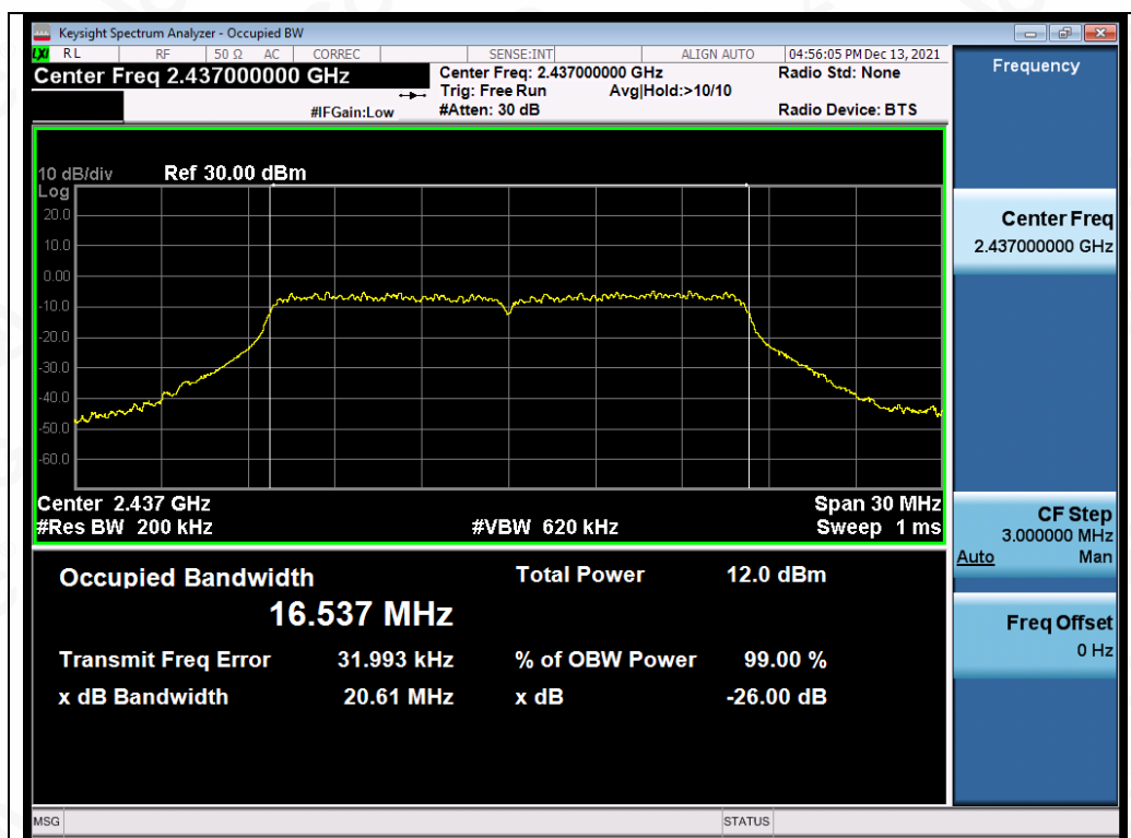
Test_Graph_802.11g_ANT2_2437_6Mbps_OBW
