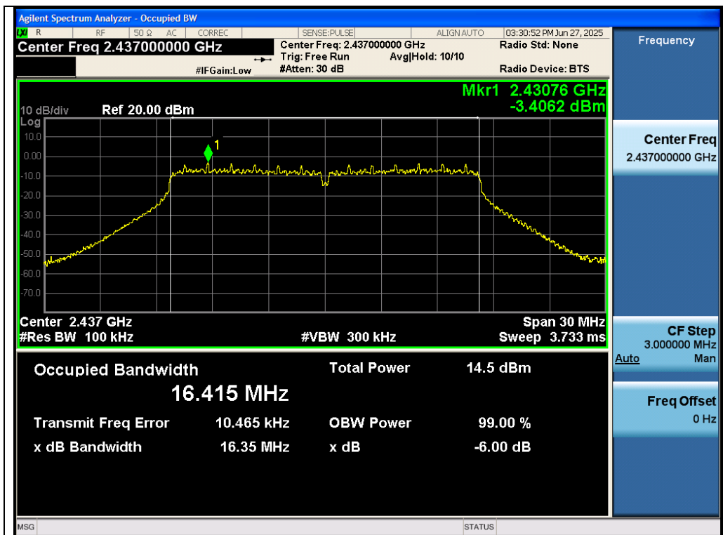
Test_Graph_802.11g_ANT1_2437_6Mbps_DTSSW
