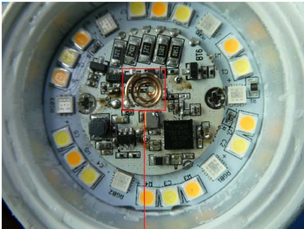
RF Antenna
