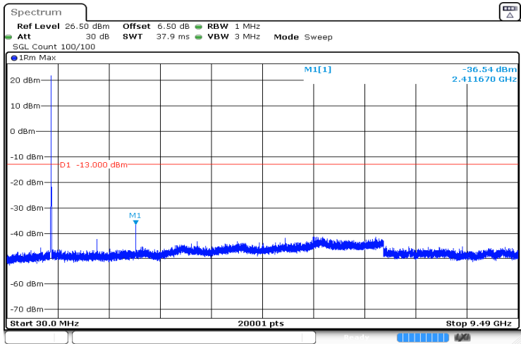
5MHz_High_QPSK_25@0 -36.54 dBm
