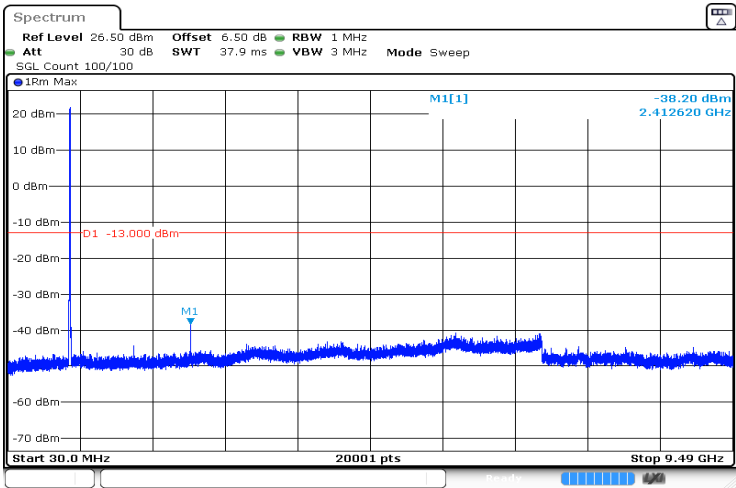
5MHz_Mid_QPSK_25@0 -38.20 dBm
