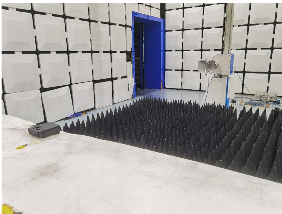
Description: Radiated Emission Test Setup for 1GHz ~ 18GHz (Mode1)
