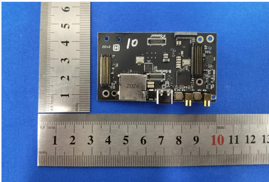
Photo 2: Internal View for PCB A
