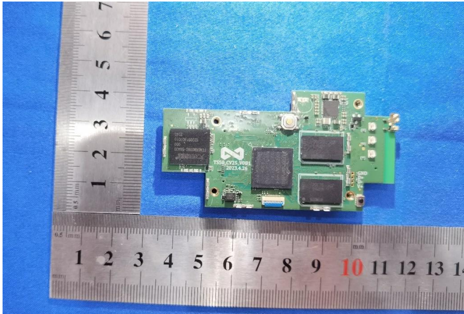
Photo 9: Internal View for PCB B
