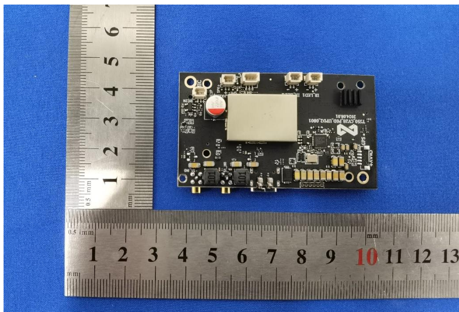
Photo 3: Internal View for PCB A
