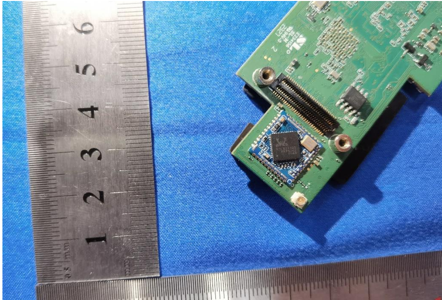
Photo 11: Internal View for WIFI/BT Chip
