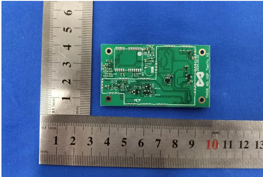
Photo 7: Internal View for PCB C
