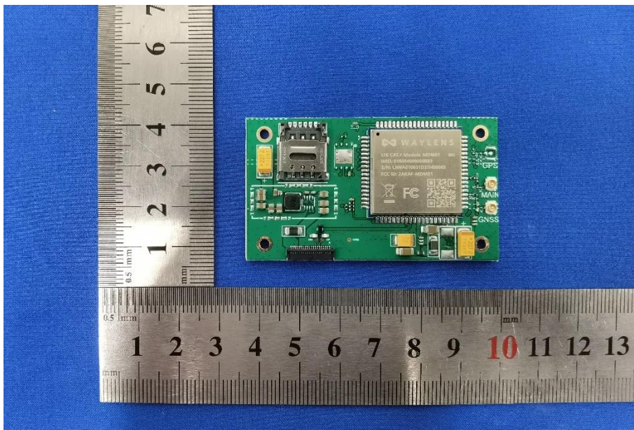
Photo 6: Internal View for PCB C
