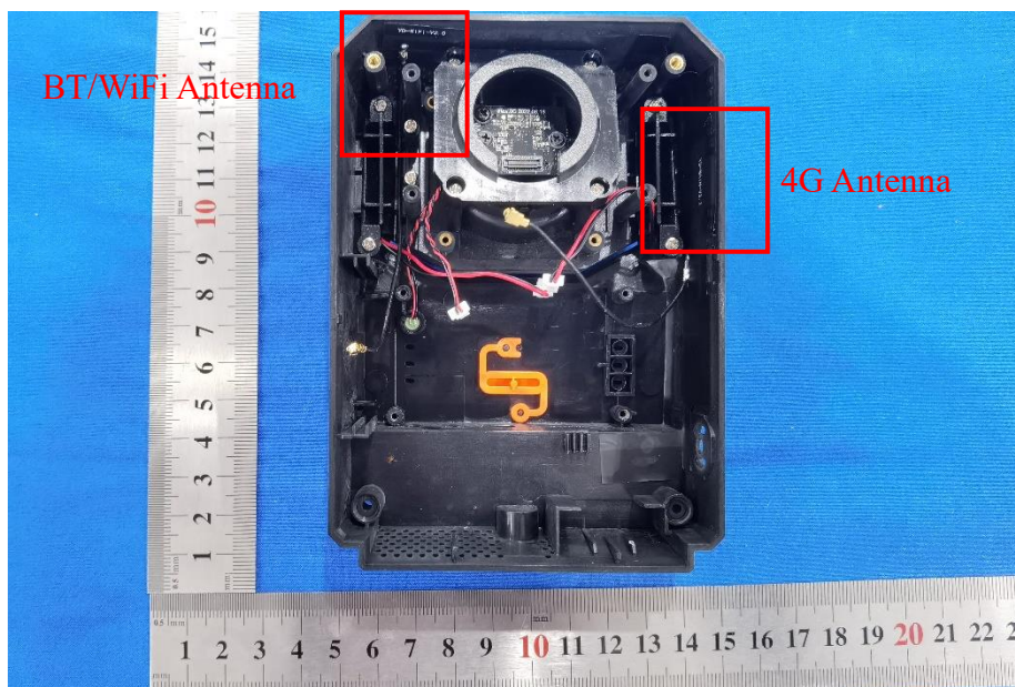
Photo 12: Antenna
