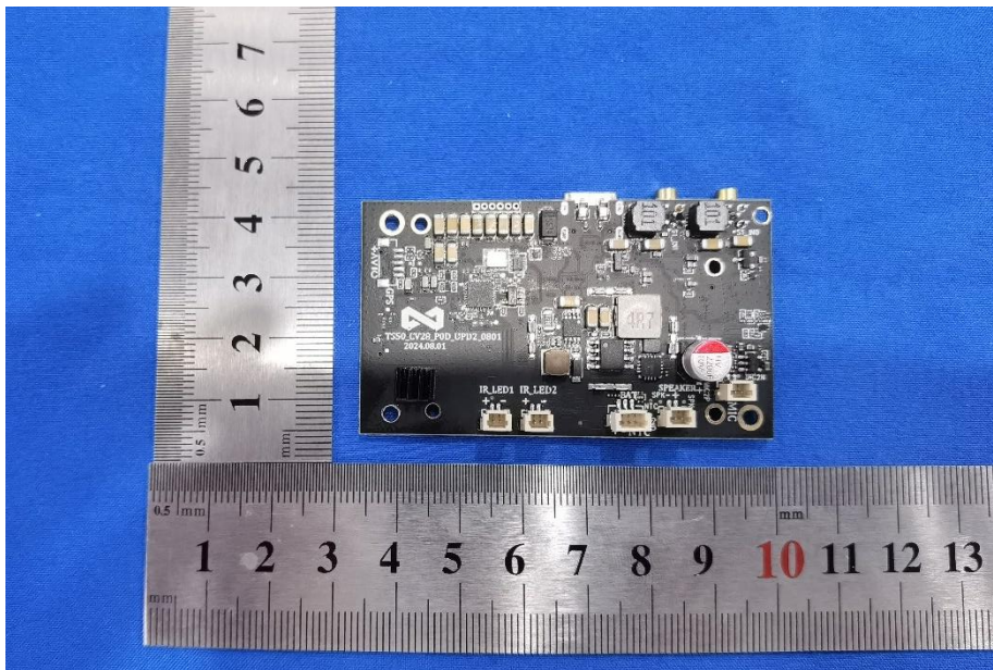
Photo 8: Internal View for PCB A
