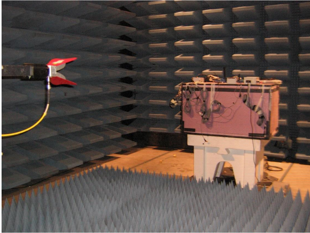
Figure 3: Radiated Emissions (above 1GHz) Test Setup
