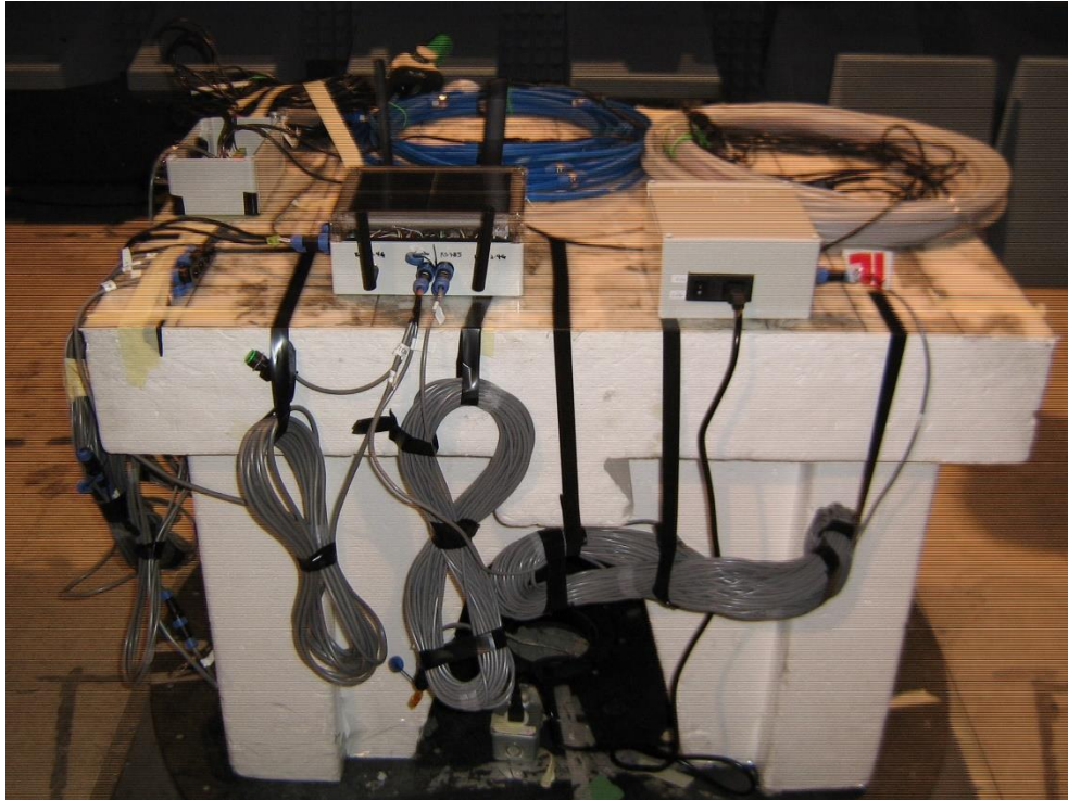
Figure 3: Radiated Emissions (below 1GHz close-up view) Test Setup
