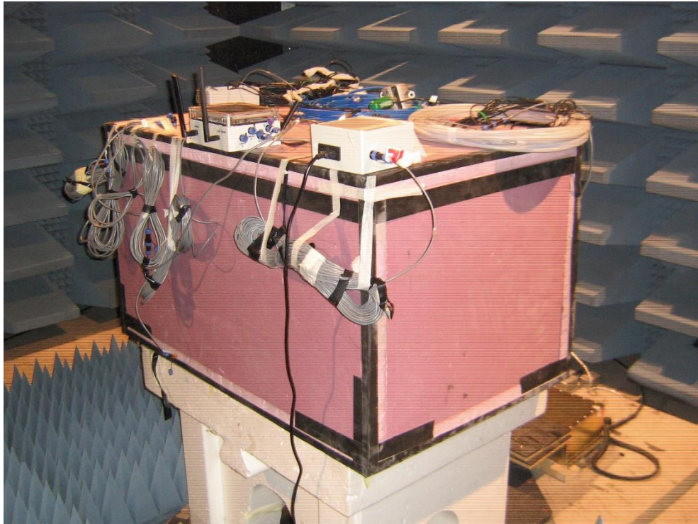
Figure 5: Radiated Emissions (above 1GHz close-up view) Test Setup
