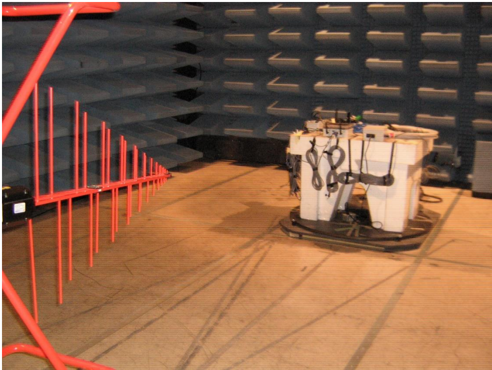
Figure 2: Radiated Emissions (30MHz - 1GHz) Test Setup
