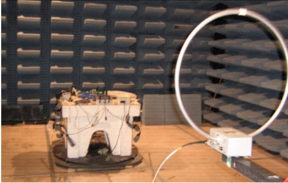
Figure 1: Radiated Emissions (30MHz - 1GHz) Test Setup
