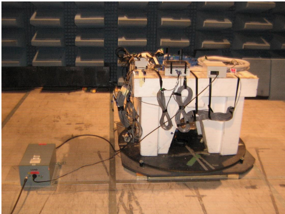
Figure 6: Conducted Emissions Test Setup
