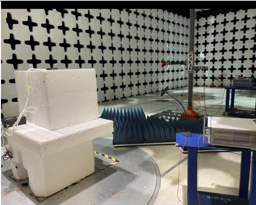
Radiated Emission Test above 1GHz Rear View
