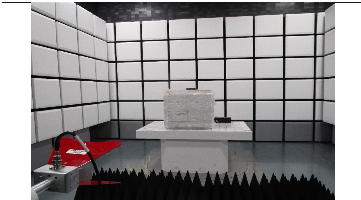
Radiated Emission Test above 1GHz Front View
