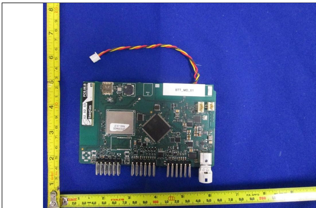
EUT Antenna Top View
