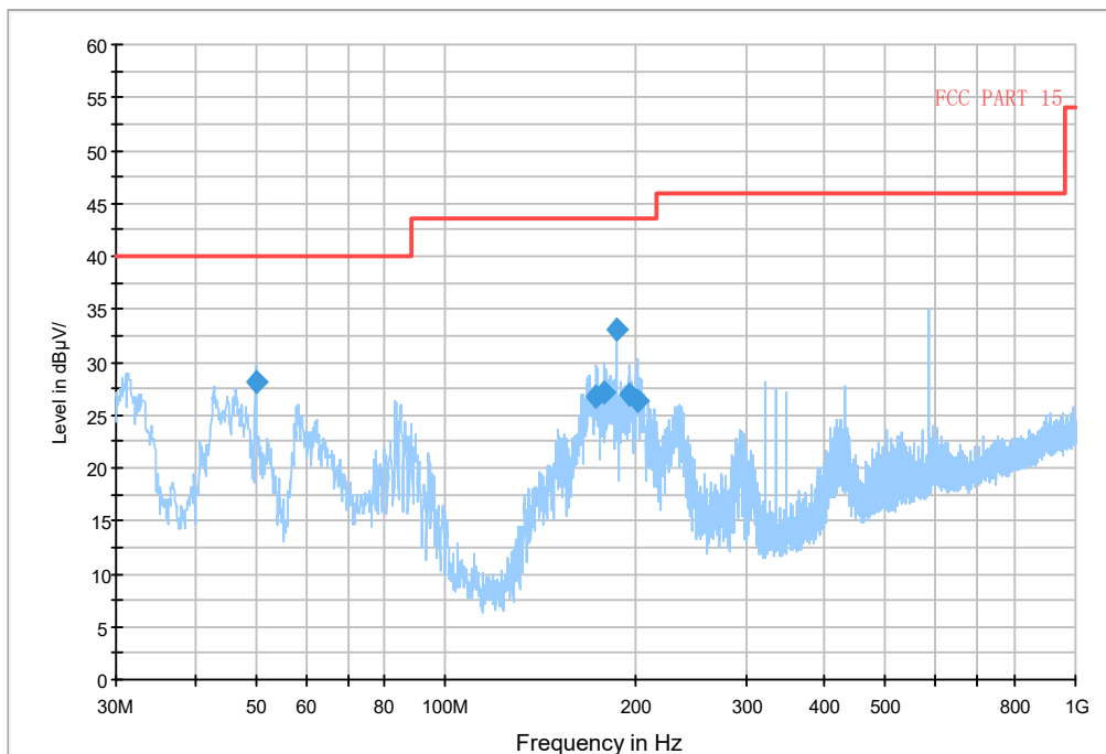
Fig.18 Radiated emission: Ch0, 30MHz-1GHz
