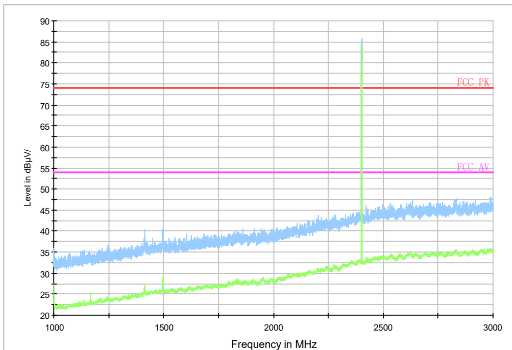
Fig.19 Radiated emission: Ch0, 1GHz-3GHz
