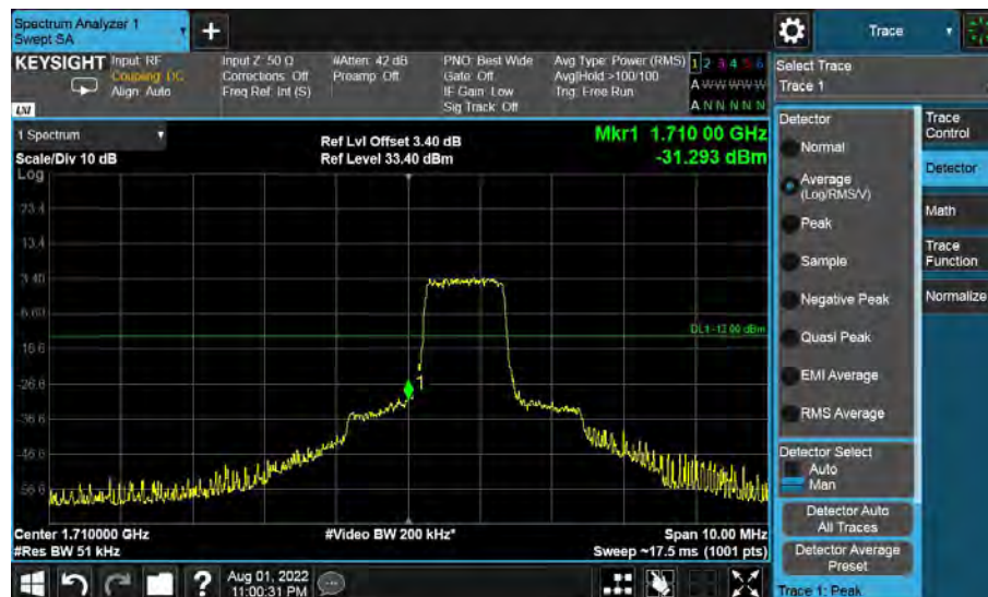
Band4-Low Channel-5MHz Bandwidth-6RB-QPSK
