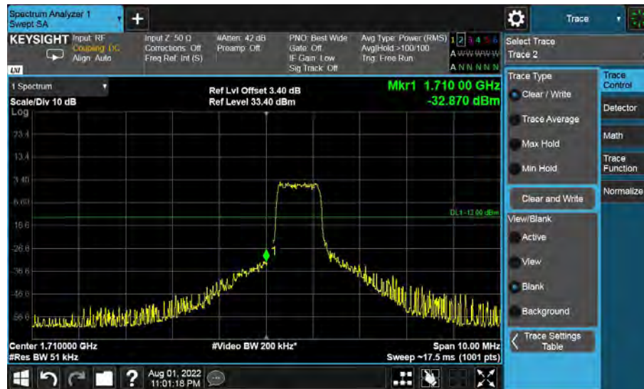
Band4-Low Channel-5MHz Bandwidth-6RB-16QAM
