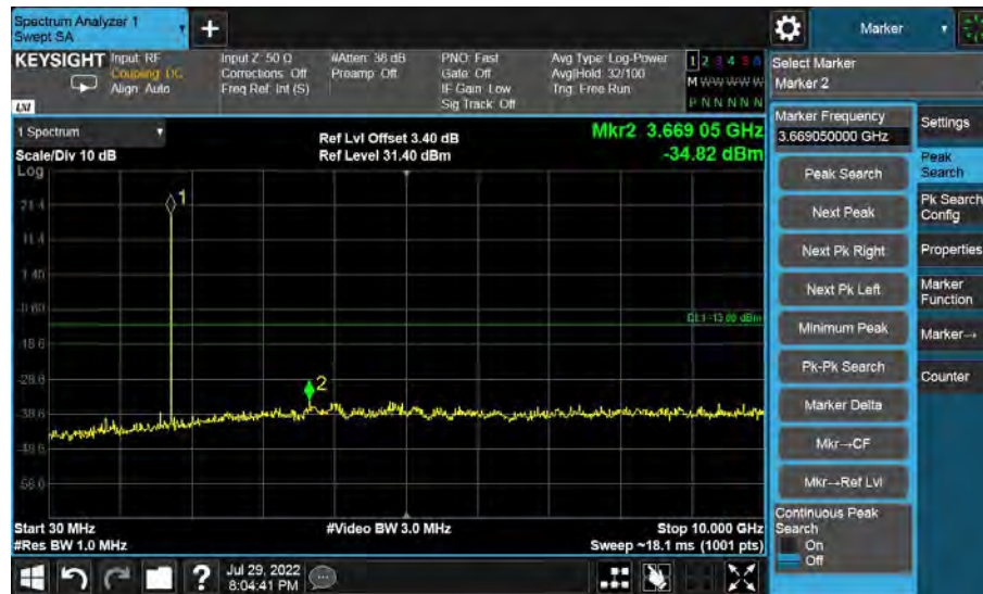
30MHz to 10GHz, Mid Channel, Subcarrier (15kHz), QPSK, 12@0
