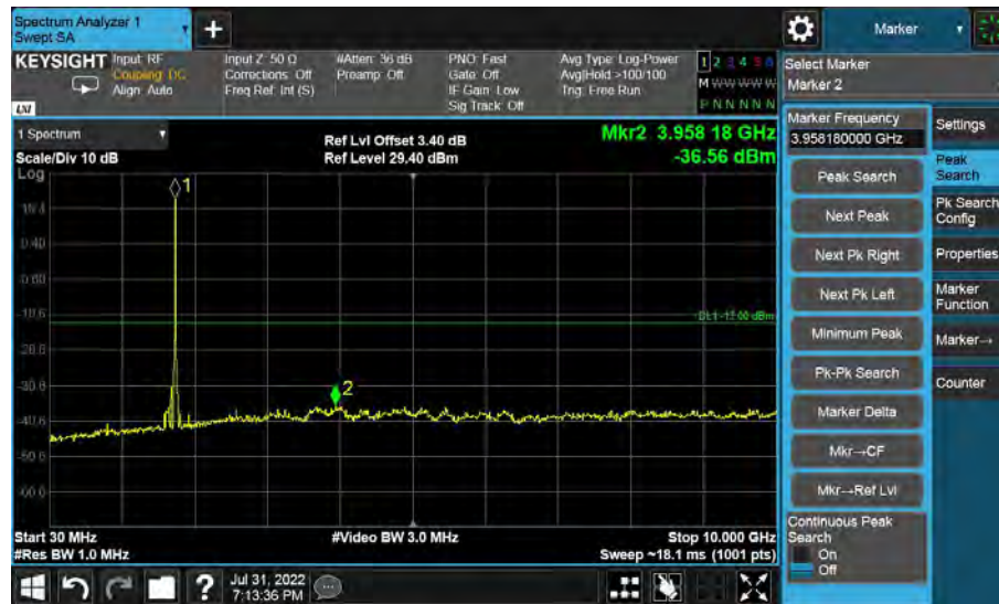
30MHz to 10GHz, High Channel, Subcarrier (3.75kHz), BPSK, 1@0
