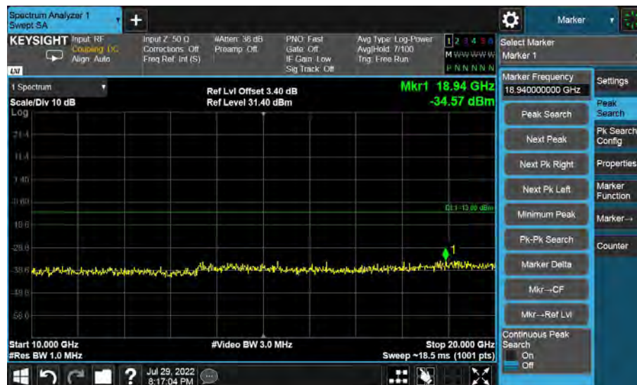
10GHz to 20GHz, High Channel, Subcarrier (15kHz), QPSK, 1@0
