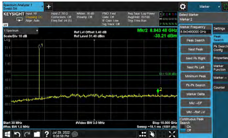
30MHz to 10GHz, Low Channel, Subcarrier (15kHz), BPSK, 1@0
