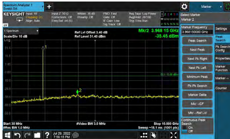
30MHz to 10GHz, High Channel, Subcarrier (15kHz), BPSK, 1@0
