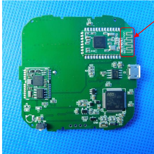
BT Antenna
