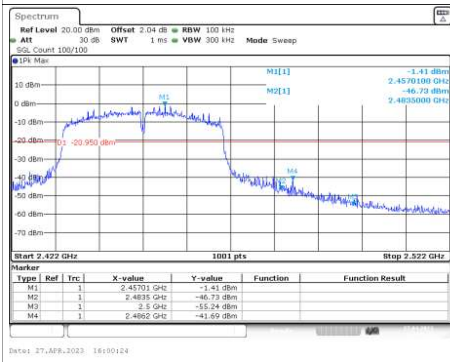
Band Edge NVNT n40 2452MHz Ant1 Emission
