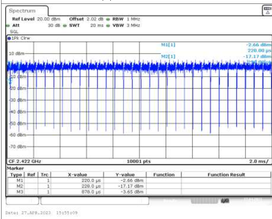
Duty Cycle NVNT n40 2422MHz Ant1
