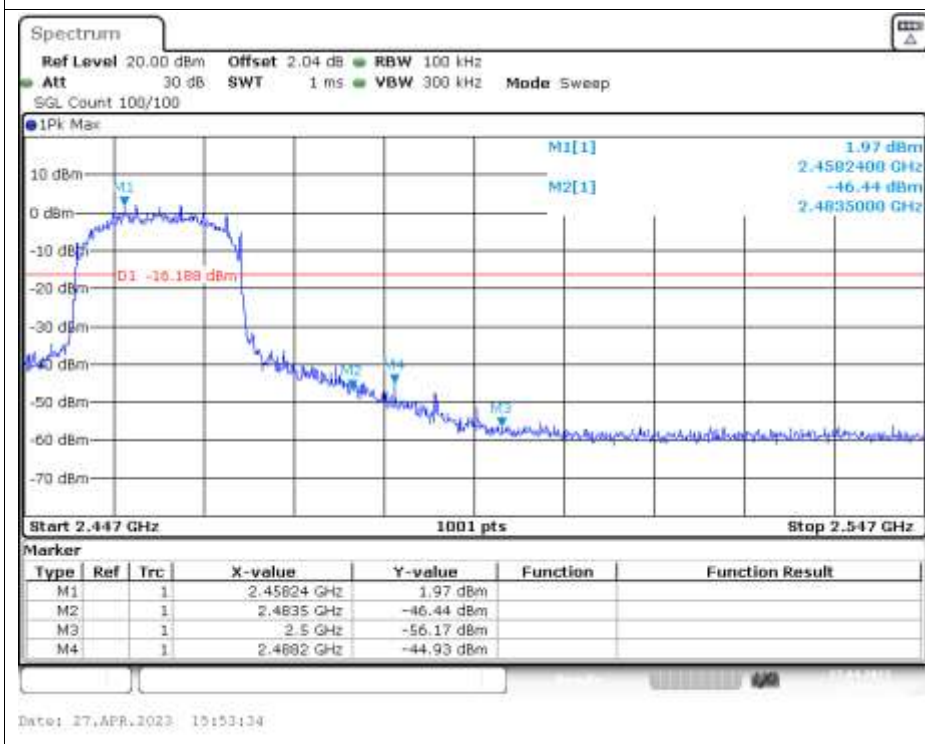
Band Edge NVNT n20 2462MHz Ant1 Emission
