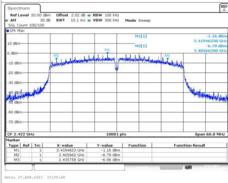
-6dB Bandwidth NVNT n40 2422MHz Ant1
