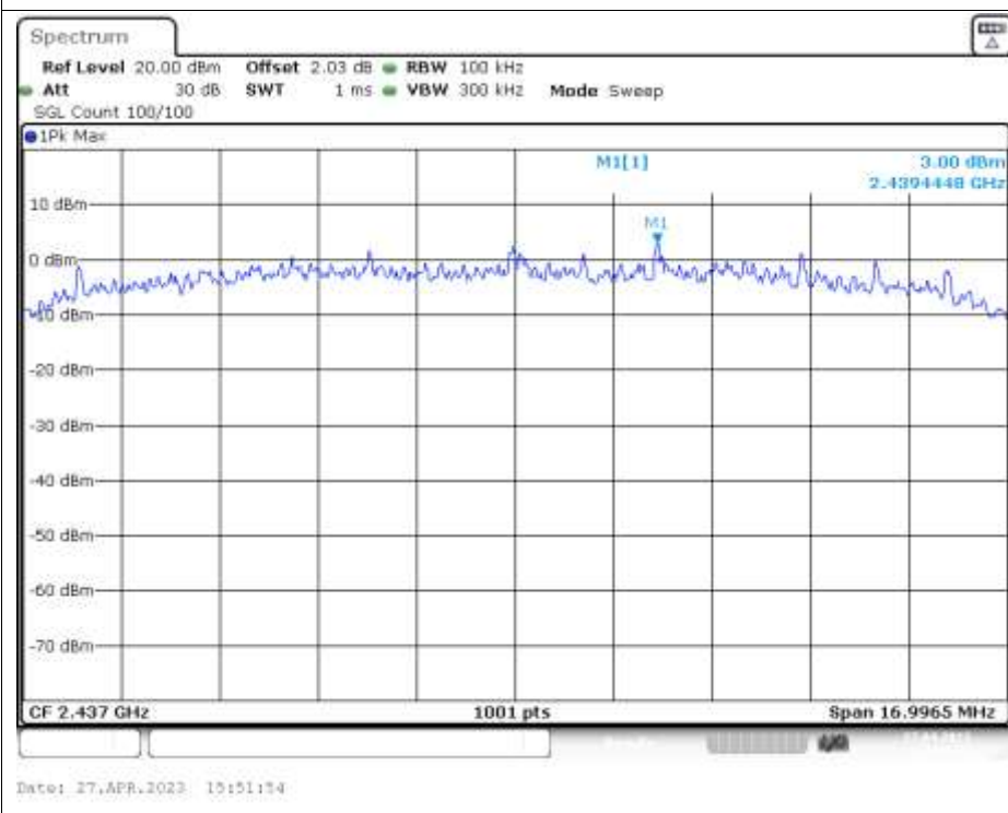
PSD NVNT n20 2437MHz Ant1
