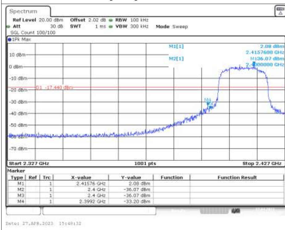
Band Edge NVNT g 2412MHz Ant1 Emission
