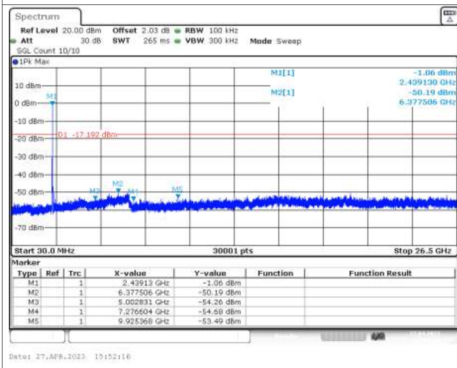
Tx. Spurious NVNT n20 2437MHz Ant1 Emission
