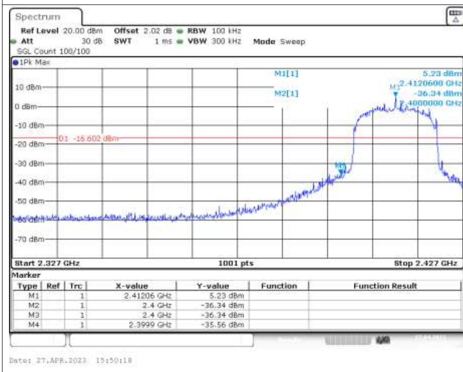
Band Edge NVNT n20 2412MHz Ant1 Emission
