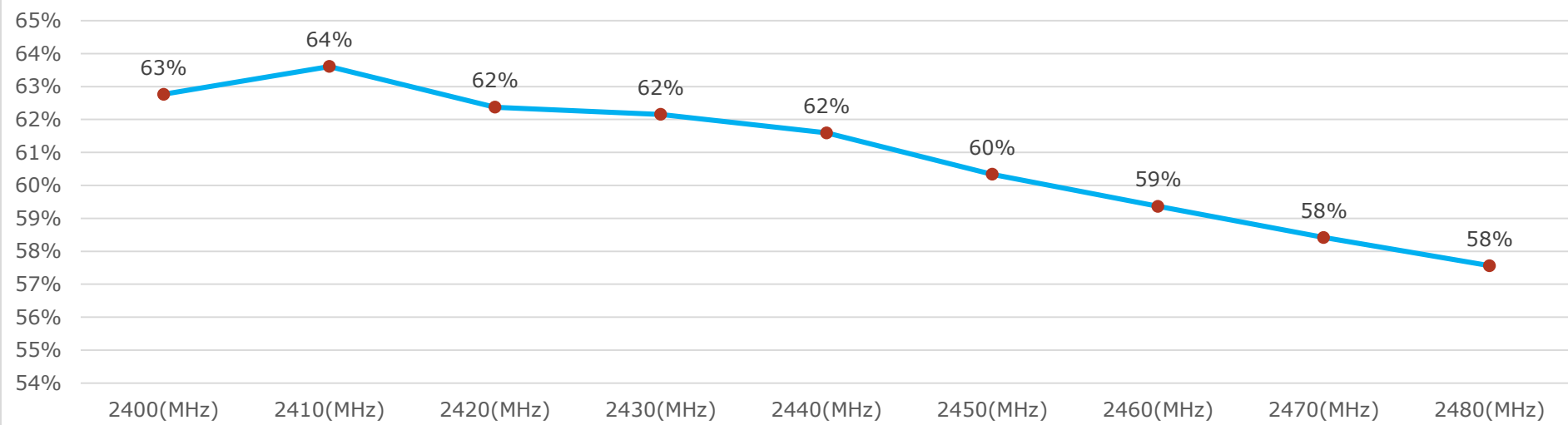
Efficiency of LVD05-WiFi
