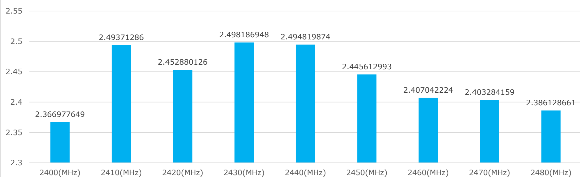
Gain of LVD05-WiFi
