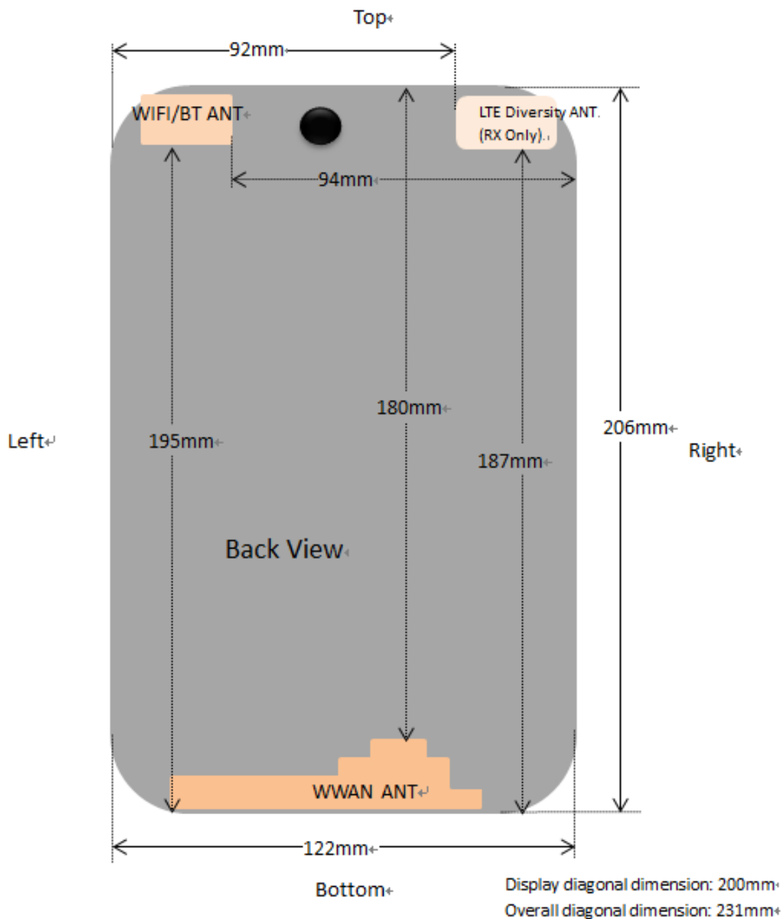
Fig.14.1 EUT Antenna Locations
