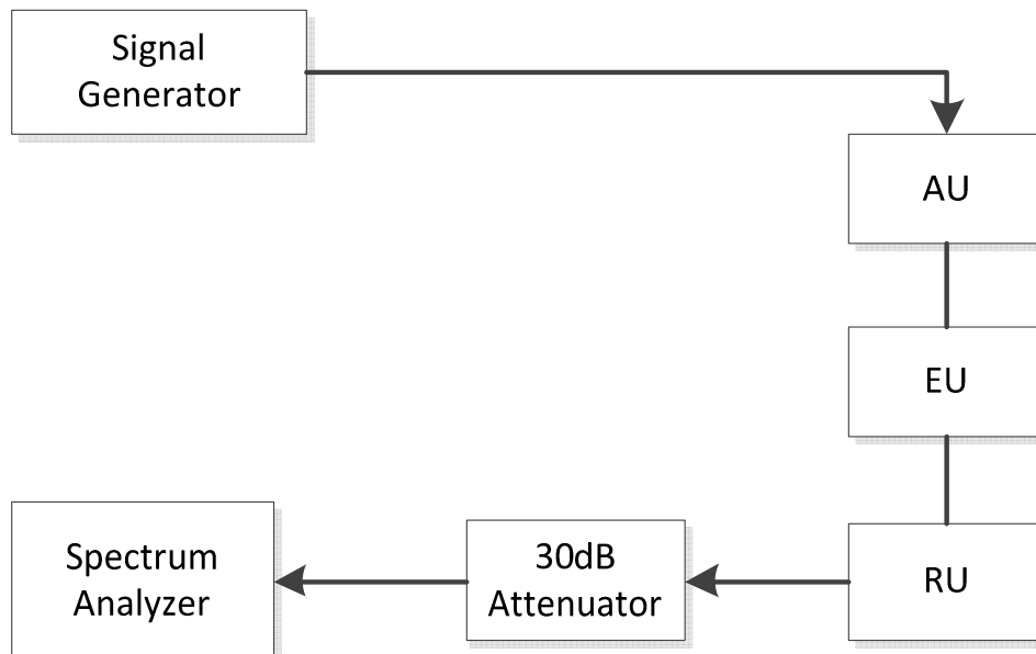
Fig.4. Out of Band rejection test configuration
