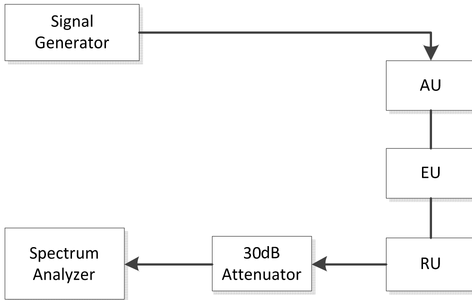
Fig.1 RF Output Power test configuration
