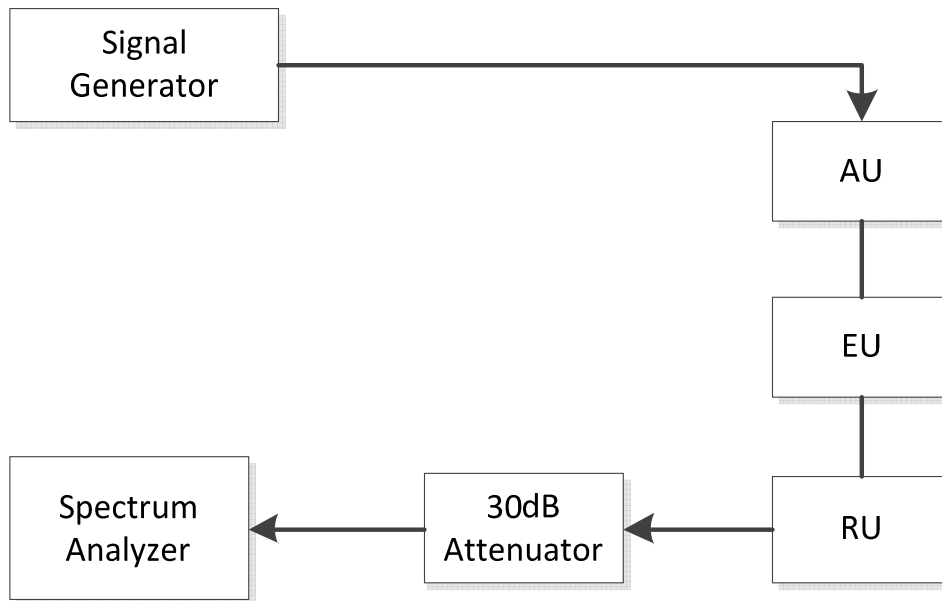
Fig.2. Conducted Spurious Emissions test configuration
