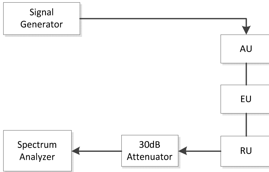
Fig.3. Band edge and Intermodulation test configuration
