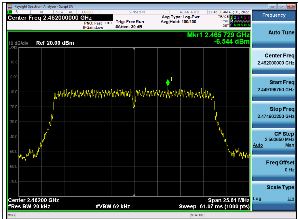
Test_Graph_802.11n20_ANT3_2462_MCS0_PSD
