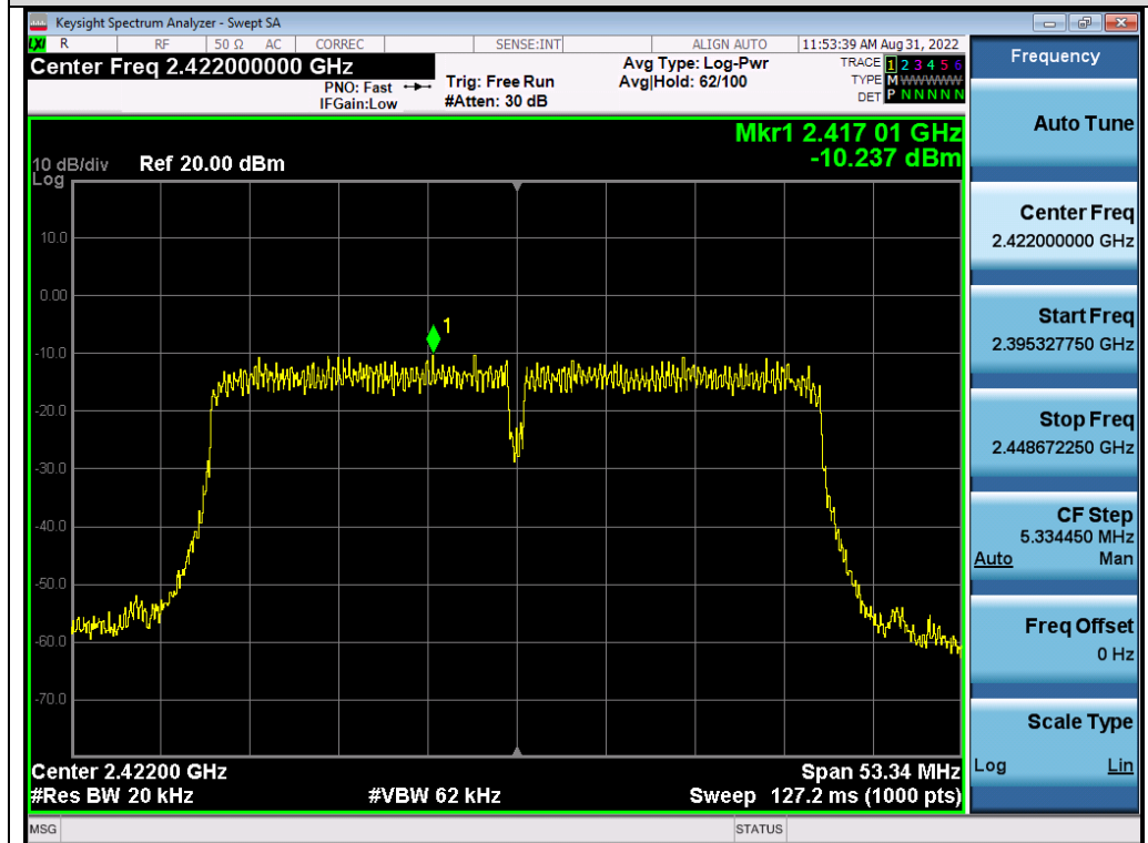
Test_Graph_802.11n40_ANT3_2422_MCS0_PSD
