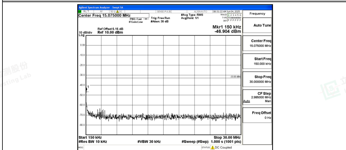
Band66_20MHz_QPSK_132072_1RB#0_0.15~30_0.15~30
