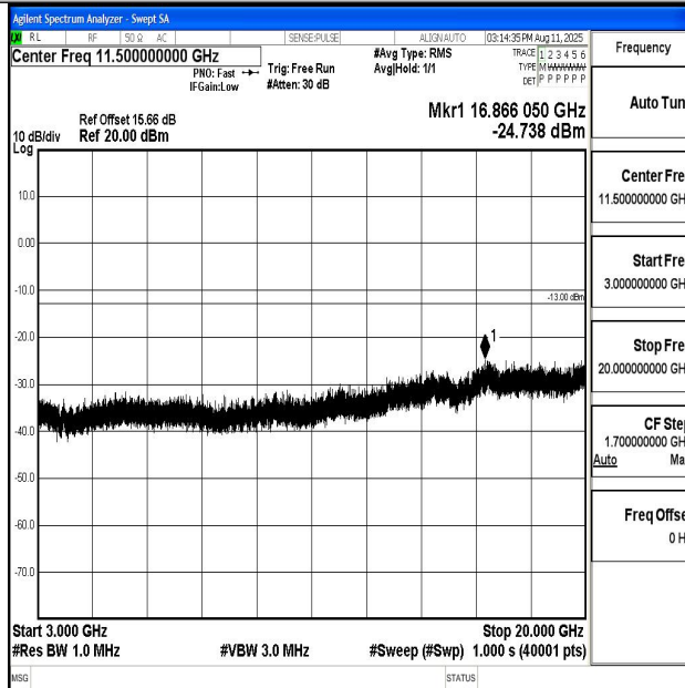
Band66_20MHz_QPSK_132572_1RB#0_3000~20000_3000~20000
