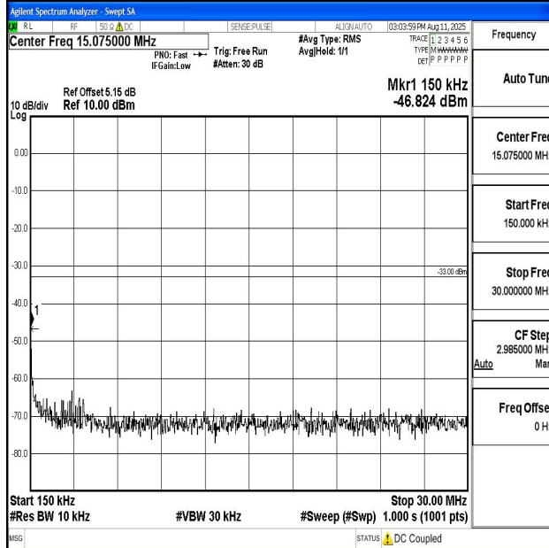
Band66_10MHz_QPSK_132022_1RB#0_0.15~30_0.15~30
