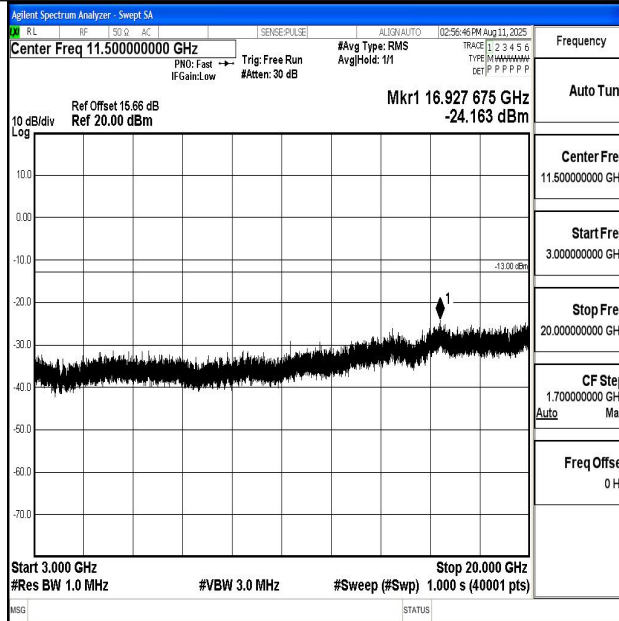
Band66_3MHz_QPSK_132322_1RB#0_3000~20000_3000~20000
