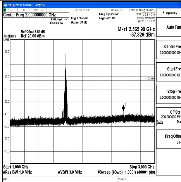
Band66_20MHz_16QAM_132572_1RB#0_1000~3000_1000~3000
