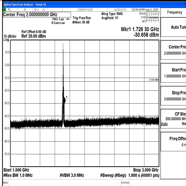
Band66_5MHz_QPSK_131997_1RB#0_1000~3000_1000~3000
