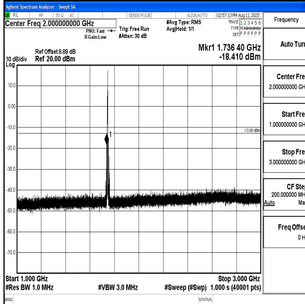
Band66_3MHz_16QAM_132322_1RB#0_1000~3000_1000~3000
