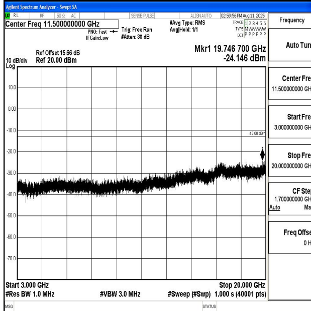
Band66_5MHz_QPSK_131997_1RB#0_3000~20000_3000~20000
