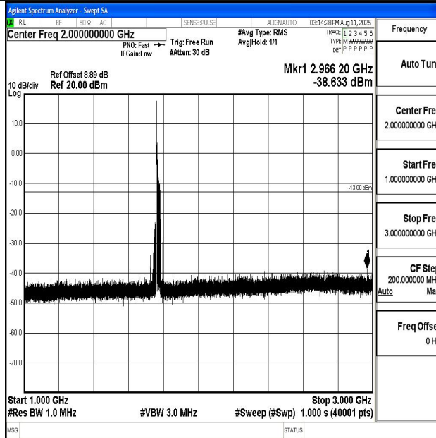
Band66_20MHz_QPSK_132572_1RB#0_1000~3000_1000~3000
