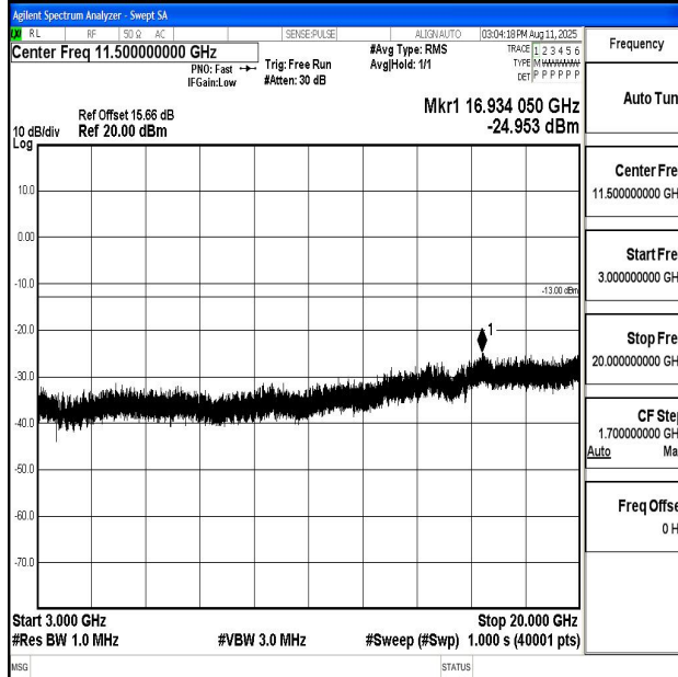
Band66_10MHz_QPSK_132022_1RB#0_3000~20000_3000~20000
