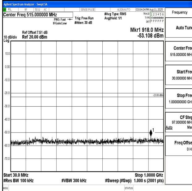
Band66_10MHz_QPSK_132022_1RB#0_30~1000_30~1000
