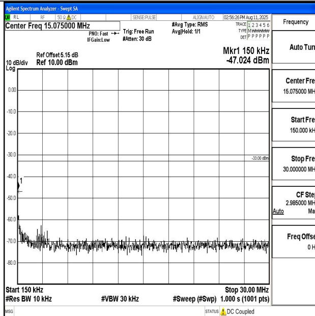
Band66_3MHz_QPSK_132322_1RB#0_0.15~30_0.15~30
