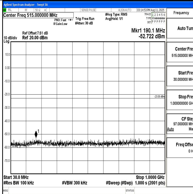
Band66_20MHz_16QAM_132572_1RB#0_30~1000_30~1000
