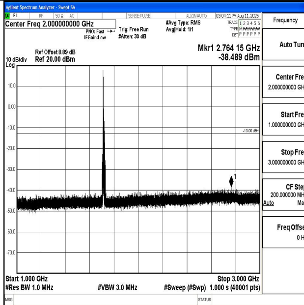
Band66_10MHz_QPSK_132022_1RB#0_1000~3000_1000~3000
