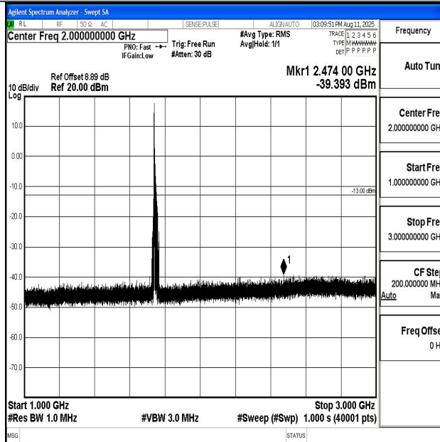
Band66_15MHz_16QAM_132322_1RB#0_1000~3000_1000~3000
