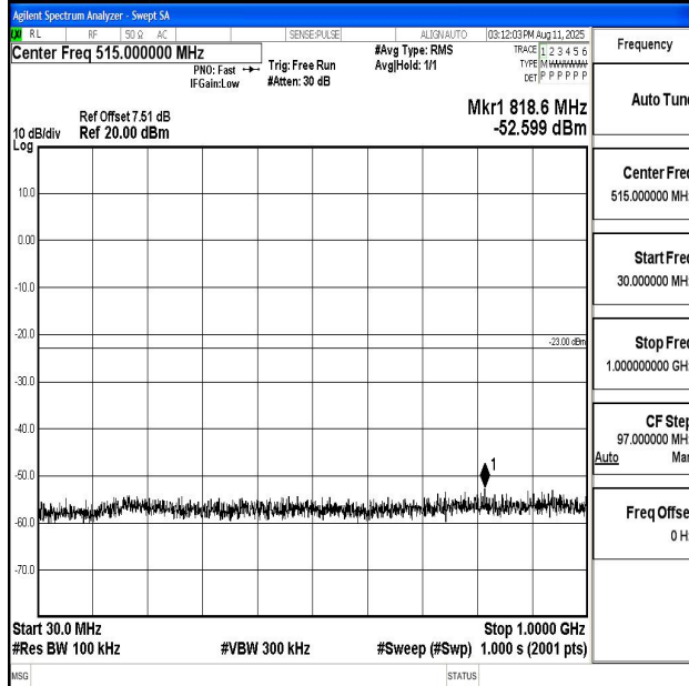
Band66_20MHz_QPSK_132072_1RB#0_30~1000_30~1000
