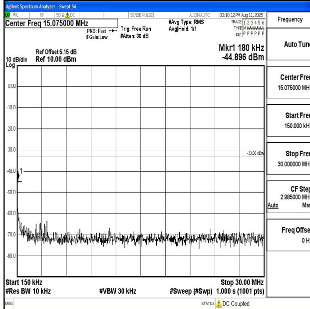
Band66_15MHz_QPSK_132597_1RB#0_0.15~30_0.15~30
