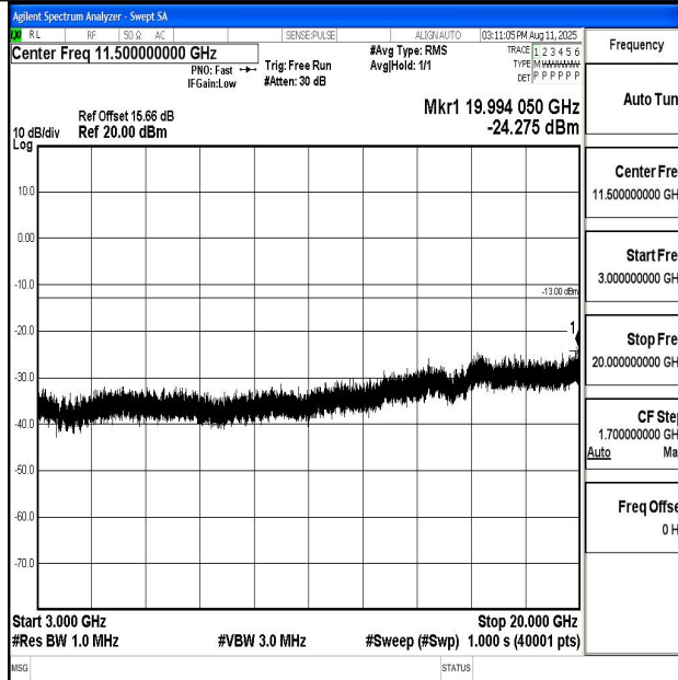
Band66_15MHz_16QAM_132597_1RB#0_3000~20000_3000~20000
