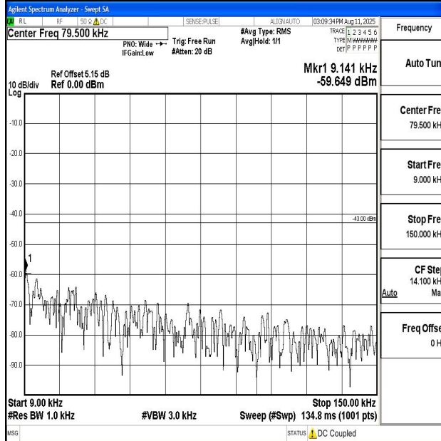
Band66_15MHz_16QAM_132322_1RB#0_0.009~0.15_0.009~0.15
