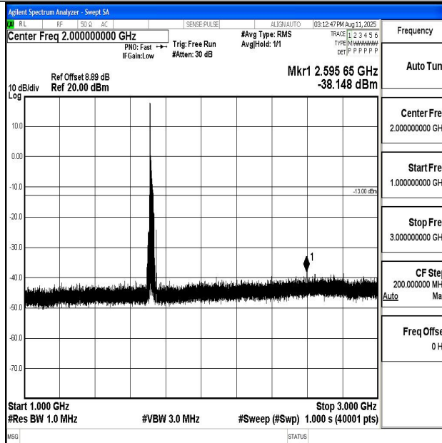
Band66_20MHz_16QAM_132072_1RB#0_1000~3000_1000~3000
