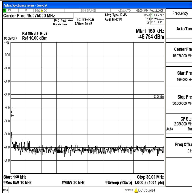
Band66_15MHz_16QAM_132322_1RB#0_0.15~30_0.15~30
