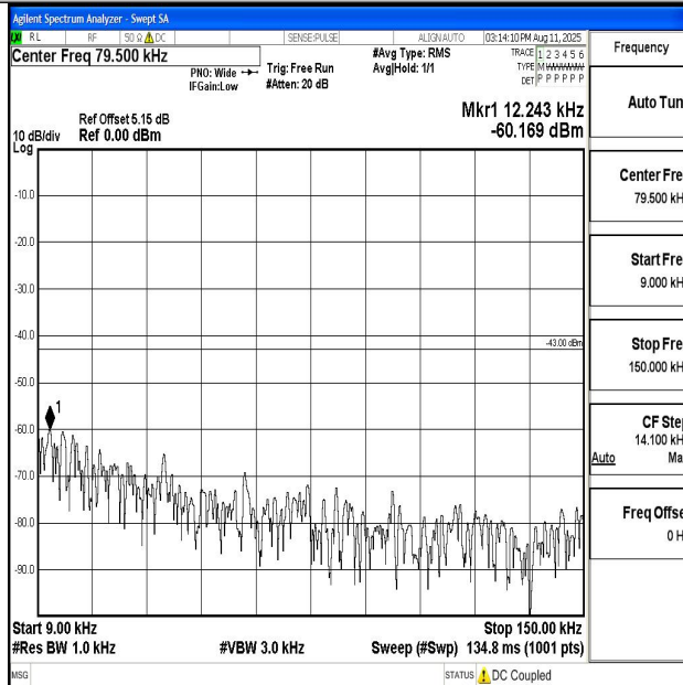
Band66_20MHz_QPSK_132572_1RB#0_0.009~0.15_0.009~0.15
