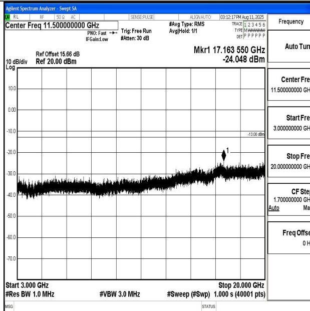
Band66_20MHz_QPSK_132072_1RB#0_3000~20000_3000~20000
