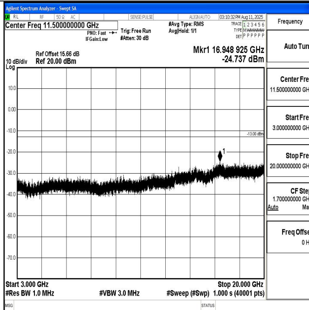
Band66_15MHz_QPSK_132597_1RB#0_3000~20000_3000~20000
