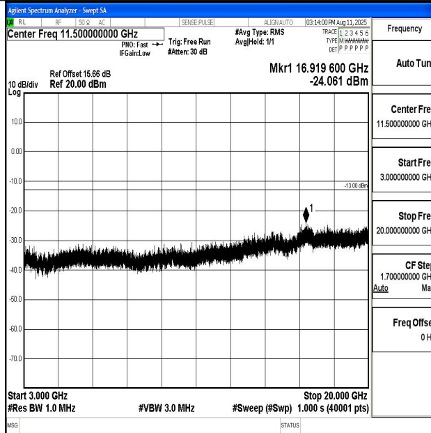
Band66_20MHz_16QAM_132322_1RB#0_3000~20000_3000~20000
