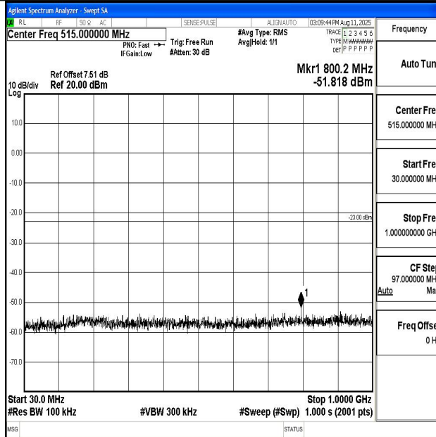
Band66_15MHz_16QAM_132322_1RB#0_30~1000_30~1000
