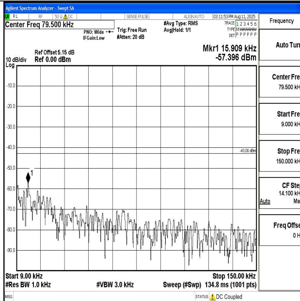
Band66_20MHz_QPSK_132072_1RB#0_0.009~0.15_0.009~0.15
