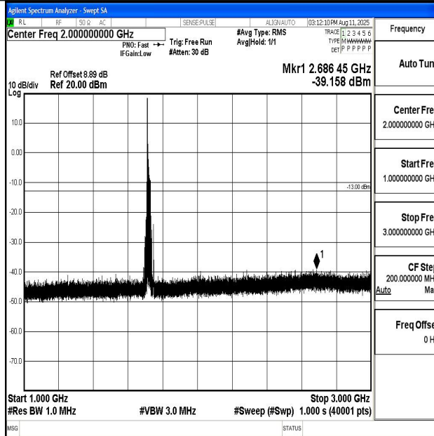
Band66_20MHz_QPSK_132072_1RB#0_1000~3000_1000~3000
