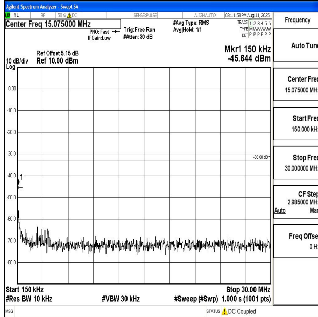
Band66_20MHz_QPSK_132072_1RB#0_0.15~30_0.15~30
