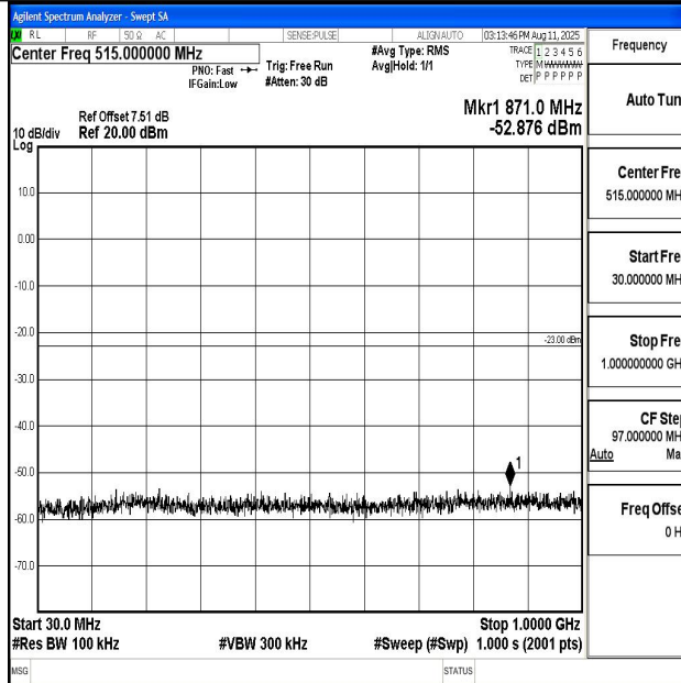
Band66_20MHz_16QAM_132322_1RB#0_30~1000_30~1000
