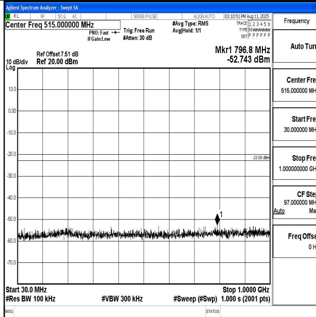
Band66_15MHz_16QAM_132597_1RB#0_30~1000_30~1000
