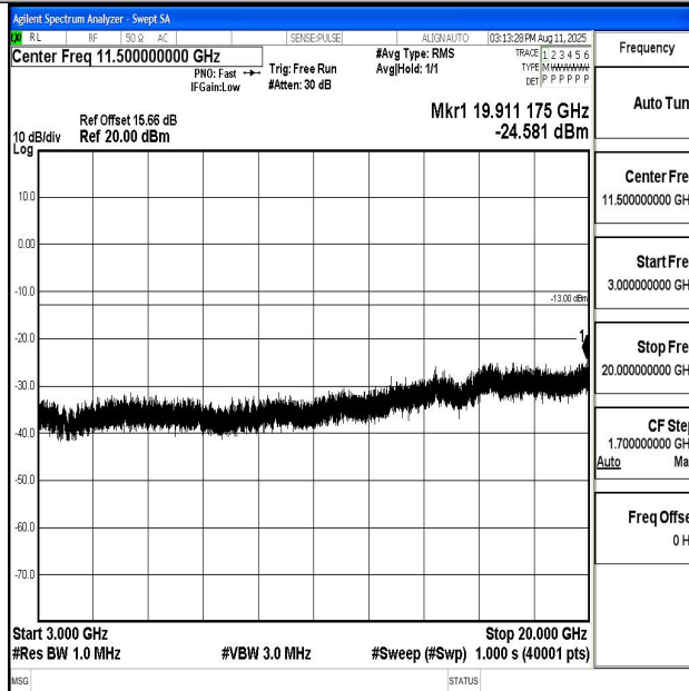
Band66_20MHz_QPSK_132322_1RB#0_3000~20000_3000~20000
