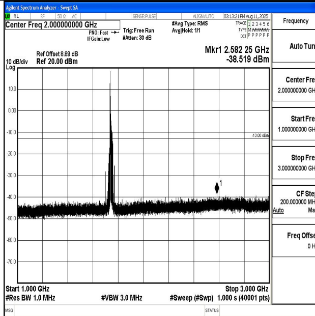
Band66_20MHz_QPSK_132322_1RB#0_1000~3000_1000~3000
