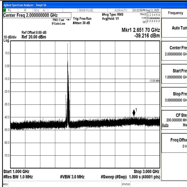
Band66_15MHz_16QAM_132597_1RB#0_1000~3000_1000~3000
