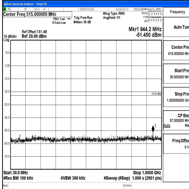
Band66_20MHz_16QAM_132072_1RB#0_30~1000_30~1000
