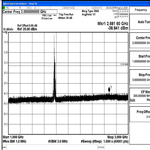
Band66_15MHz_QPSK_132597_1RB#0_1000~3000_1000~3000
