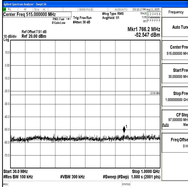
Band66_15MHz_QPSK_132597_1RB#0_30~1000_30~1000
