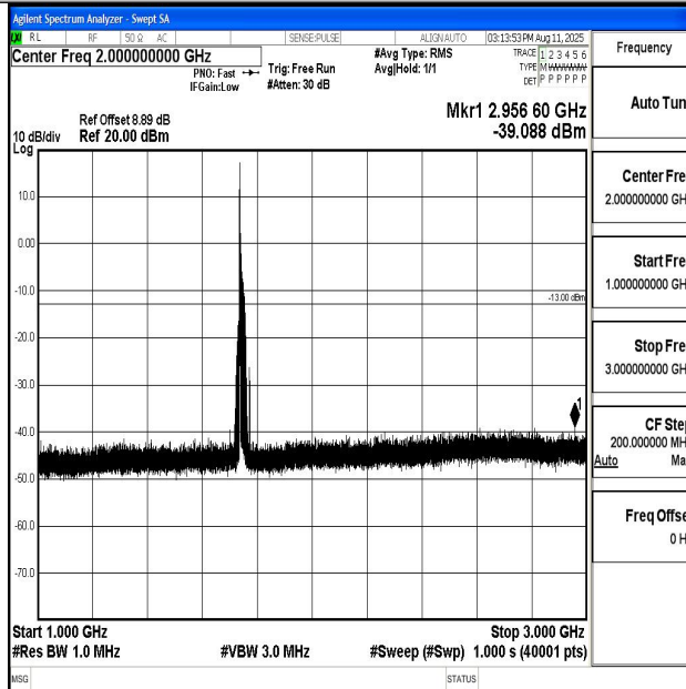
Band66_20MHz_16QAM_132322_1RB#0_1000~3000_1000~3000
