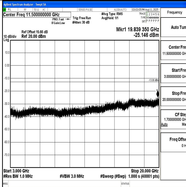
Band66_5MHz_16QAM_132647_1RB#0_3000~20000_3000~20000
