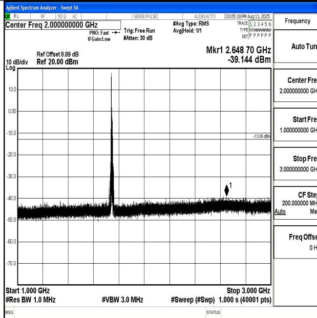
Band66_10MHz_QPSK_132322_1RB#0_1000~3000_1000~3000
