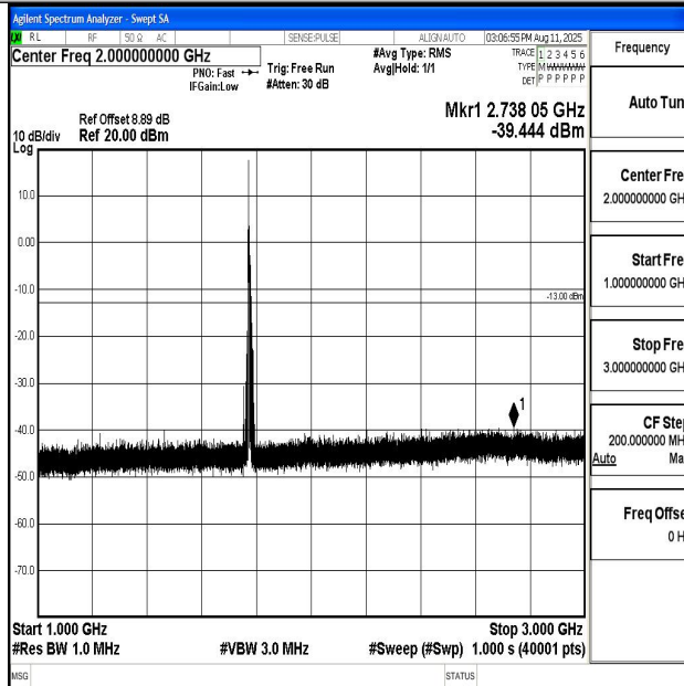
Band66_10MHz_16QAM_132622_1RB#0_1000~3000_1000~3000
