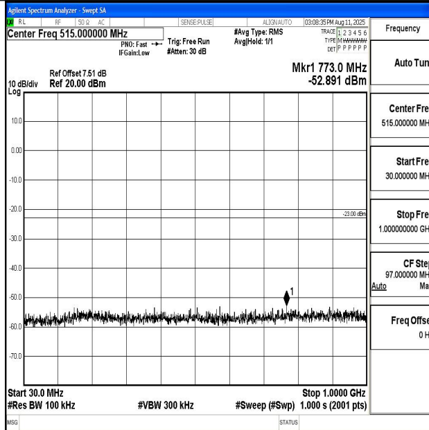
Band66_15MHz_16QAM_132047_1RB#0_30~1000_30~1000
