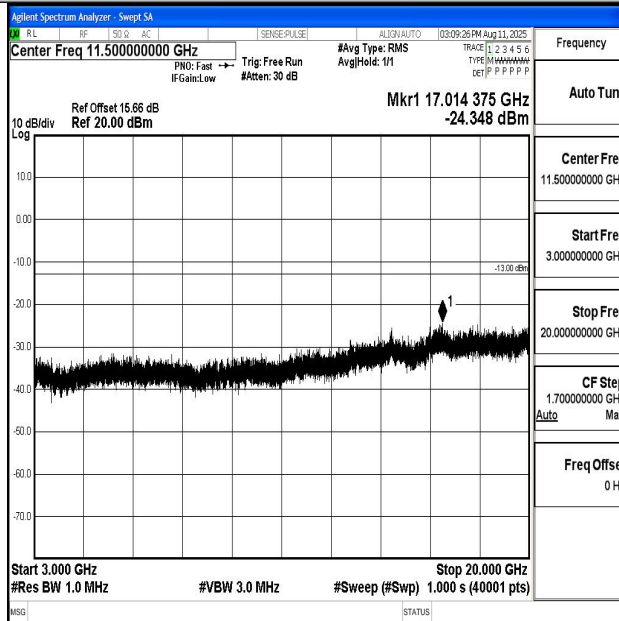
Band66_15MHz_QPSK_132322_1RB#0_3000~20000_3000~20000
