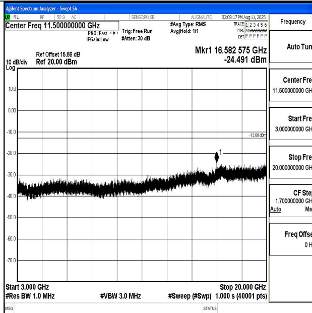
Band66_15MHz_QPSK_132047_1RB#0_3000~20000_3000~20000
