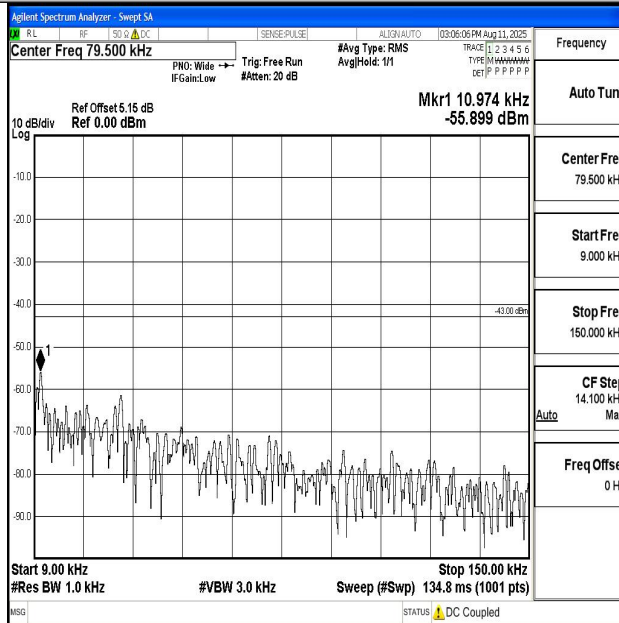
Band66_10MHz_QPSK_132622_1RB#0_0.009~0.15_0.009~0.15
