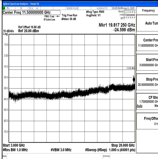
Band66_10MHz_16QAM_132322_1RB#0_3000~20000_3000~20000
