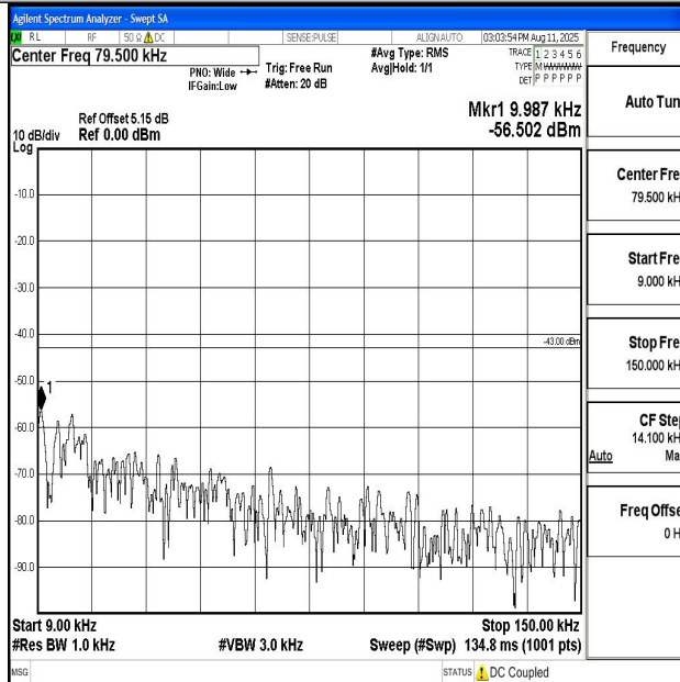
Band66_10MHz_QPSK_132022_1RB#0_0.009~0.15_0.009~0.15
