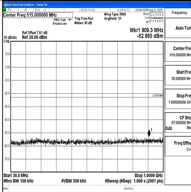
Band66_10MHz_16QAM_132622_1RB#0_30~1000_30~1000
