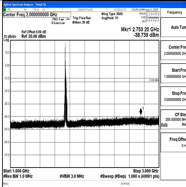
Band66_15MHz_QPSK_132322_1RB#0_1000~3000_1000~3000
