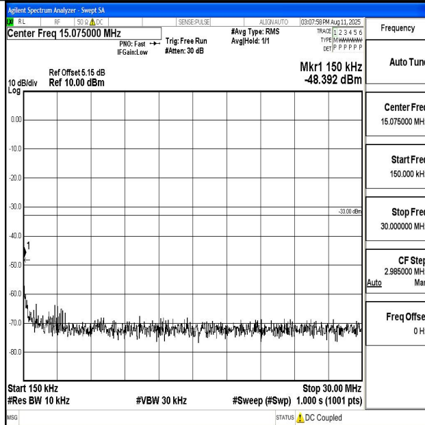
Band66_15MHz_QPSK_132047_1RB#0_0.15~30_0.15~30
