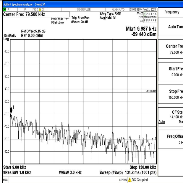
Band66_10MHz_16QAM_132322_1RB#0_0.009~0.15_0.009~0.15
