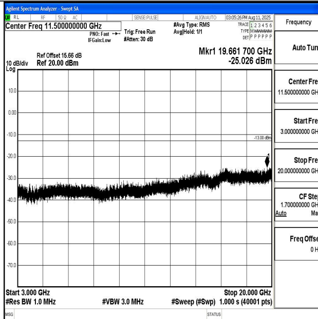
Band66_10MHz_QPSK_132322_1RB#0_3000~20000_3000~20000
