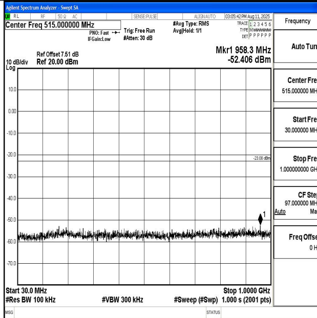
Band66_10MHz_16QAM_132322_1RB#0_30~1000_30~1000
