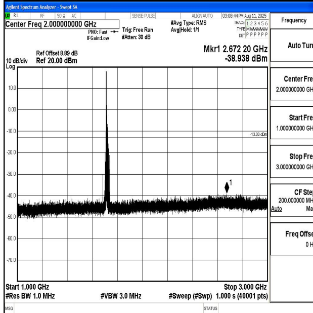
Band66_15MHz_16QAM_132047_1RB#0_1000~3000_1000~3000
