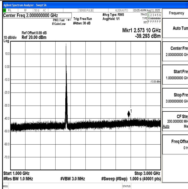
Band66_10MHz_16QAM_132322_1RB#0_1000~3000_1000~3000
