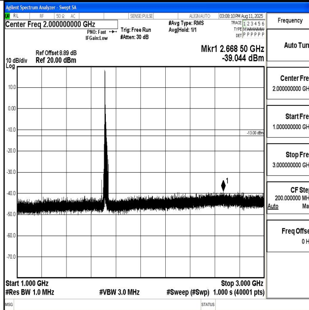
Band66_15MHz_QPSK_132047_1RB#0_1000~3000_1000~3000
