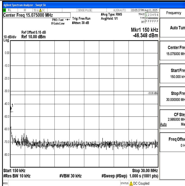
Band66_10MHz_16QAM_132322_1RB#0_0.15~30_0.15~30
