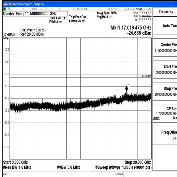
Band66_5MHz_QPSK_132322_1RB#0_3000~20000_3000~20000
