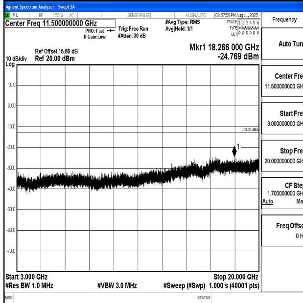
Band66_3MHz_QPSK_132657_1RB#0_3000~20000_3000~20000
