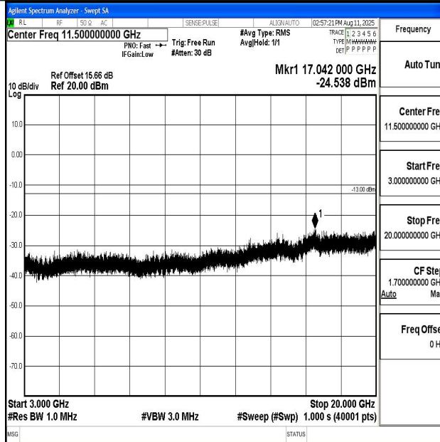
Band66_3MHz_16QAM_132322_1RB#0_3000~20000_3000~20000
