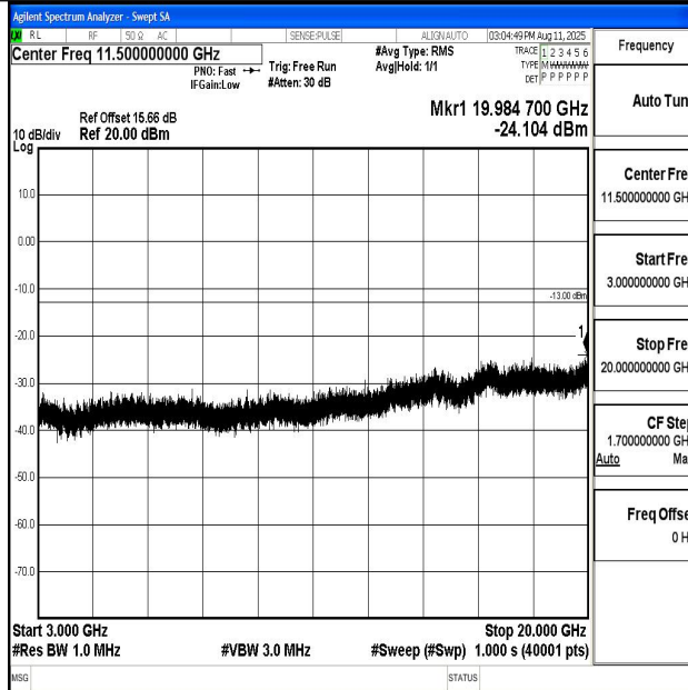
Band66_10MHz_16QAM_132022_1RB#0_3000~20000_3000~20000
