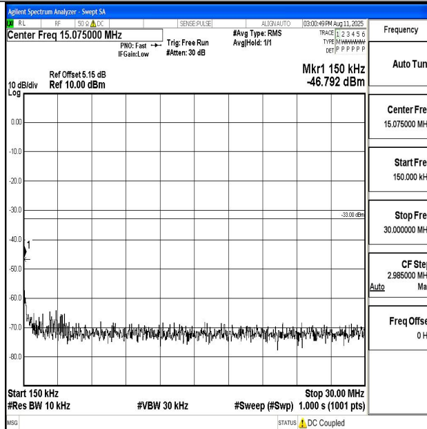
Band66_5MHz_QPSK_132322_1RB#0_0.15~30_0.15~30
