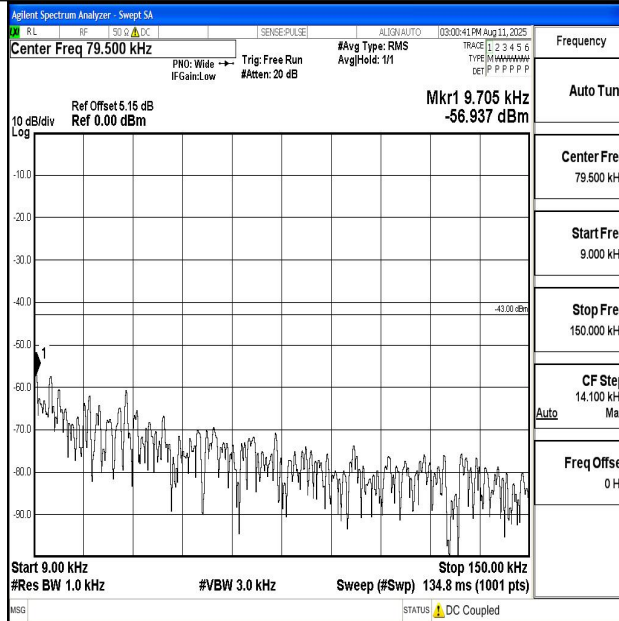
Band66_5MHz_QPSK_132322_1RB#0_0.009~0.15_0.009~0.15
