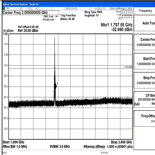
Band66_5MHz_16QAM_132322_1RB#0_1000~3000_1000~3000
