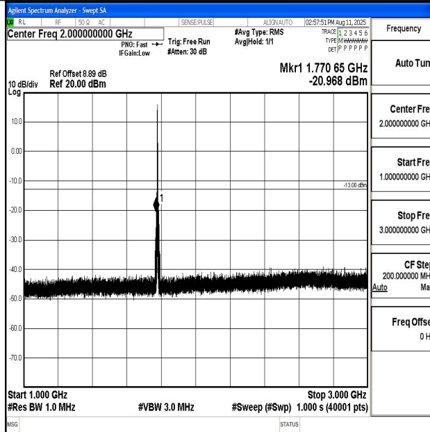
Band66_3MHz_QPSK_132657_1RB#0_1000~3000_1000~3000
