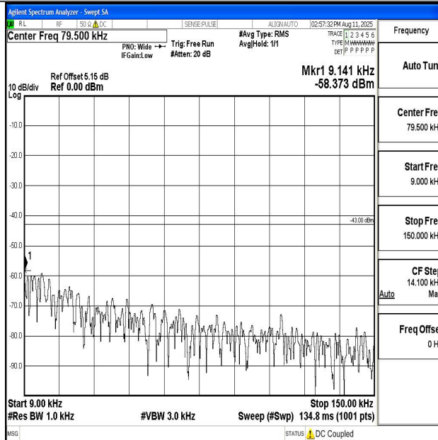
Band66_3MHz_QPSK_132657_1RB#0_0.009~0.15_0.009~0.15
