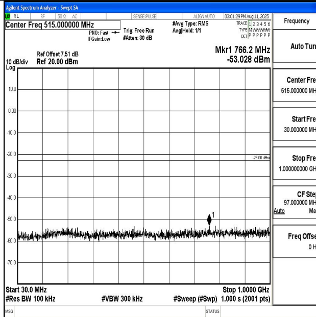
Band66_5MHz_16QAM_132322_1RB#0_30~1000_30~1000
