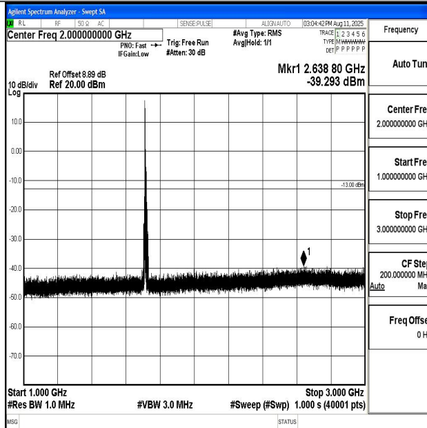
Band66_10MHz_16QAM_132022_1RB#0_1000~3000_1000~3000
