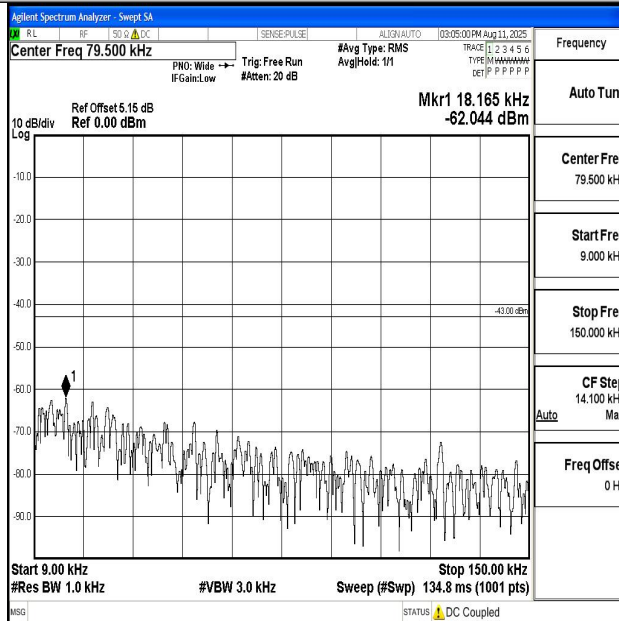
Band66_10MHz_QPSK_132322_1RB#0_0.009~0.15_0.009~0.15
