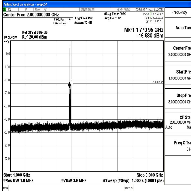
Band66_3MHz_16QAM_132657_1RB#0_1000~3000_1000~3000
