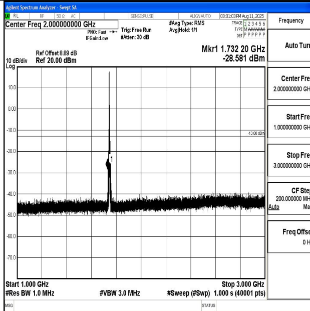
Band66_5MHz_QPSK_132322_1RB#0_1000~3000_1000~3000
