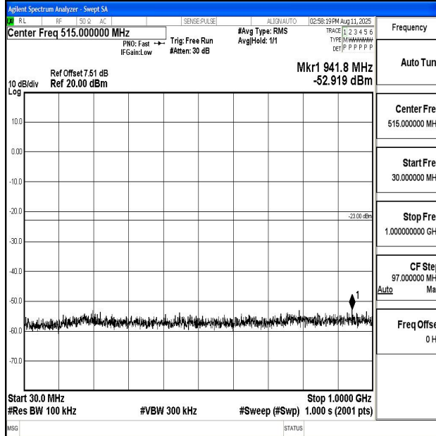
Band66_3MHz_16QAM_132657_1RB#0_30~1000_30~1000
