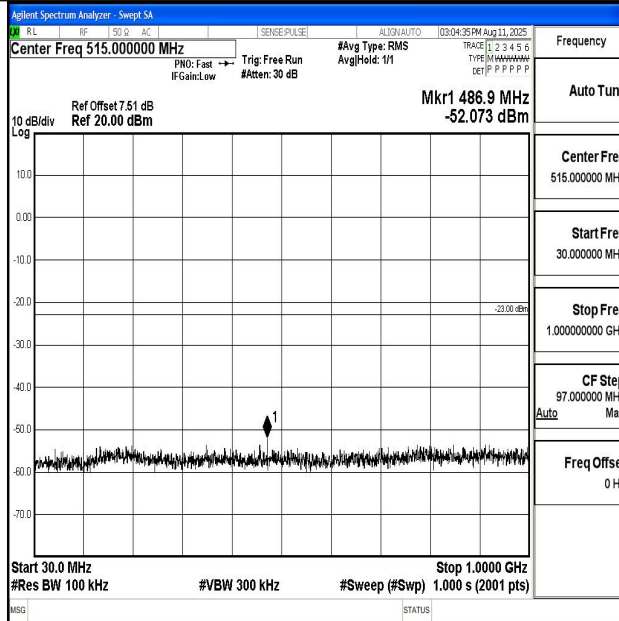
Band66_10MHz_16QAM_132022_1RB#0_30~1000_30~1000
