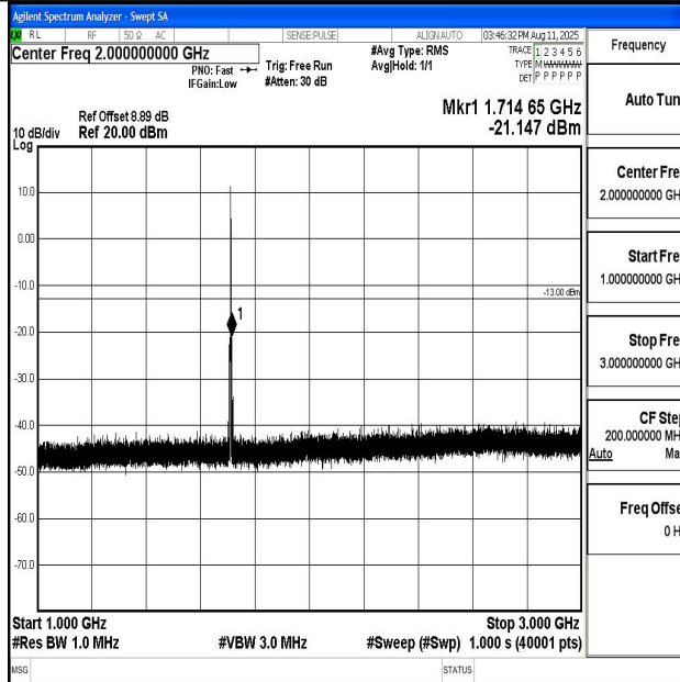
Band66_1.4MHz_16QAM_131979_1RB#0_1000~3000_1000~3000
