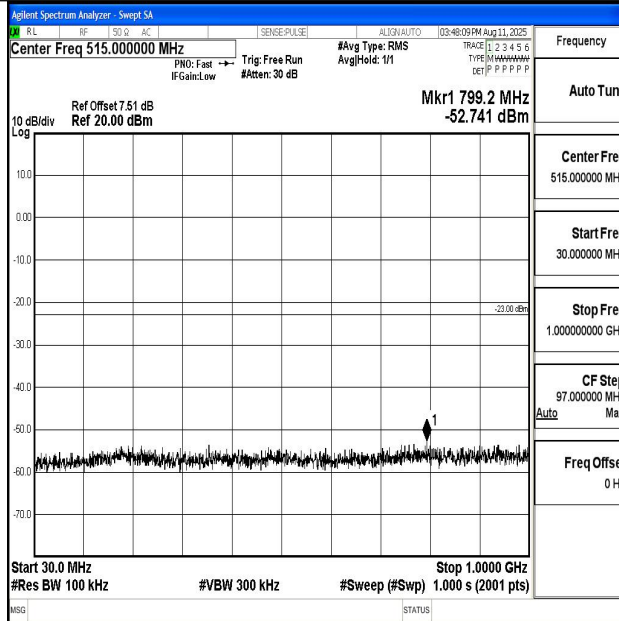
Band66_1.4MHz_QPSK_132665_1RB#0_30~1000_30~1000
