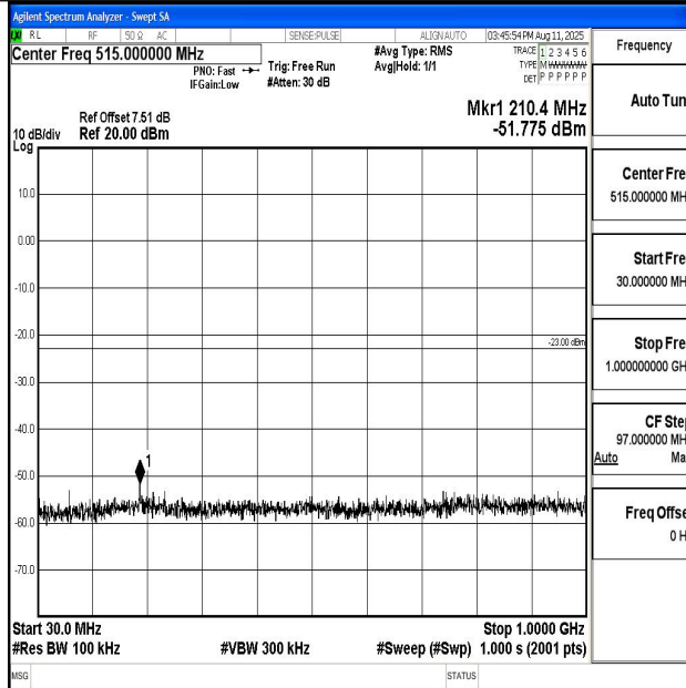
Band66_1.4MHz_QPSK_131979_1RB#0_30~1000_30~1000
