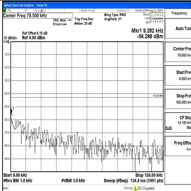
Band66_1.4MHz_16QAM_131979_1RB#0_0.009~0.15_0.009~0.15
