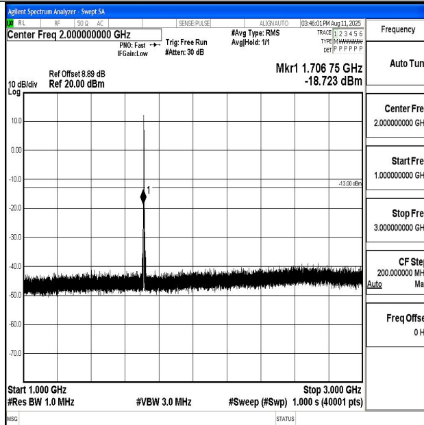
Band66_1.4MHz_QPSK_131979_1RB#0_1000~3000_1000~3000
