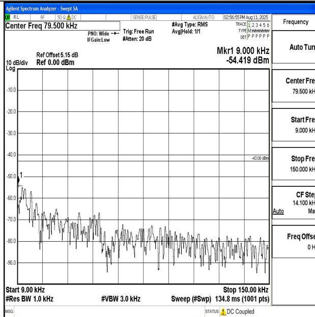
Band66_3MHz_16QAM_132322_1RB#0_0.009~0.15_0.009~0.15
