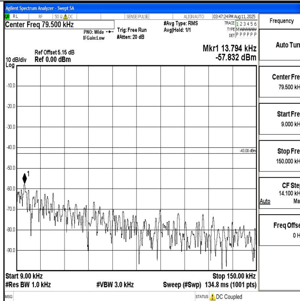
Band66_1.4MHz_16QAM_132322_1RB#0_0.009~0.15_0.009~0.15
