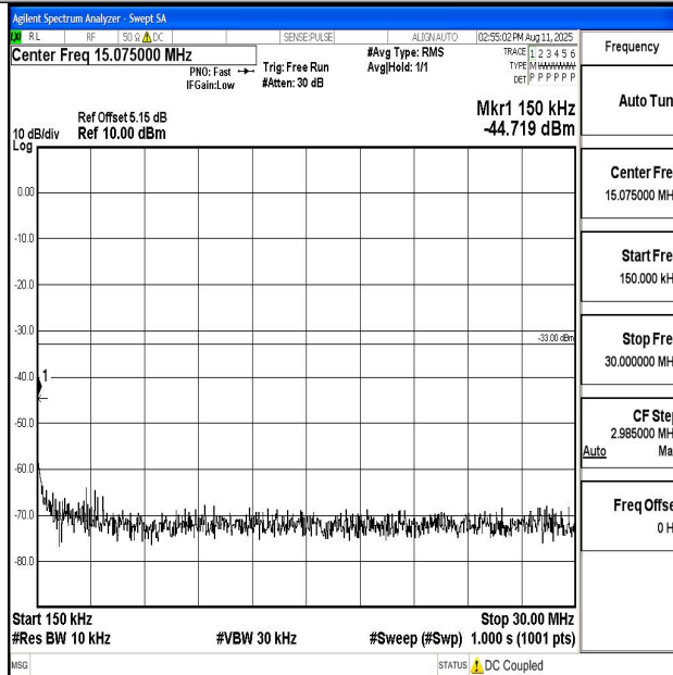
Band66_3MHz_QPSK_131987_1RB#0_0.15~30_0.15~30
