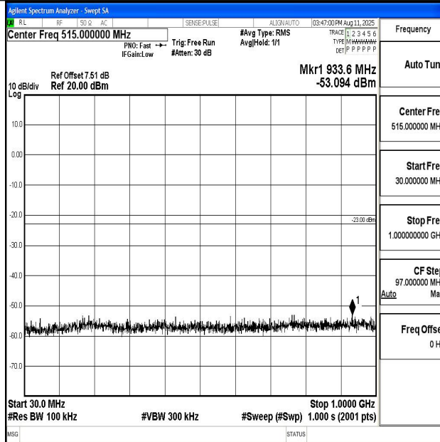
Band66_1.4MHz_QPSK_132322_1RB#0_30~1000_30~1000
