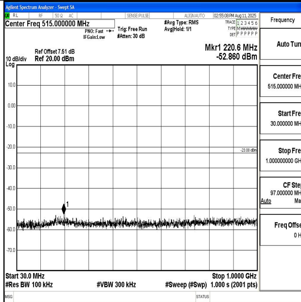
Band66_3MHz_QPSK_131987_1RB#0_30~1000_30~1000
