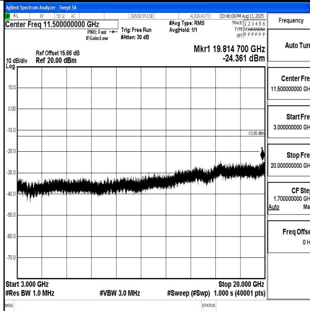
Band66_1.4MHz_QPSK_131979_1RB#0_3000~20000_3000~20000
