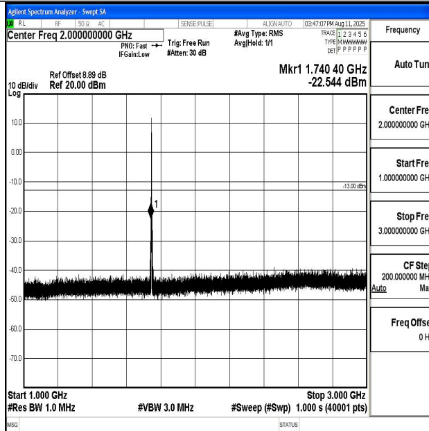
Band66_1.4MHz_QPSK_132322_1RB#0_1000~3000_1000~3000
