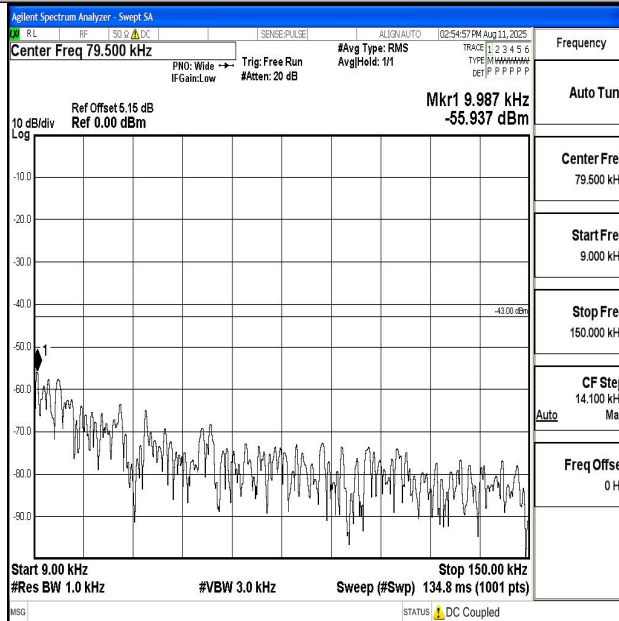
Band66_3MHz_QPSK_131987_1RB#0_0.009~0.15_0.009~0.15
