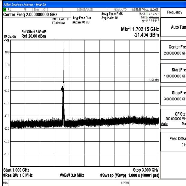
Band66_3MHz_16QAM_131987_1RB#0_1000~3000_1000~3000
