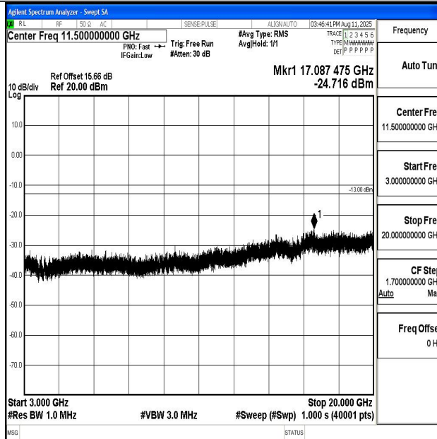
Band66_1.4MHz_16QAM_131979_1RB#0_3000~20000_3000~20000
