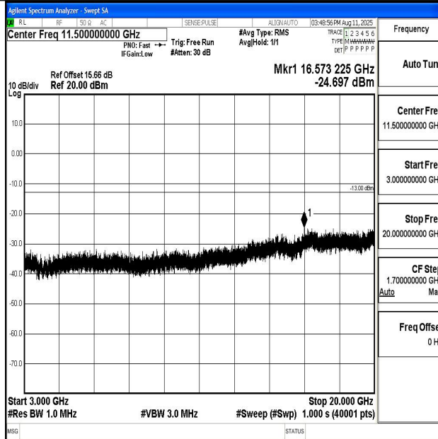
Band66_1.4MHz_16QAM_132665_1RB#0_3000~20000_3000~20000
