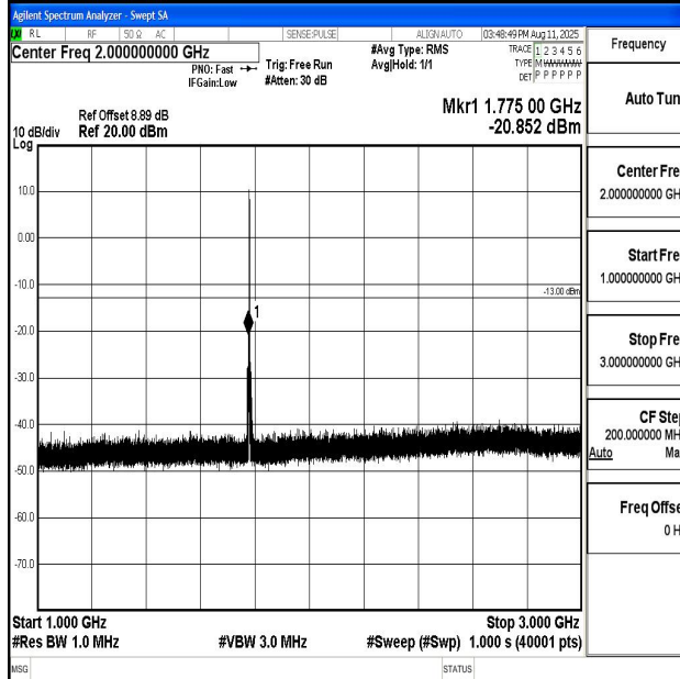
Band66_1.4MHz_16QAM_132665_1RB#0_1000~3000_1000~3000
