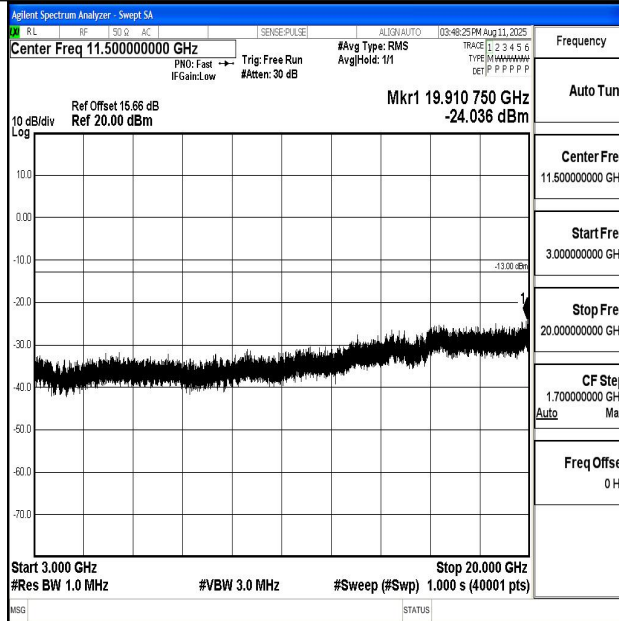
Band66_1.4MHz_QPSK_132665_1RB#0_3000~20000_3000~20000
