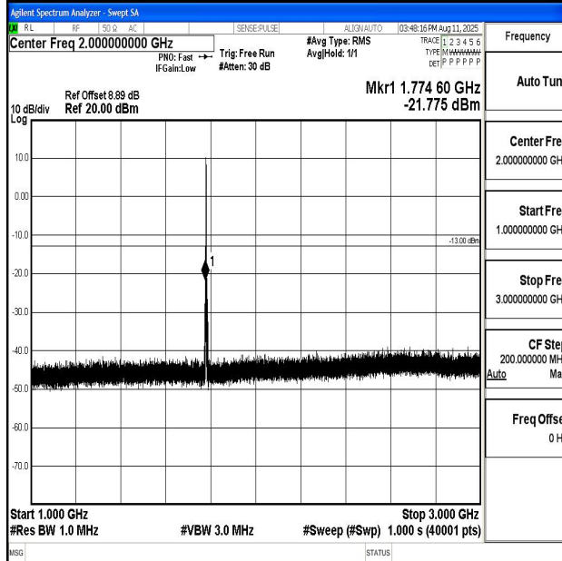
Band66_1.4MHz_QPSK_132665_1RB#0_1000~3000_1000~3000
