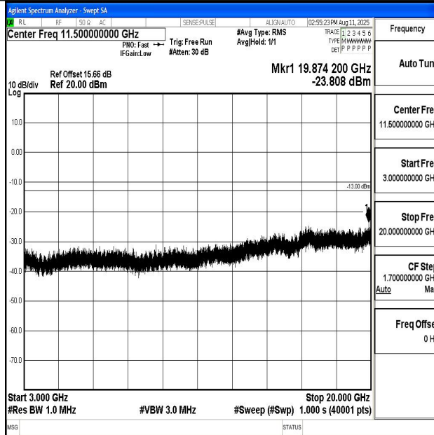
Band66_3MHz_QPSK_131987_1RB#0_3000~20000_3000~20000
