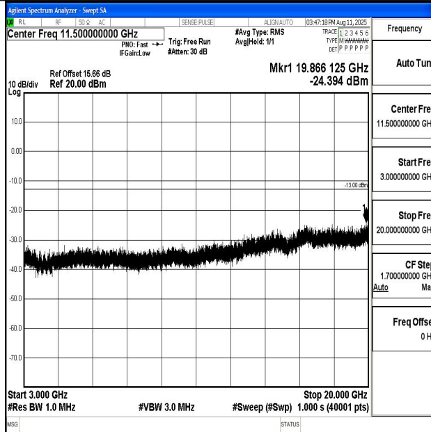
Band66_1.4MHz_QPSK_132322_1RB#0_3000~20000_3000~20000
