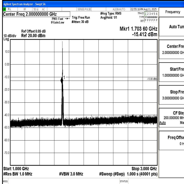
Band66_3MHz_QPSK_131987_1RB#0_1000~3000_1000~3000
