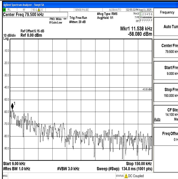
Band66_3MHz_16QAM_131987_1RB#0_0.009~0.15_0.009~0.15
