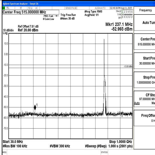
Band13_10MHz_16QAM_23230_1RB#0_30~1000_30~1000
