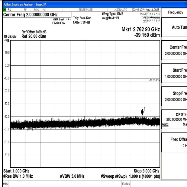
Band13_10MHz_QPSK_23230_1RB#0_1000~3000_1000~3000
