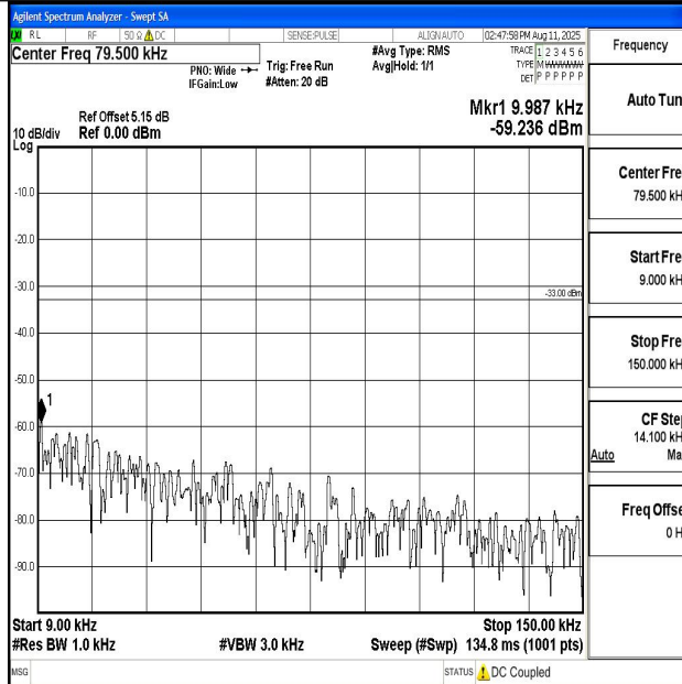
Band13_5MHz_16QAM_23255_1RB#0_0.009~0.15_0.009~0.15
