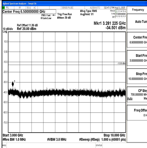
Band13_5MHz_16QAM_23230_1RB#0_3000~10000_3000~10000
