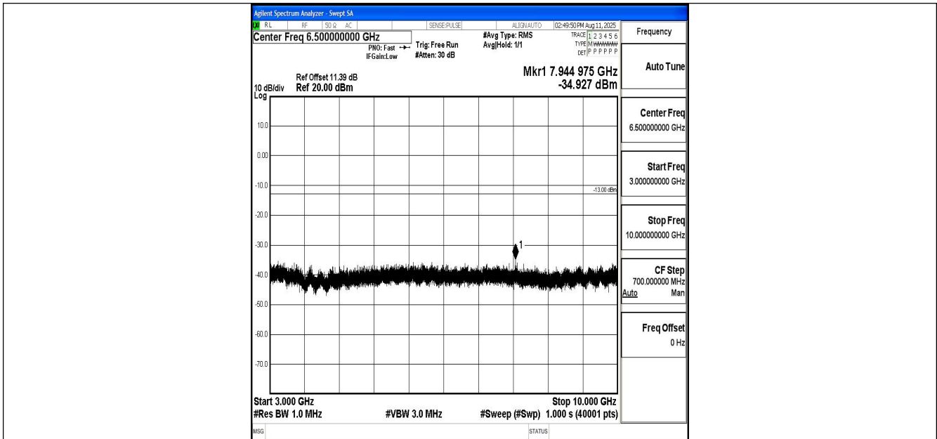
Band13_10MHz_16QAM_23230_1RB#0_3000~10000_3000~10000
