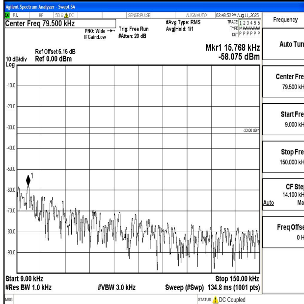
Band13_10MHz_QPSK_23230_1RB#0_0.009~0.15_0.009~0.15
