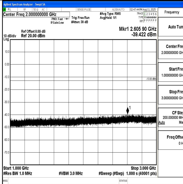
Band13_5MHz_QPSK_23255_1RB#0_1000~3000_1000~3000
