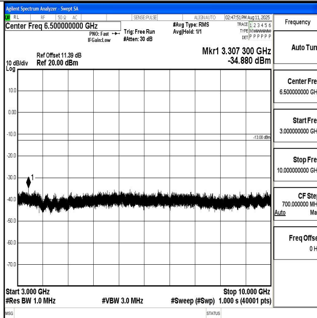
Band13_5MHz_QPSK_23255_1RB#0_3000~10000_3000~10000
