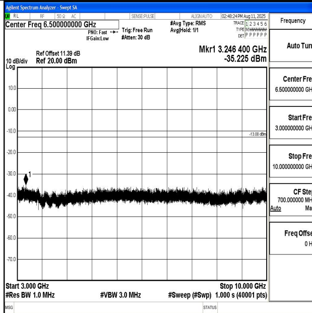
Band13_5MHz_16QAM_23255_1RB#0_3000~10000_3000~10000
