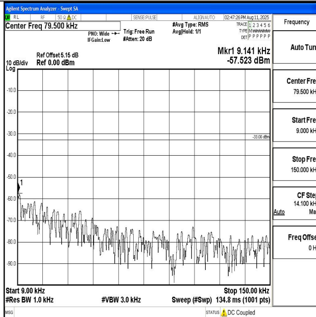
Band13_5MHz_QPSK_23255_1RB#0_0.009~0.15_0.009~0.15
