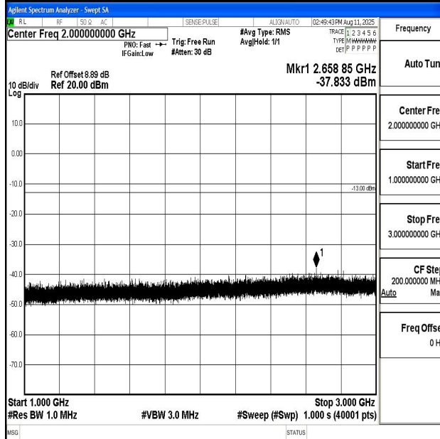
Band13_10MHz_16QAM_23230_1RB#0_1000~3000_1000~3000
