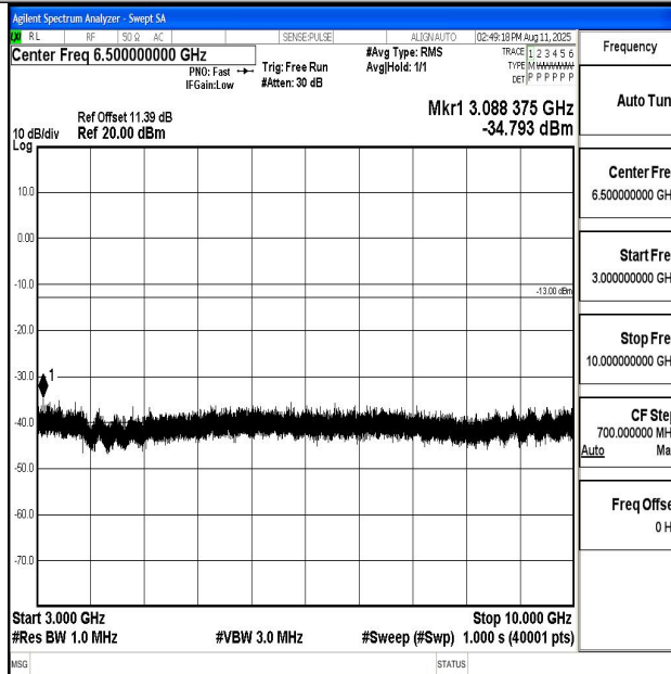
Band13_10MHz_QPSK_23230_1RB#0_3000~10000_3000~10000
