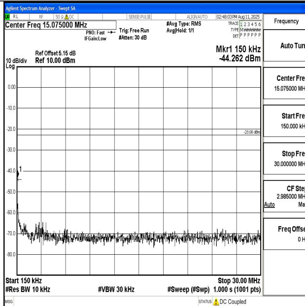
Band13_5MHz_16QAM_23255_1RB#0_0.15~30_0.15~30
