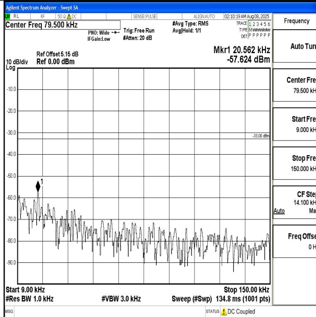
Band12_3MHz_QPSK_23165_1RB#0_0.009~0.15_0.009~0.15
