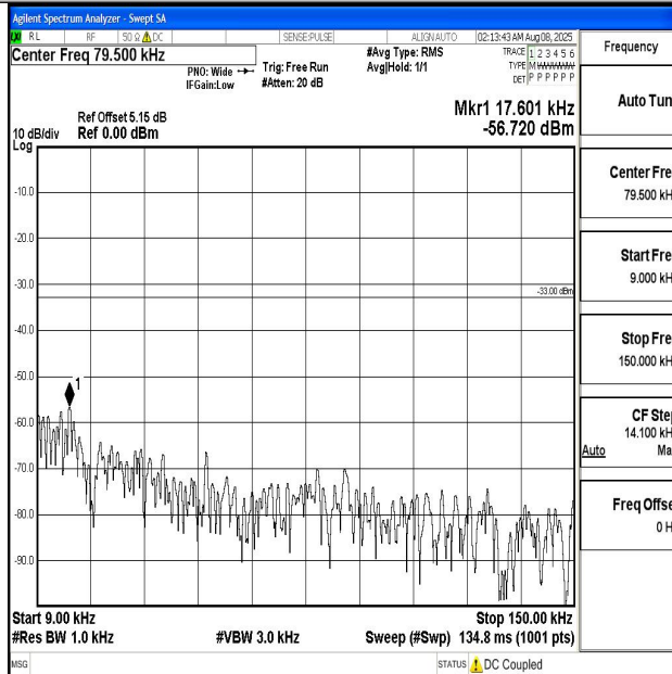
Band12_5MHz_16QAM_23095_1RB#0_0.009~0.15_0.009~0.15
