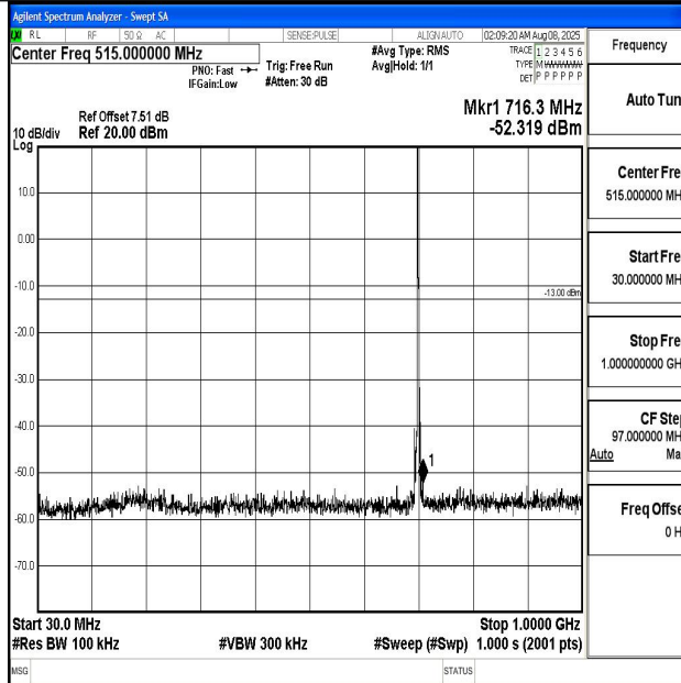
Band12_3MHz_QPSK_23095_1RB#0_30~1000_30~1000
