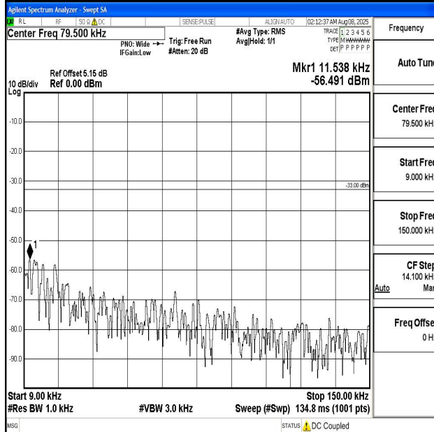
Band12_5MHz_16QAM_23035_1RB#0_0.009~0.15_0.009~0.15
