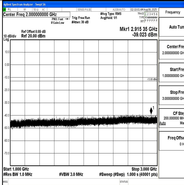
Band12_3MHz_16QAM_23095_1RB#0_1000~3000_1000~3000
