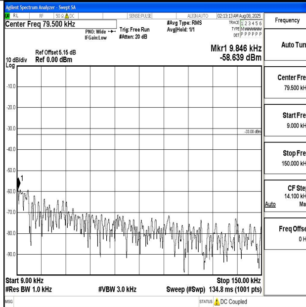
Band12_5MHz_QPSK_23095_1RB#0_0.009~0.15_0.009~0.15
