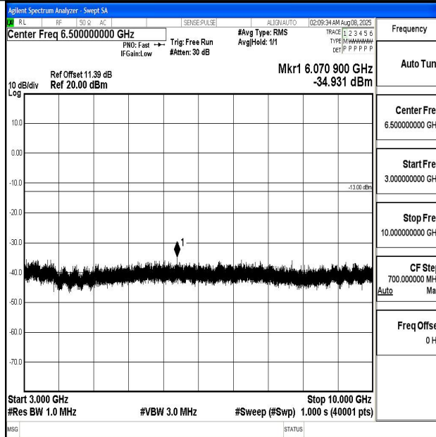
Band12_3MHz_QPSK_23095_1RB#0_3000~10000_3000~10000
