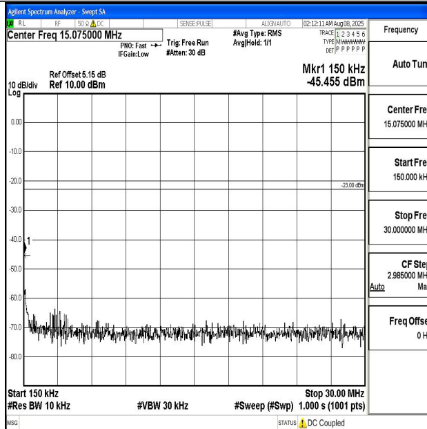
Band12_5MHz_QPSK_23035_1RB#0_0.15~30_0.15~30
