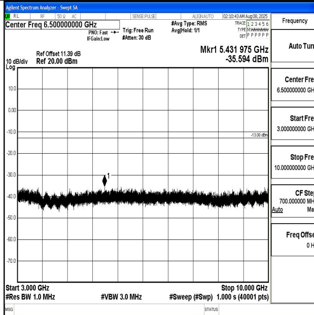
Band12_3MHz_QPSK_23165_1RB#0_3000~10000_3000~10000
