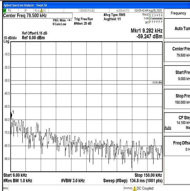
Band12_3MHz_16QAM_23095_1RB#0_0.009~0.15_0.009~0.15
