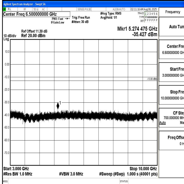
Band12_3MHz_16QAM_23165_1RB#0_3000~10000_3000~10000
