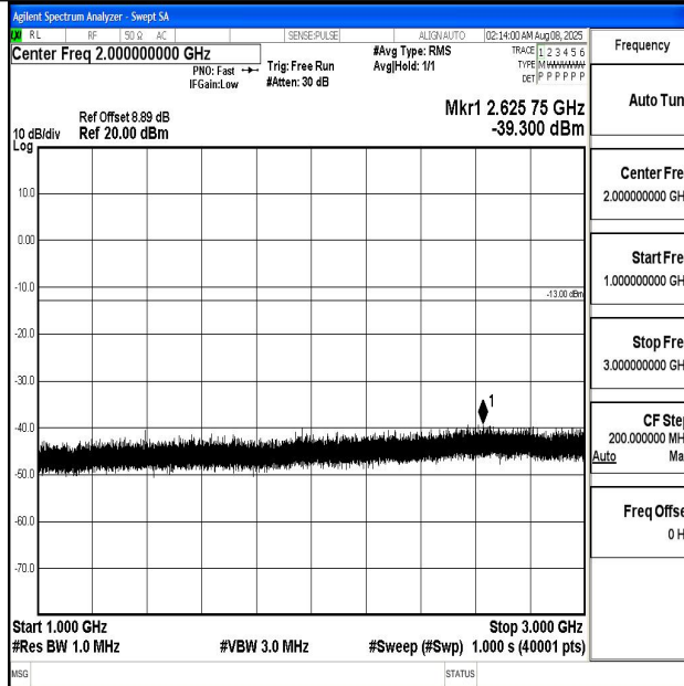
Band12_5MHz_16QAM_23095_1RB#0_1000~3000_1000~3000
