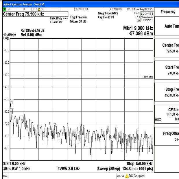
Band12_5MHz_QPSK_23035_1RB#0_0.009~0.15_0.009~0.15
