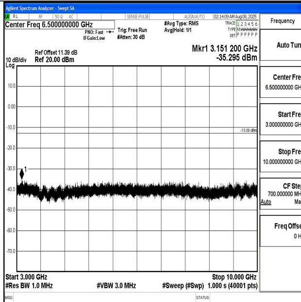
Band12_5MHz_16QAM_23095_1RB#0_3000~10000_3000~10000
