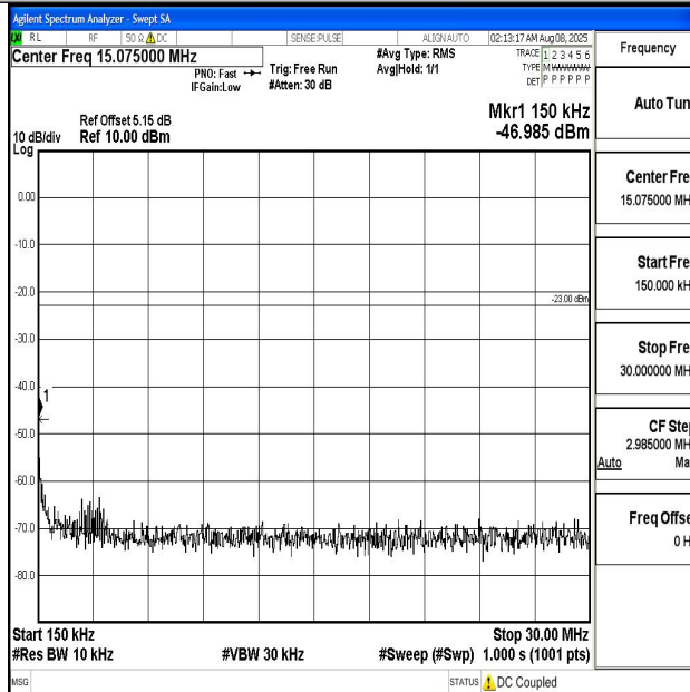
Band12_5MHz_QPSK_23095_1RB#0_0.15~30_0.15~30
