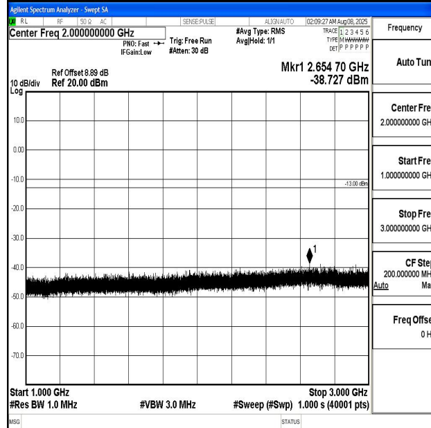
Band12_3MHz_QPSK_23095_1RB#0_1000~3000_1000~3000
