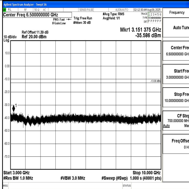
Band12_5MHz_QPSK_23035_1RB#0_3000~10000_3000~10000
