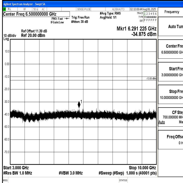
Band12_3MHz_16QAM_23095_1RB#0_3000~10000_3000~10000
