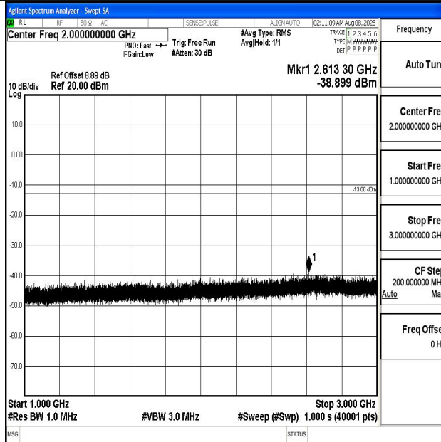
Band12_3MHz_16QAM_23165_1RB#0_1000~3000_1000~3000
