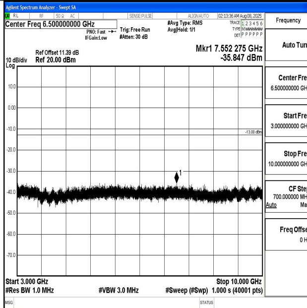
Band12_5MHz_QPSK_23095_1RB#0_3000~10000_3000~10000
