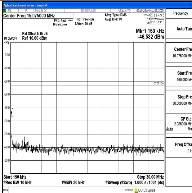
Band12_3MHz_QPSK_23165_1RB#0_0.15~30_0.15~30
