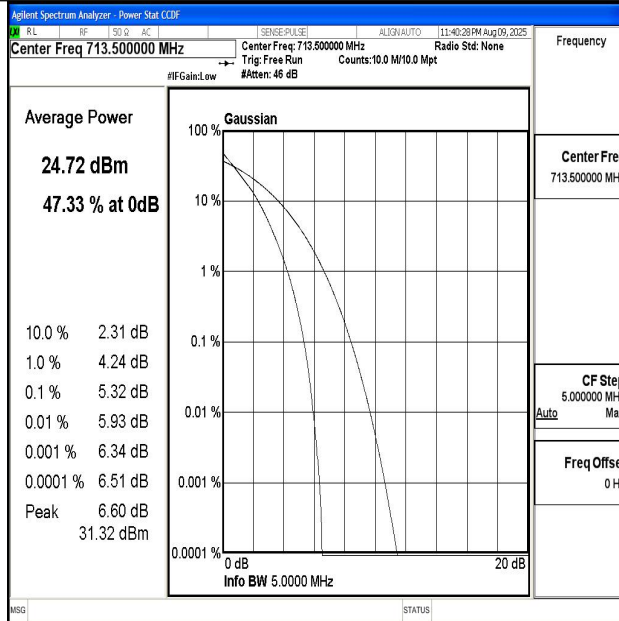
Band12-5MHz-QPSK-23155-25RB#0-PASS
