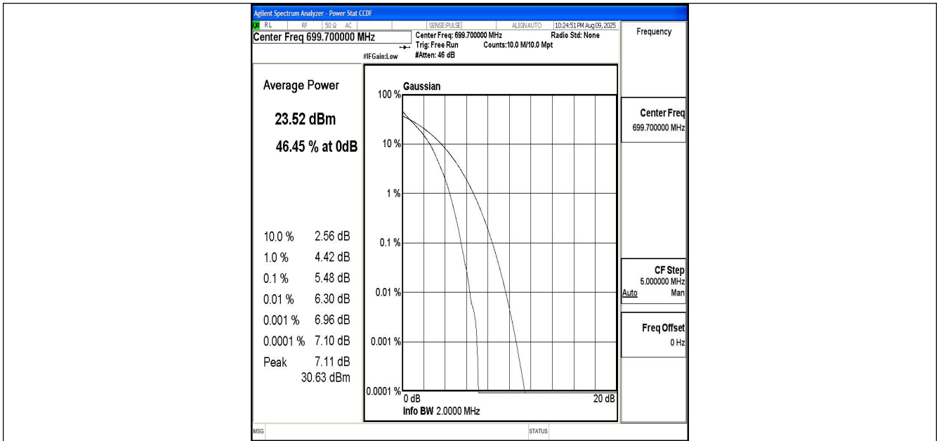
Band12-1.4MHz-QPSK-23017-6RB#0-PASS
