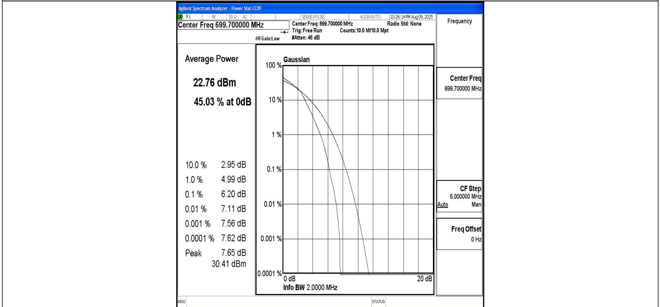
Band12-1.4MHz-16QAM-23017-6RB#0-PASS
