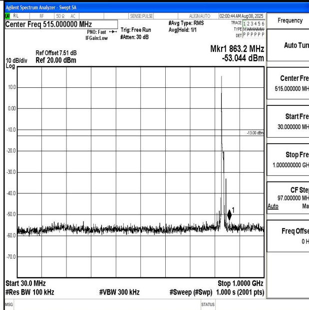
Band5_10MHz_QPSK_20525_1RB#0_30~1000_30~1000
