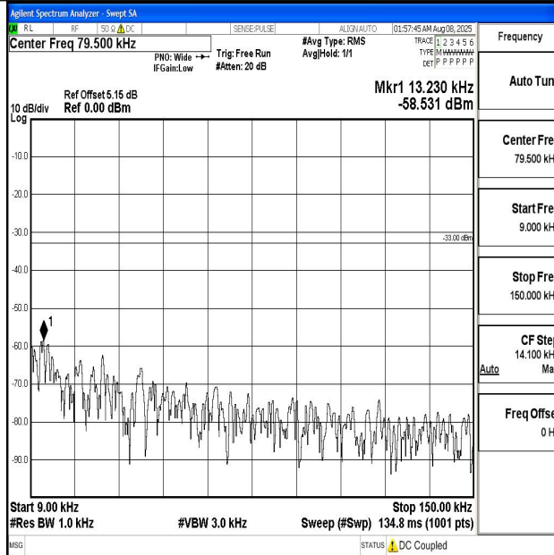
Band5_5MHz_QPSK_20625_1RB#0_0.009~0.15_0.009~0.15
