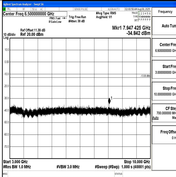
Band5_10MHz_QPSK_20525_1RB#0_3000~10000_3000~10000
