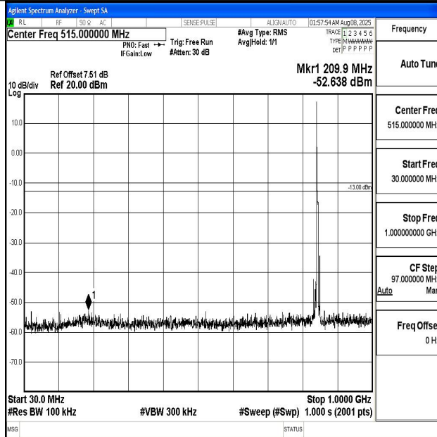
Band5_5MHz_QPSK_20625_1RB#0_30~1000_30~1000
