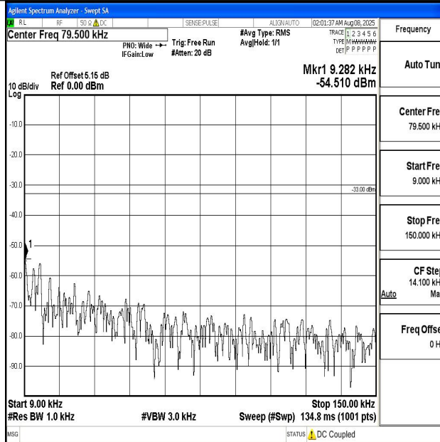
Band5_10MHz_QPSK_20600_1RB#0_0.009~0.15_0.009~0.15
