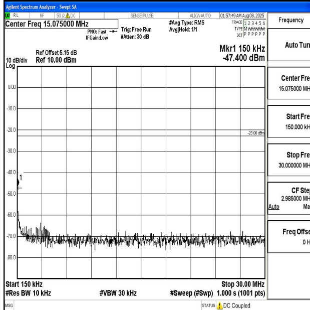
Band5_5MHz_QPSK_20625_1RB#0_0.15~30_0.15~30
