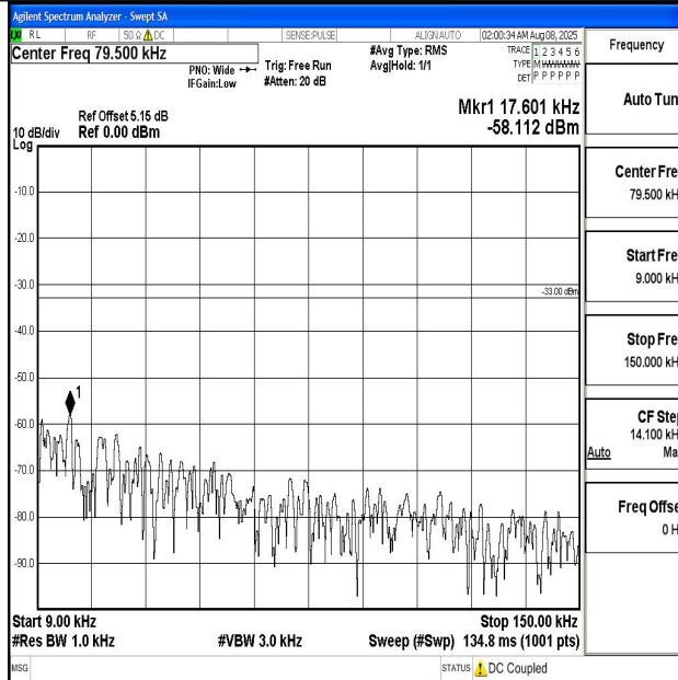
Band5_10MHz_QPSK_20525_1RB#0_0.009~0.15_0.009~0.15
