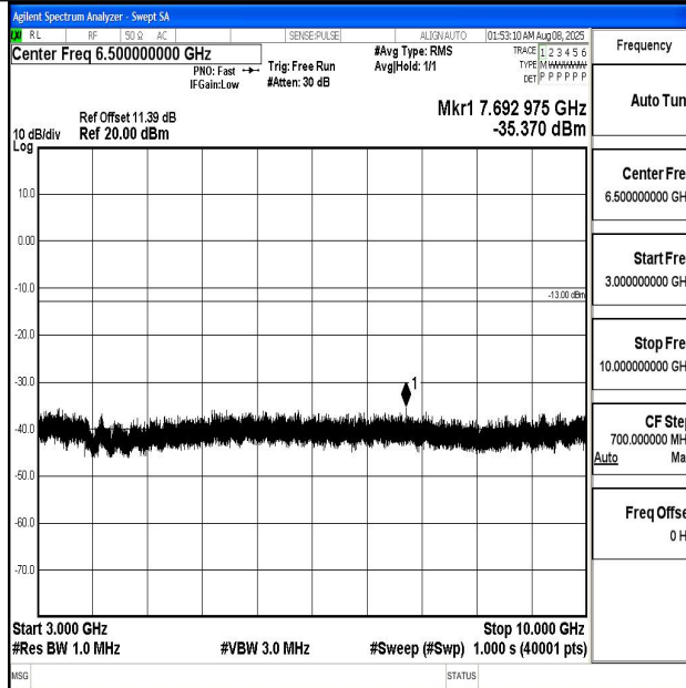
Band5_3MHz_QPSK_20525_1RB#0_3000~10000_3000~10000
