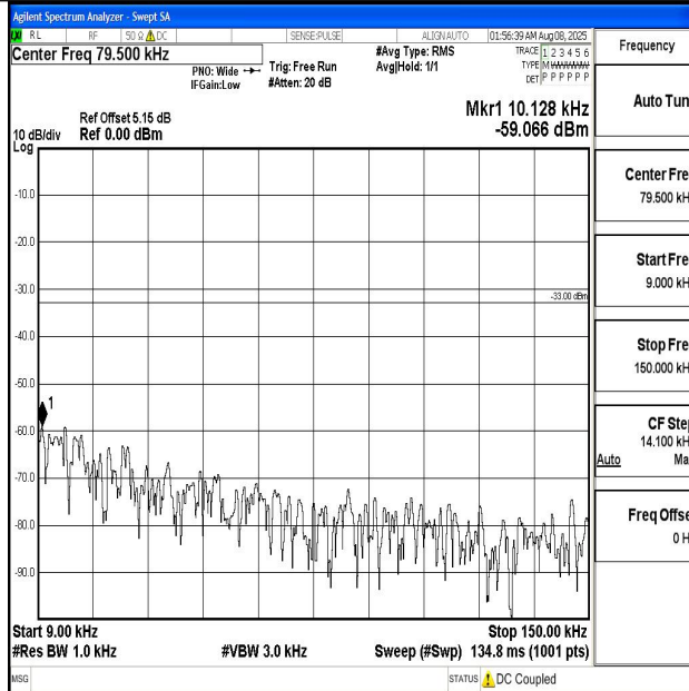
Band5_5MHz_QPSK_20525_1RB#0_0.009~0.15_0.009~0.15
