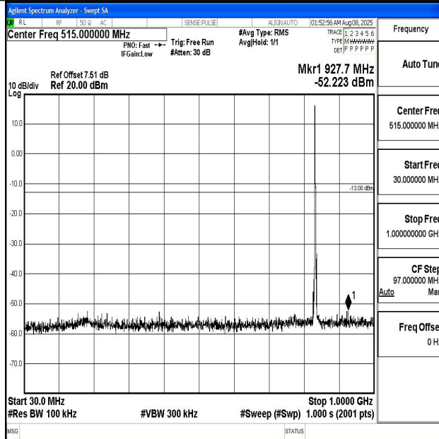
Band5_3MHz_QPSK_20525_1RB#0_30~1000_30~1000
