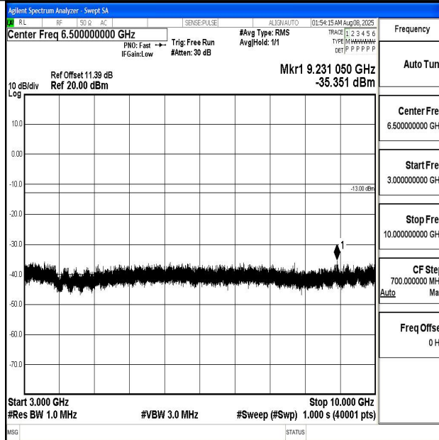
Band5_3MHz_QPSK_20635_1RB#0_3000~10000_3000~10000
