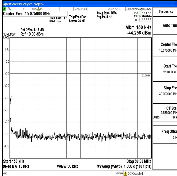
Band5_5MHz_QPSK_20425_1RB#0_0.15~30_0.15~30
