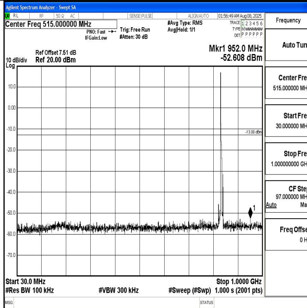
Band5_5MHz_QPSK_20525_1RB#0_30~1000_30~1000
