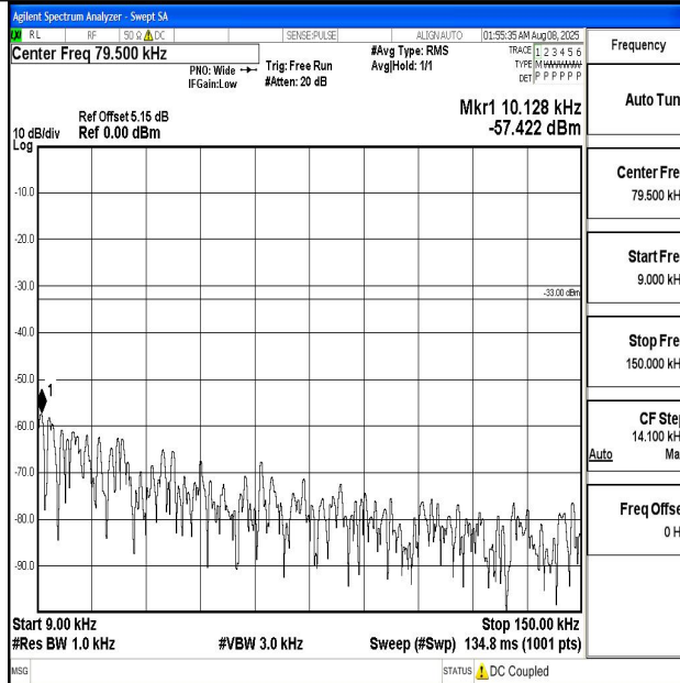
Band5_5MHz_QPSK_20425_1RB#0_0.009~0.15_0.009~0.15
