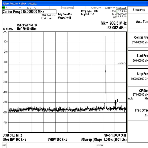
Band5_5MHz_QPSK_20425_1RB#0_30~1000_30~1000
