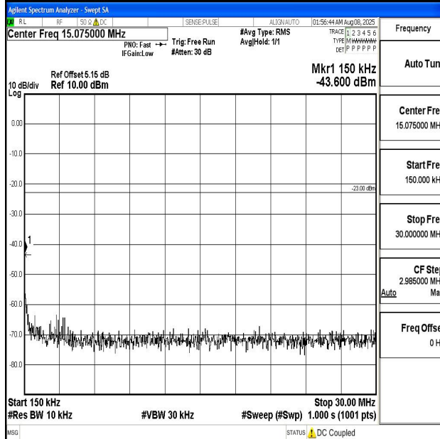
Band5_5MHz_QPSK_20525_1RB#0_0.15~30_0.15~30
