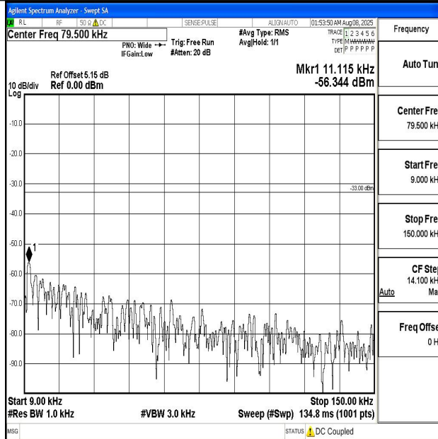
Band5_3MHz_QPSK_20635_1RB#0_0.009~0.15_0.009~0.15
