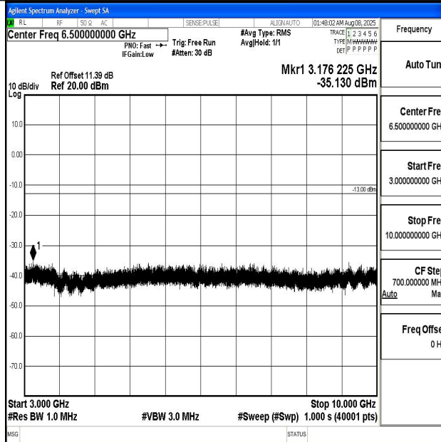
Band5_1.4MHz_QPSK_20407_1RB#0_3000~10000_3000~10000
