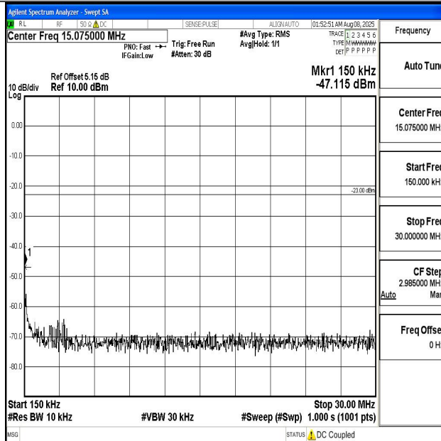
Band5_3MHz_QPSK_20525_1RB#0_0.15~30_0.15~30
