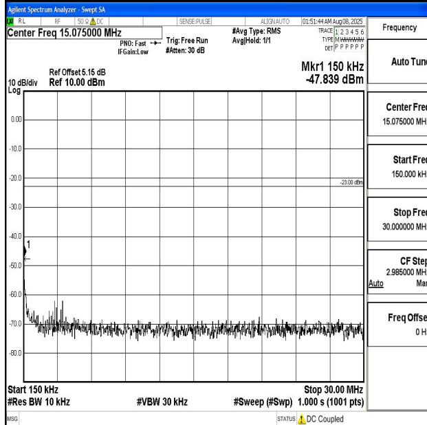
Band5_3MHz_QPSK_20415_1RB#0_0.15~30_0.15~30
