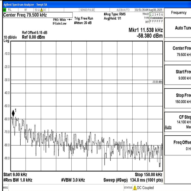
Band5_3MHz_QPSK_20415_1RB#0_0.009~0.15_0.009~0.15
