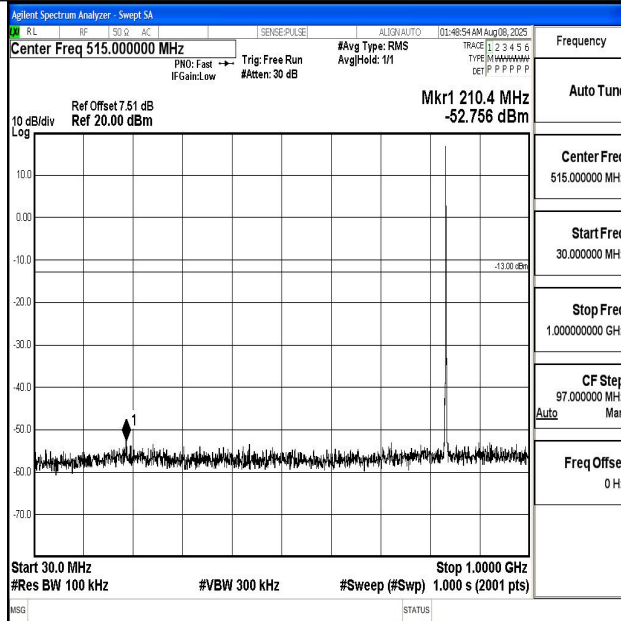
Band5_1.4MHz_QPSK_20525_1RB#0_30~1000_30~1000
