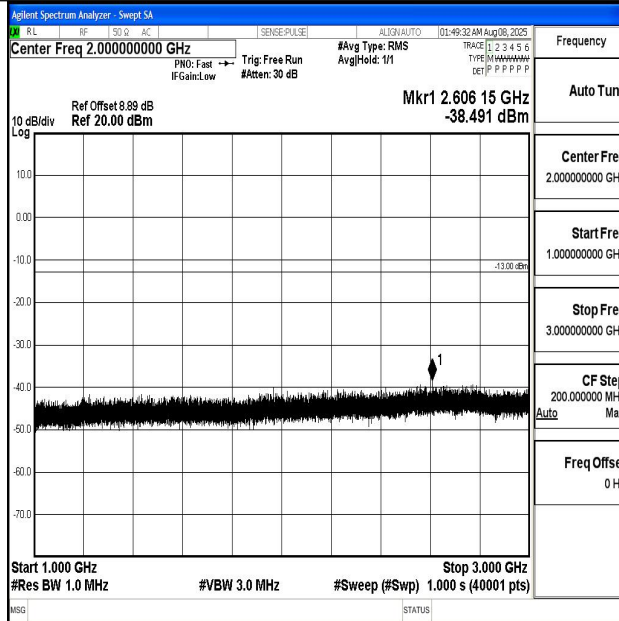
Band5_1.4MHz_16QAM_20525_1RB#0_1000~3000_1000~3000
