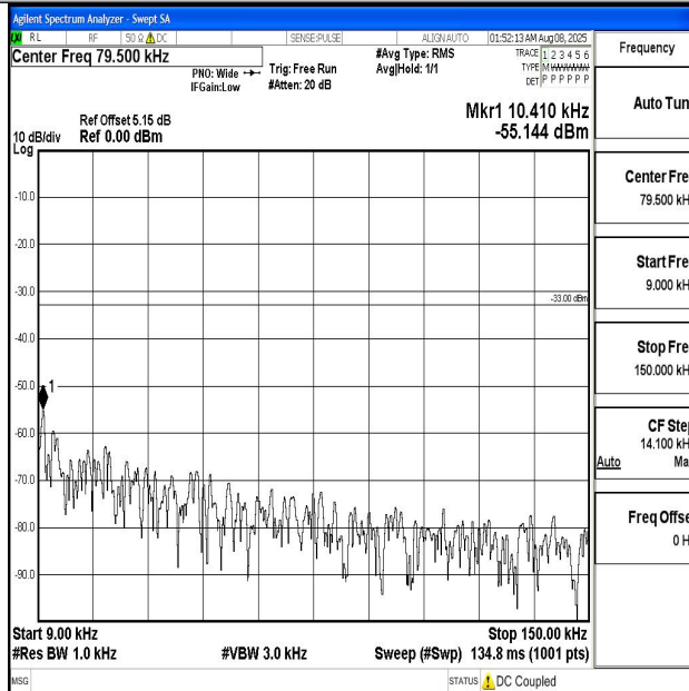
Band5_3MHz_16QAM_20415_1RB#0_0.009~0.15_0.009~0.15
