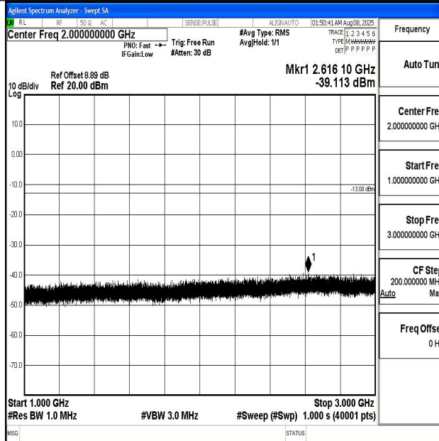
Band5_1.4MHz_16QAM_20643_1RB#0_1000~3000_1000~3000
