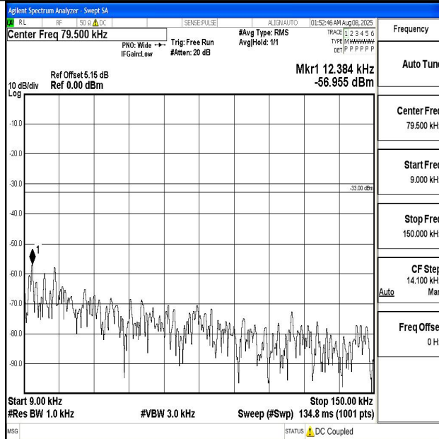
Band5_3MHz_QPSK_20525_1RB#0_0.009~0.15_0.009~0.15
