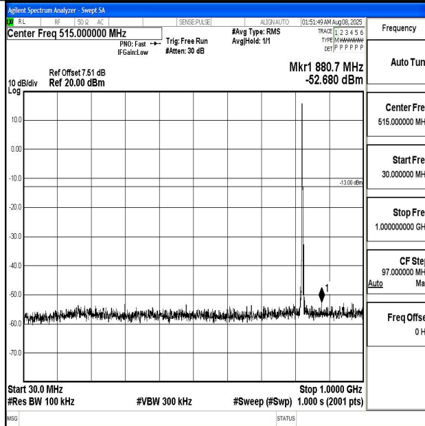
Band5_3MHz_QPSK_20415_1RB#0_30~1000_30~1000
