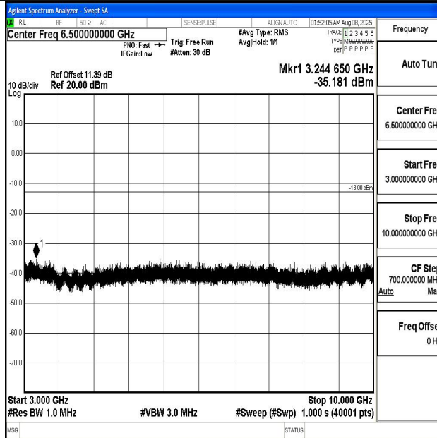
Band5_3MHz_QPSK_20415_1RB#0_3000~10000_3000~10000
