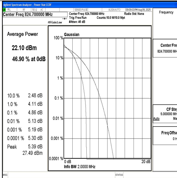
Band5-1.4MHz-QPSK-20407-1RB#0-PASS
