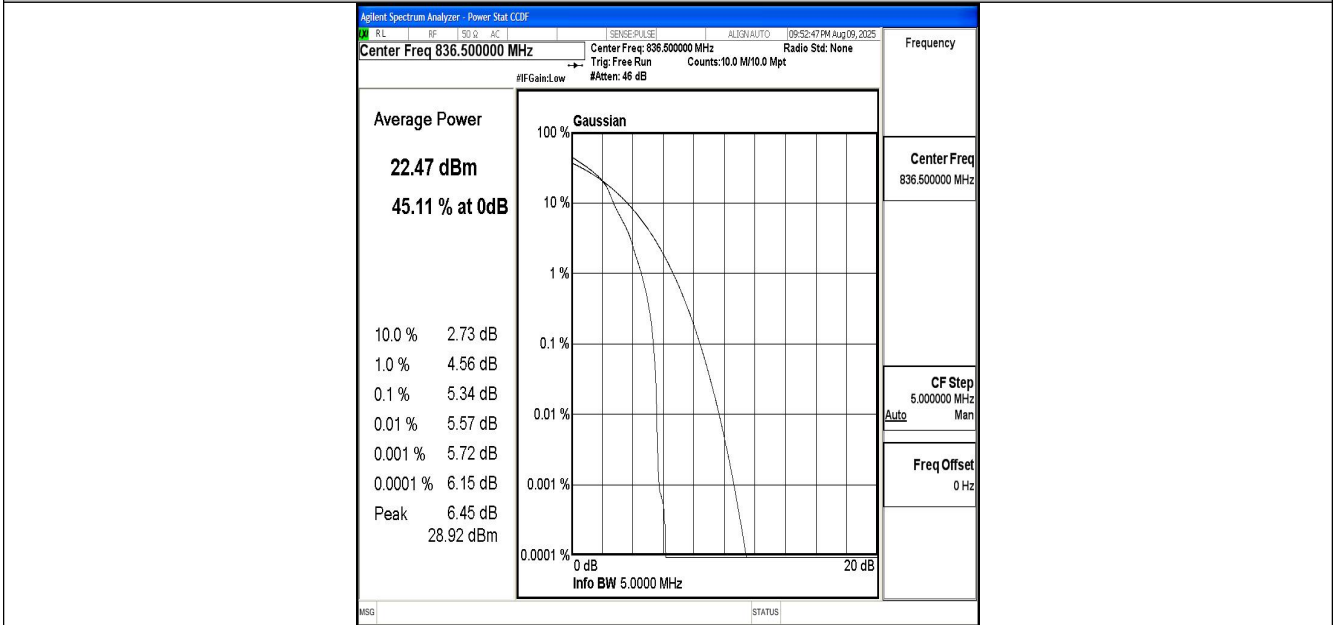
Band5-5MHz-16QAM-20525-1RB#0-PASS
