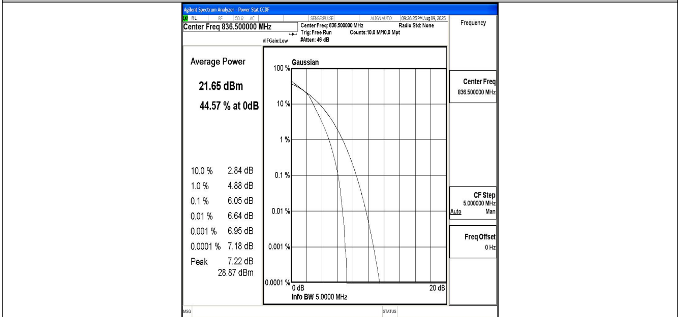
Band5-3MHz-16QAM-20525-15RB#0-PASS
