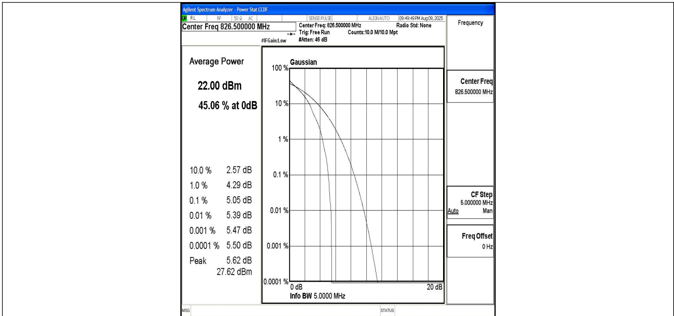
Band5-5MHz-QPSK-20425-1RB#0-PASS
