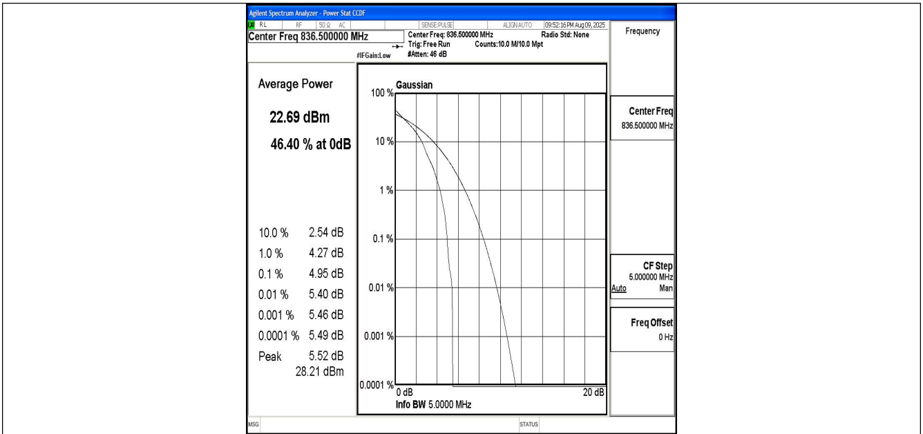
Band5-5MHz-QPSK-20525-1RB#0-PASS
