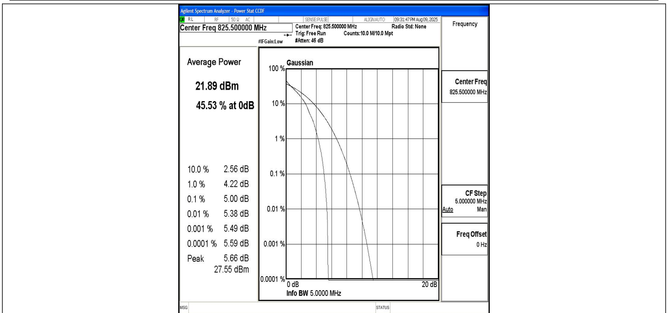
Band5-3MHz-QPSK-20415-1RB#0-PASS
