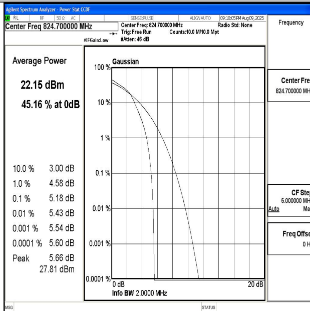
Band5-1.4MHz-16QAM-20407-1RB#0-PASS
