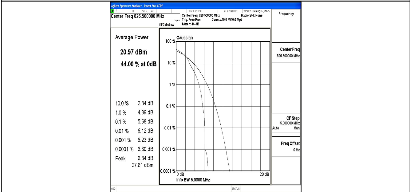
Band5-5MHz-16QAM-20425-1RB#0-PASS
