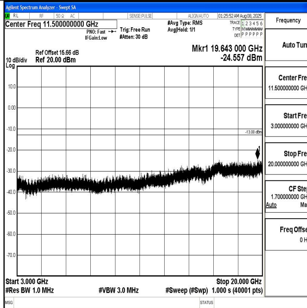
Band4_20MHz_QPSK_20175_1RB#0_3000~20000_3000~20000
