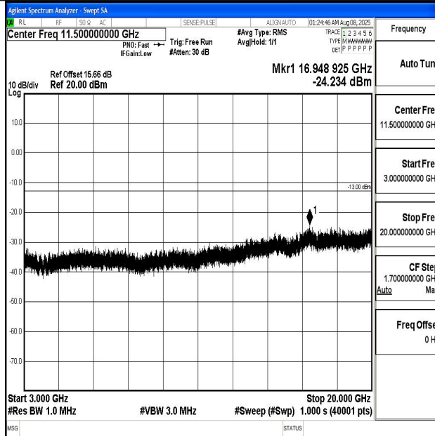
Band4_20MHz_QPSK_20050_1RB#0_3000~20000_3000~20000
