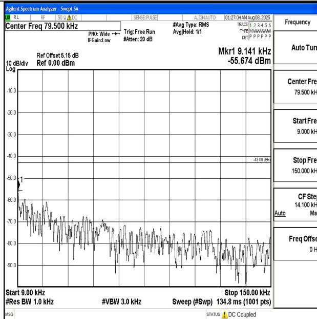
Band4_20MHz_16QAM_20300_1RB#0_0.009~0.15_0.009~0.15
