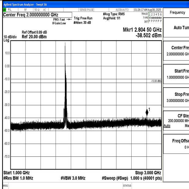
Band4_20MHz_16QAM_20175_1RB#0_1000~3000_1000~3000
