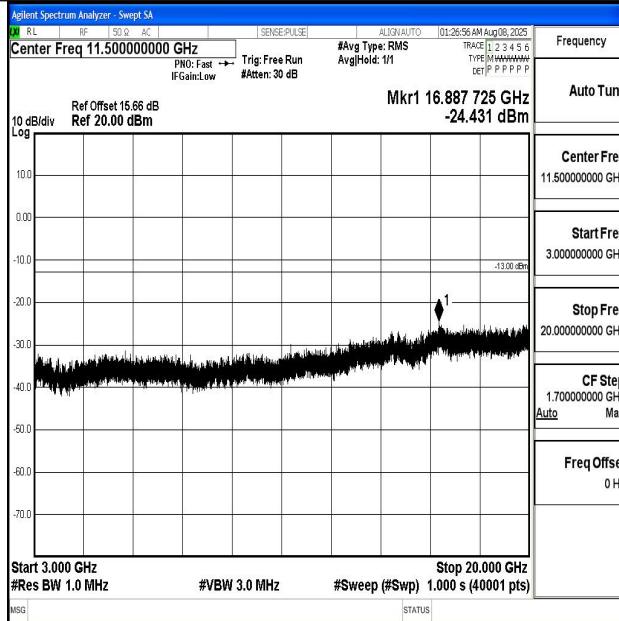
Band4_20MHz_QPSK_20300_1RB#0_3000~20000_3000~20000
