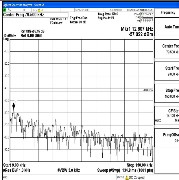
Band4_20MHz_16QAM_20175_1RB#0_0.009~0.15_0.009~0.15
