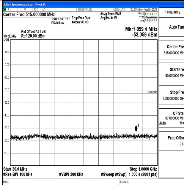
Band4_20MHz_QPSK_20175_1RB#0_30~1000_30~1000
