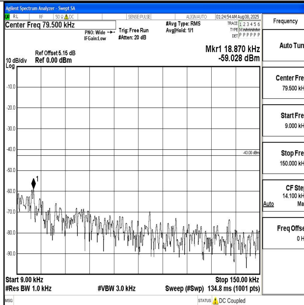
Band4_20MHz_16QAM_20050_1RB#0_0.009~0.15_0.009~0.15
