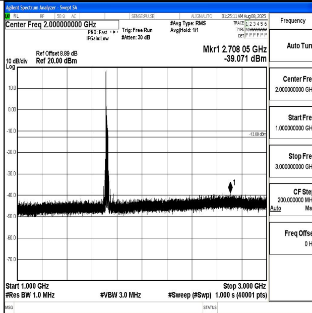
Band4_20MHz_16QAM_20050_1RB#0_1000~3000_1000~3000
