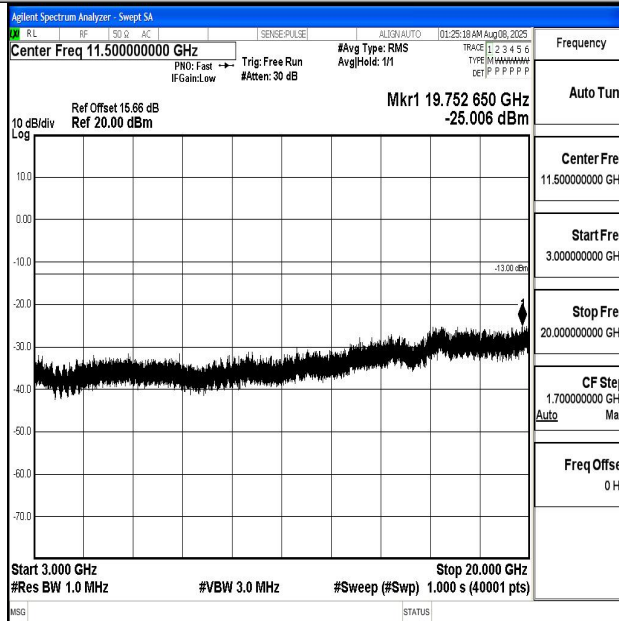
Band4_20MHz_16QAM_20050_1RB#0_3000~20000_3000~20000
