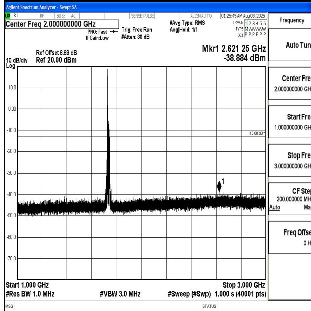
Band4_20MHz_QPSK_20175_1RB#0_1000~3000_1000~3000
