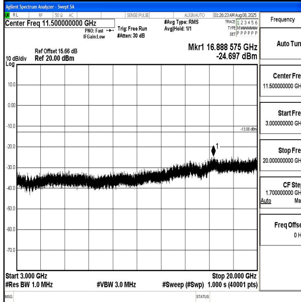
Band4_20MHz_16QAM_20175_1RB#0_3000~20000_3000~20000
