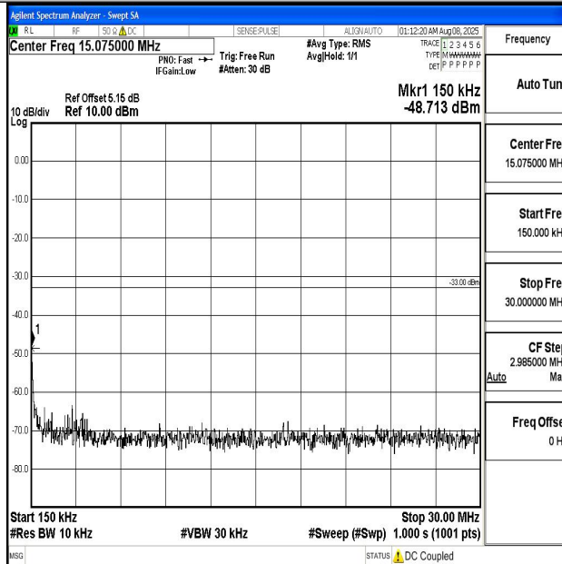
Band4_5MHz_QPSK_19975_1RB#0_0.15~30_0.15~30
