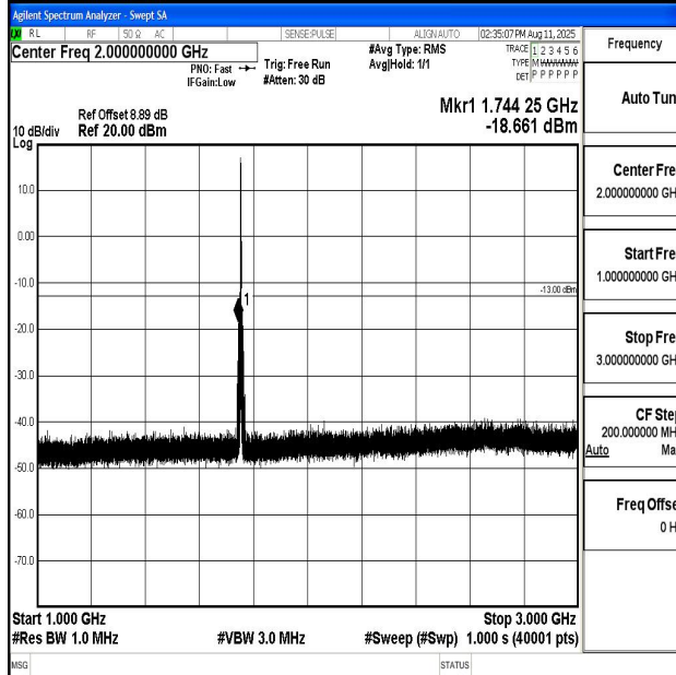
Band4_3MHz_QPSK_20385_1RB#0_1000~3000_1000~3000
