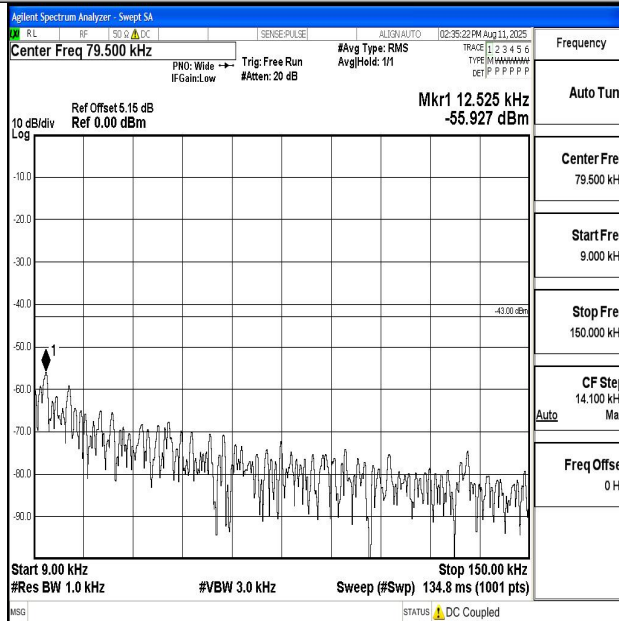
Band4_3MHz_16QAM_20385_1RB#0_0.009~0.15_0.009~0.15
