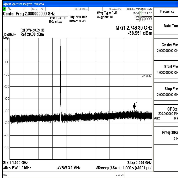
Band4_5MHz_QPSK_19975_1RB#0_1000~3000_1000~3000
