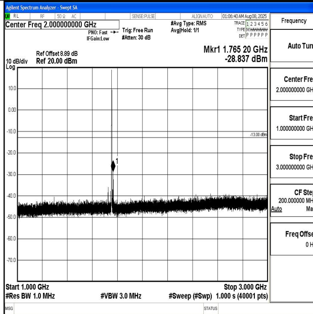
Band4_1.4MHz_QPSK_20393_1RB#0_1000~3000_1000~3000
