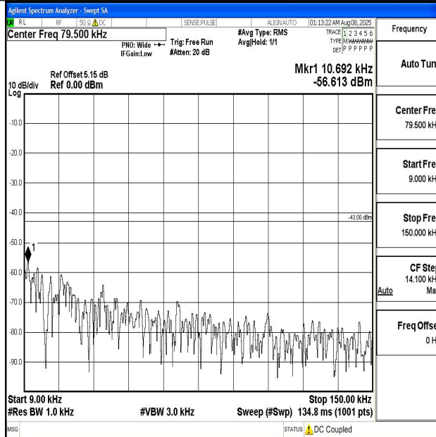
Band4_5MHz_QPSK_20175_1RB#0_0.009~0.15_0.009~0.15
