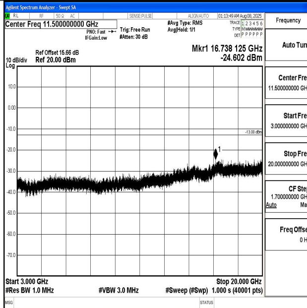
Band4_5MHz_QPSK_20175_1RB#0_3000~20000_3000~20000
