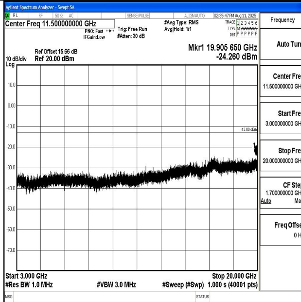
Band4_3MHz_16QAM_20385_1RB#0_3000~20000_3000~20000
