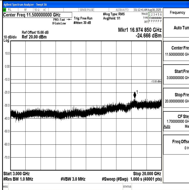
Band4_5MHz_QPSK_19975_1RB#0_3000~20000_3000~20000
