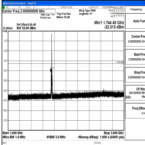
Band4_3MHz_16QAM_20385_1RB#0_1000~3000_1000~3000
