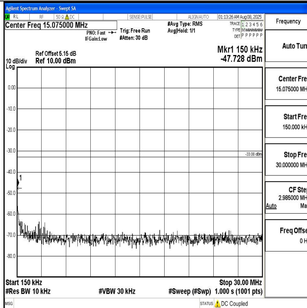
Band4_5MHz_QPSK_20175_1RB#0_0.15~30_0.15~30
