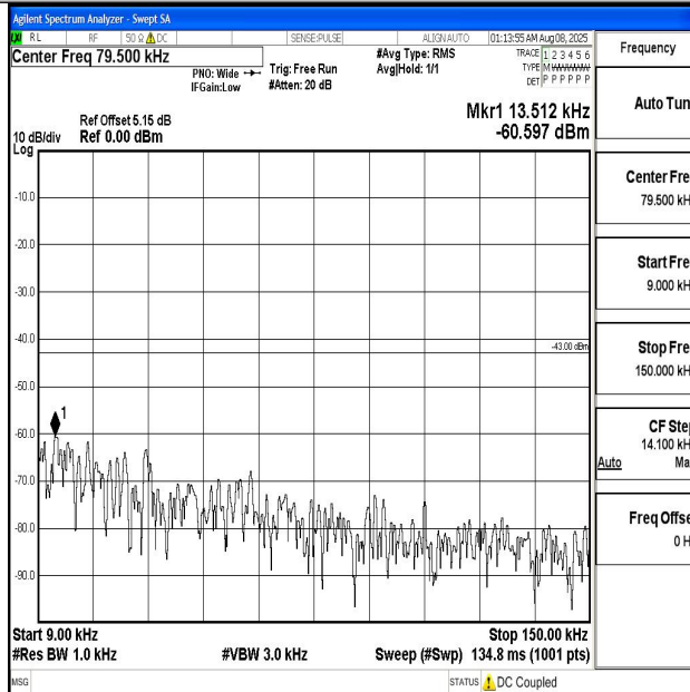
Band4_5MHz_16QAM_20175_1RB#0_0.009~0.15_0.009~0.15
