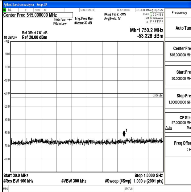
Band4_5MHz_QPSK_20175_1RB#0_30~1000_30~1000
