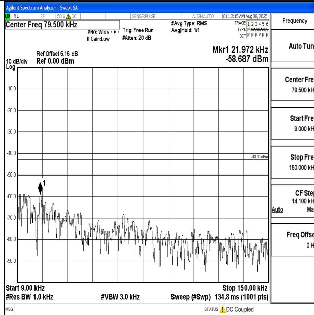
Band4_5MHz_QPSK_19975_1RB#0_0.009~0.15_0.009~0.15
