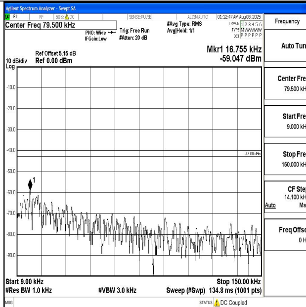
Band4_5MHz_16QAM_19975_1RB#0_0.009~0.15_0.009~0.15
