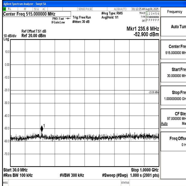
Band4_5MHz_QPSK_19975_1RB#0_30~1000_30~1000
