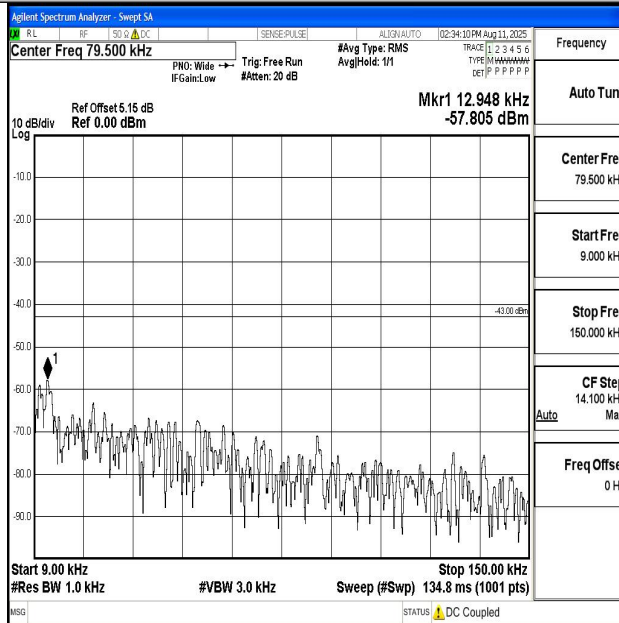
Band4_3MHz_16QAM_20175_1RB#0_0.009~0.15_0.009~0.15
