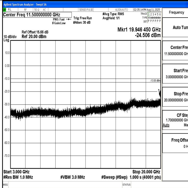
Band4_3MHz_QPSK_20385_1RB#0_3000~20000_3000~20000
