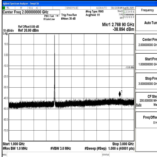
Band4_5MHz_QPSK_20175_1RB#0_1000~3000_1000~3000
