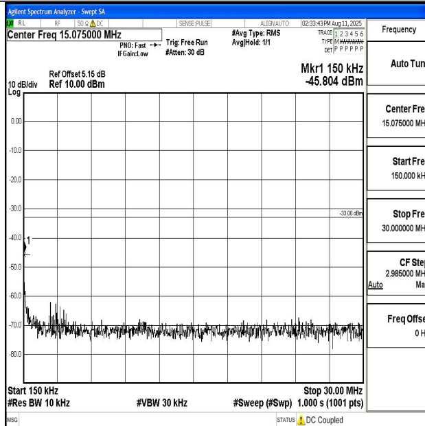
Band4_3MHz_QPSK_20175_1RB#0_0.15~30_0.15~30
