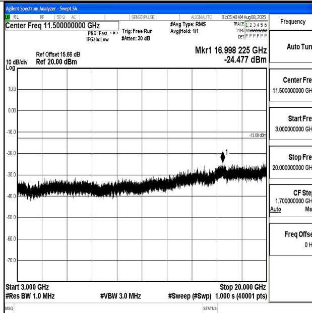
Band4_1.4MHz_QPSK_20175_1RB#0_3000~20000_3000~20000
