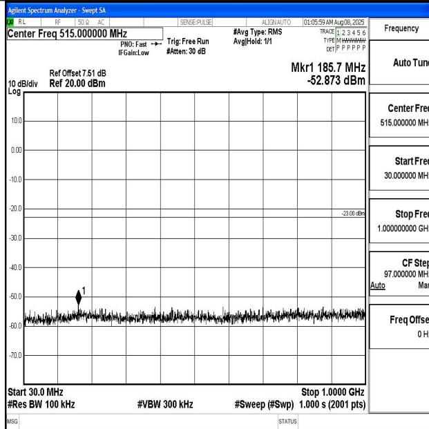
Band4_1.4MHz_16QAM_20175_1RB#0_30~1000_30~1000
