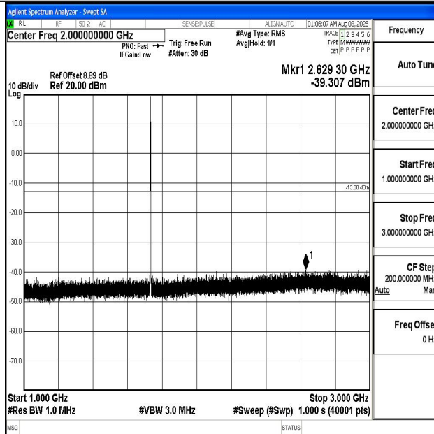
Band4_1.4MHz_16QAM_20175_1RB#0_1000~3000_1000~3000
