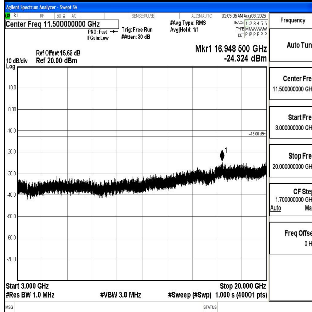
Band4_1.4MHz_16QAM_19957_1RB#0_3000~20000_3000~20000
