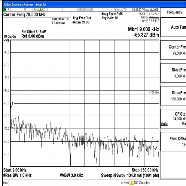
Band4_3MHz_QPSK_20175_1RB#0_0.009~0.15_0.009~0.15
