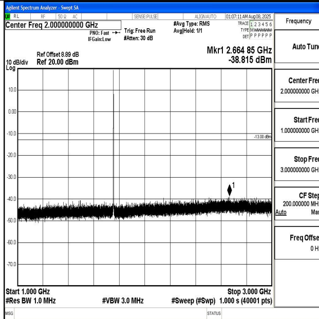
Band4_1.4MHz_16QAM_20393_1RB#0_1000~3000_1000~3000
