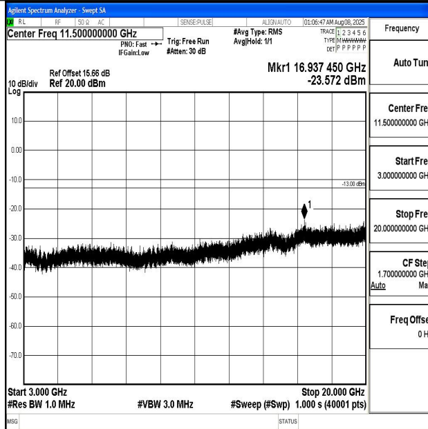
Band4_1.4MHz_QPSK_20393_1RB#0_3000~20000_3000~20000
