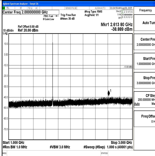
Band4_1.4MHz_16QAM_19957_1RB#0_1000~3000_1000~3000
