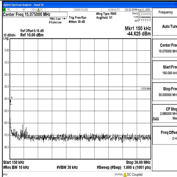
Band4_3MHz_QPSK_19965_1RB#0_0.15~30_0.15~30
