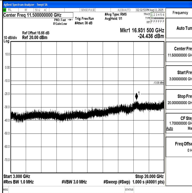
Band4_3MHz_QPSK_19965_1RB#0_3000~20000_3000~20000
