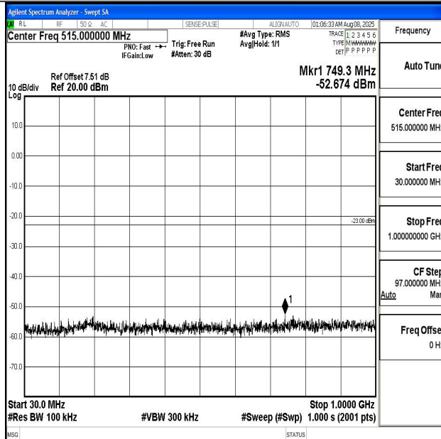
Band4_1.4MHz_QPSK_20393_1RB#0_30~1000_30~1000
