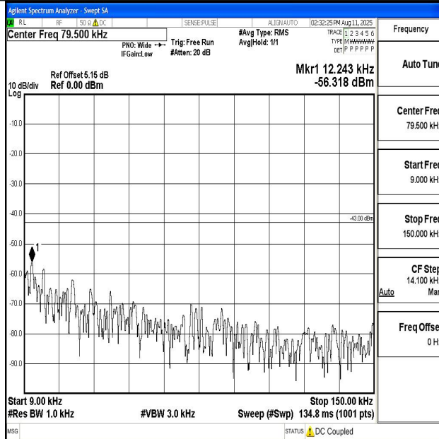
Band4_3MHz_QPSK_19965_1RB#0_0.009~0.15_0.009~0.15
