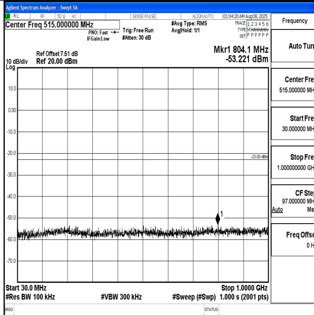
Band4_1.4MHz_QPSK_19957_1RB#0_30~1000_30~1000
