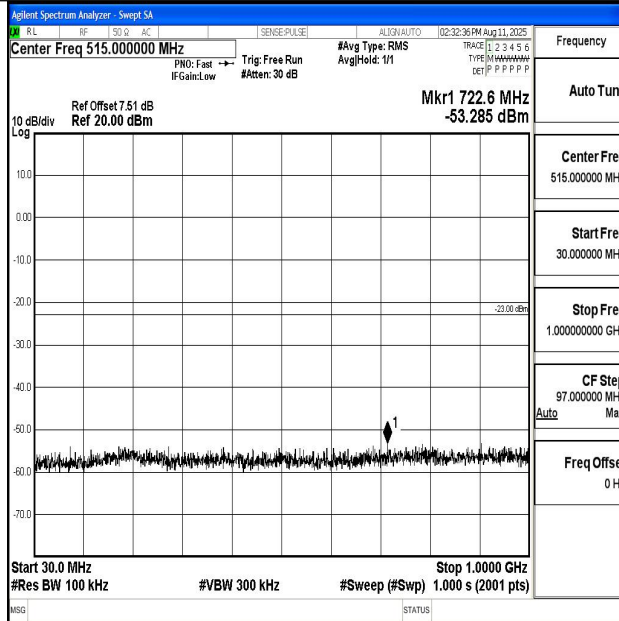
Band4_3MHz_QPSK_19965_1RB#0_30~1000_30~1000
