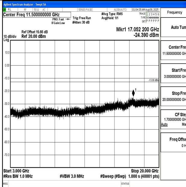
Band4_1.4MHz_QPSK_19957_1RB#0_3000~20000_3000~20000
