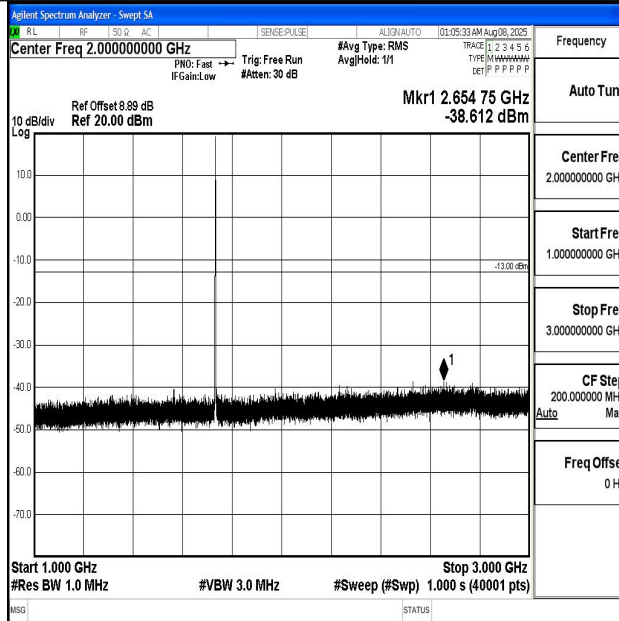
Band4_1.4MHz_QPSK_20175_1RB#0_1000~3000_1000~3000
