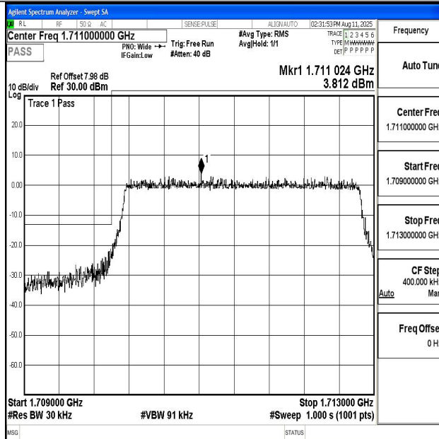
Band4_3MHz_16QAM_19965_15RB#0
