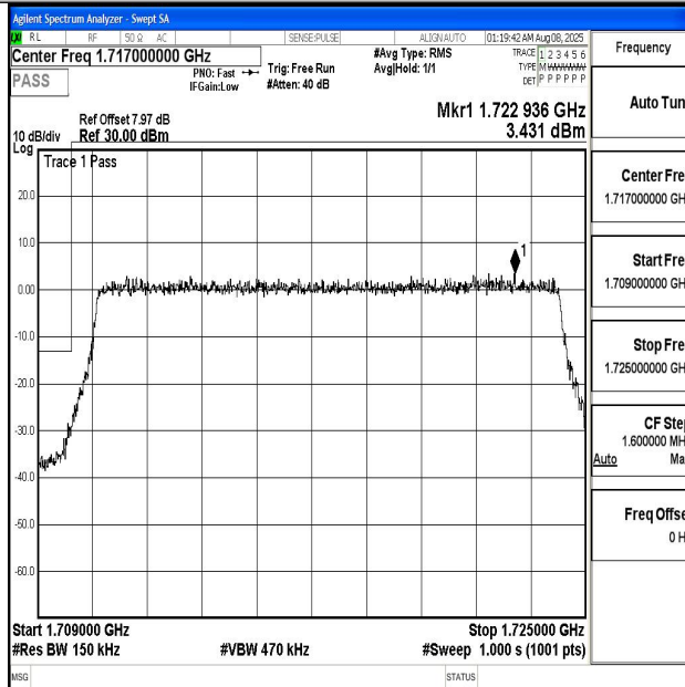
Band4_15MHz_16QAM_20025_75RB#0
