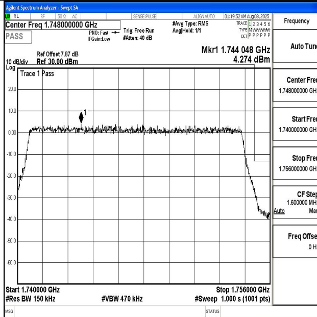
Band4_15MHz_QPSK_20325_75RB#0
