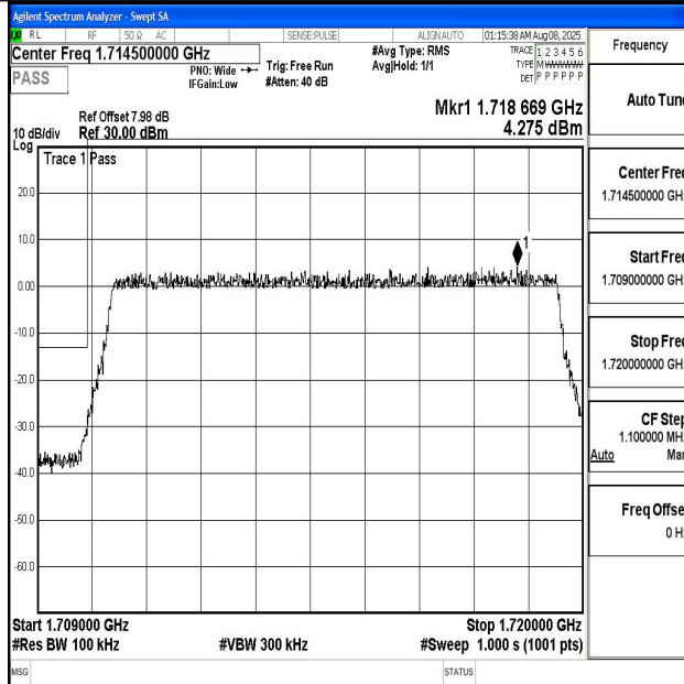
Band4_10MHz_QPSK_20000_50RB#0
