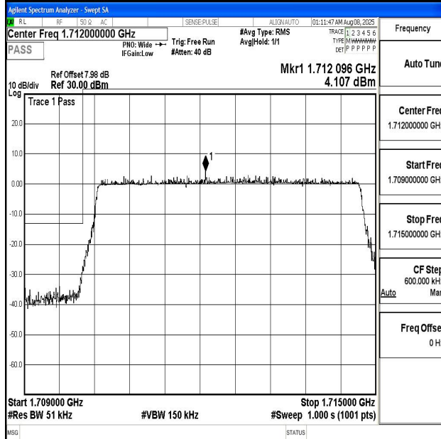
Band4_5MHz_16QAM_19975_25RB#0
