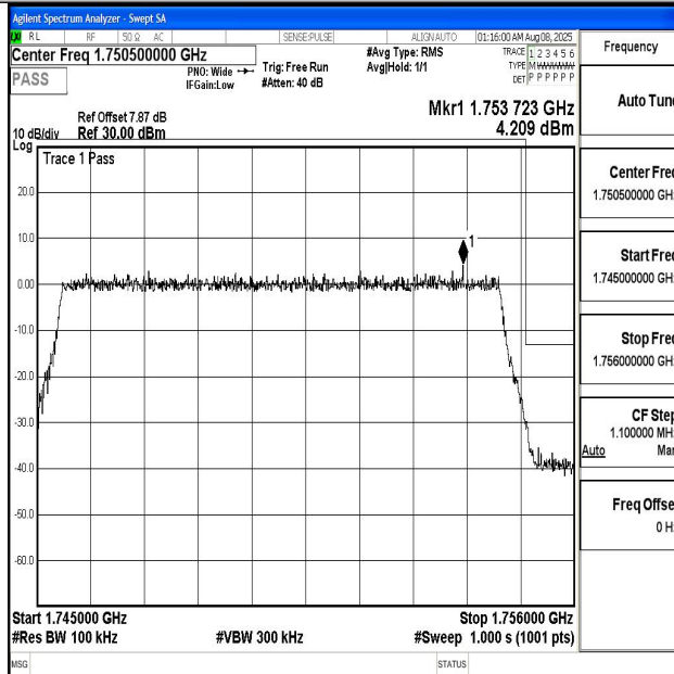
Band4_10MHz_16QAM_20350_50RB#0
