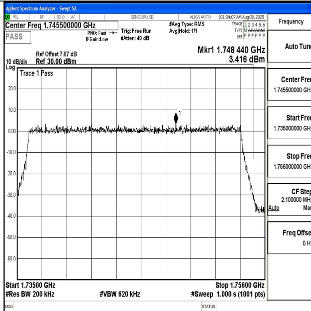
Band4_20MHz_16QAM_20300_100RB#0
