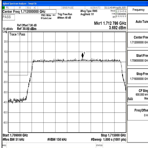
Band4_5MHz_QPSK_19975_25RB#0
