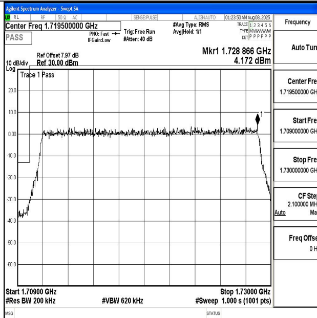
Band4_20MHz_16QAM_20050_100RB#0
