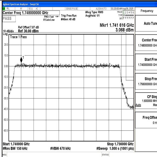
Band4_15MHz_16QAM_20325_75RB#0
