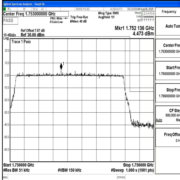
Band4_5MHz_16QAM_20375_25RB#0
