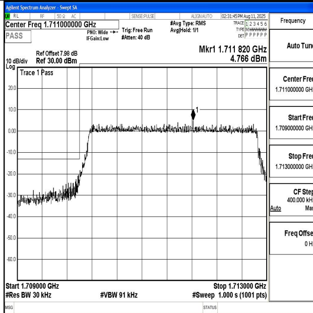
Band4_3MHz_QPSK_19965_15RB#0
