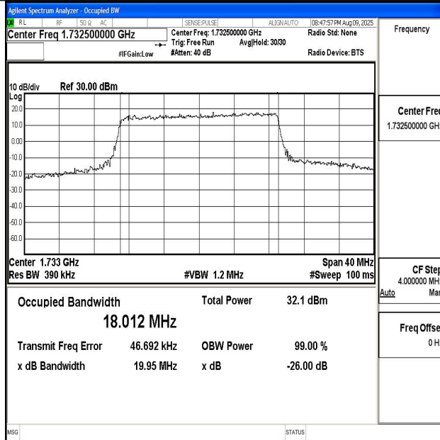
Band4-20MHz-QPSK-20175-100RB#0-PASS
