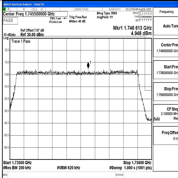
Band4_20MHz_QPSK_20300_100RB#0
