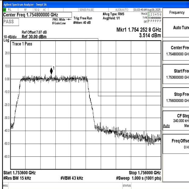
Band4_1.4MHz_QPSK_20393_6RB#0
