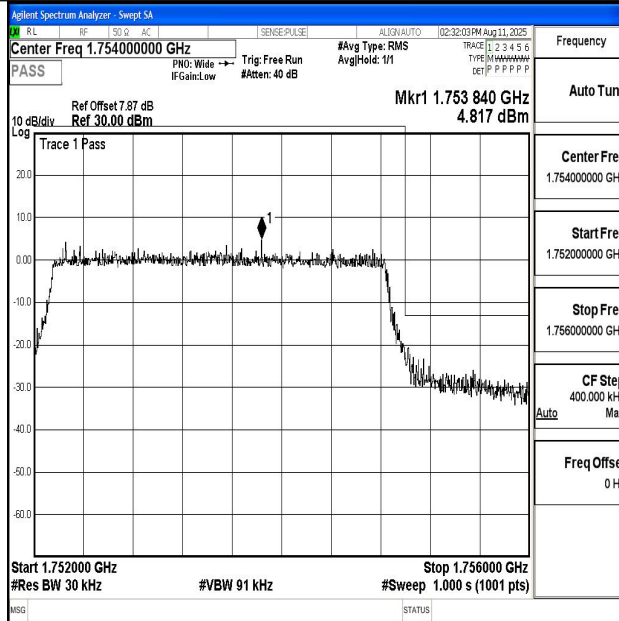
Band4_3MHz_QPSK_20385_15RB#0
