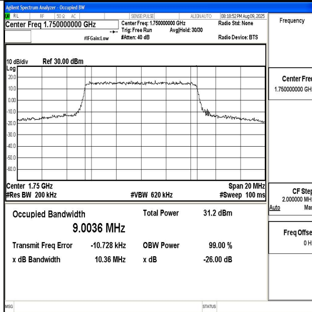
Band4-10MHz-QPSK-20350-50RB#0-PASS
