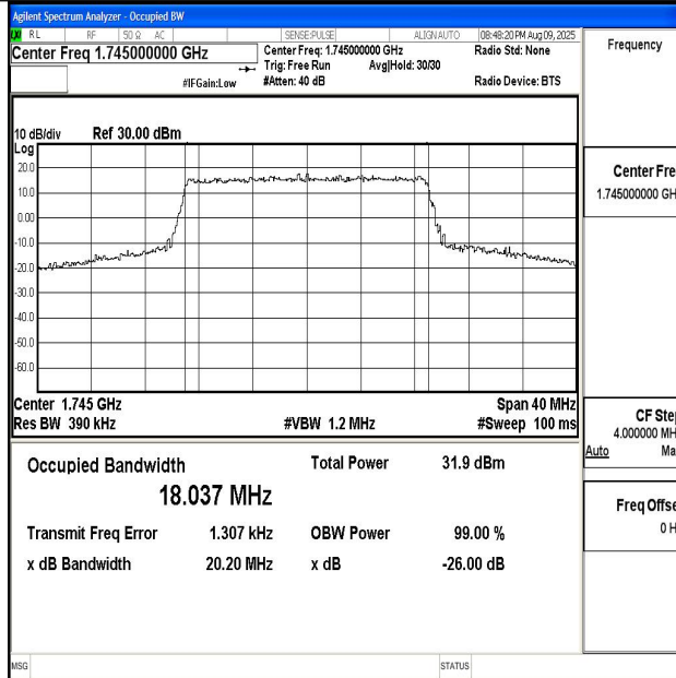
Band4-20MHz-QPSK-20300-100RB#0-PASS
