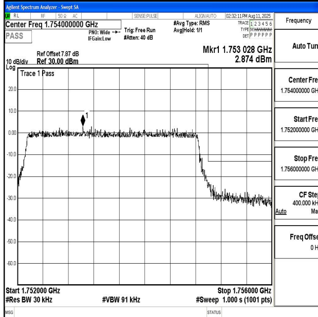
Band4_3MHz_16QAM_20385_15RB#0
