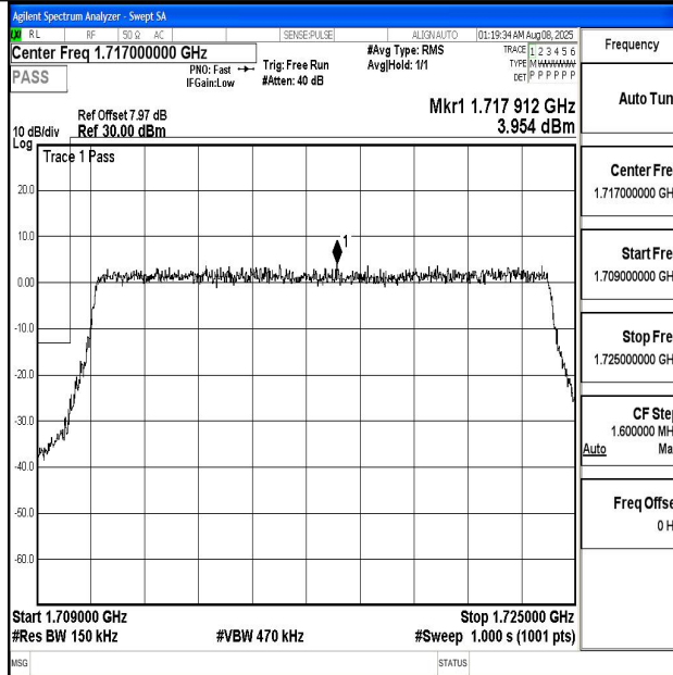
Band4_15MHz_QPSK_20025_75RB#0
