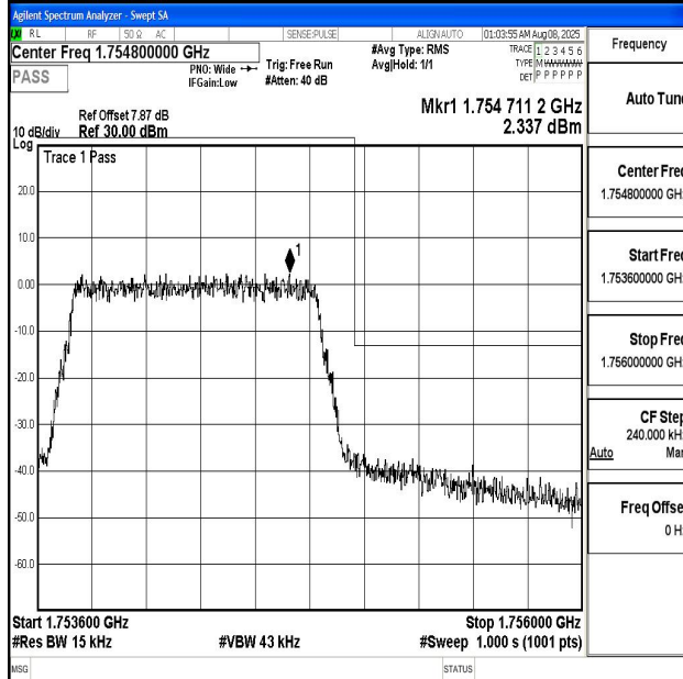
Band4_1.4MHz_16QAM_20393_6RB#0
