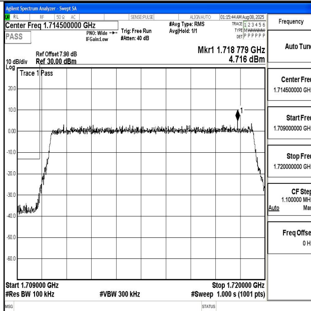
Band4_10MHz_16QAM_20000_50RB#0
