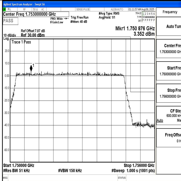
Band4_5MHz_QPSK_20375_25RB#0
