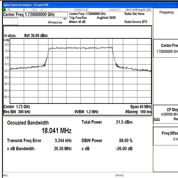
Band4-20MHz-16QAM-20050-100RB#0-PASS
