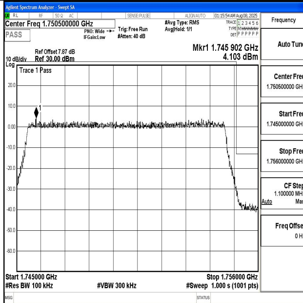
Band4_10MHz_QPSK_20350_50RB#0
